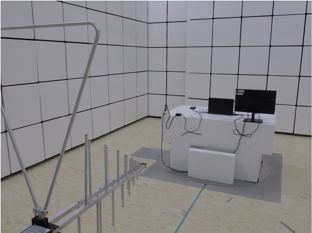
Radiated Test
