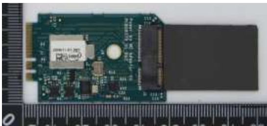
Socket front
