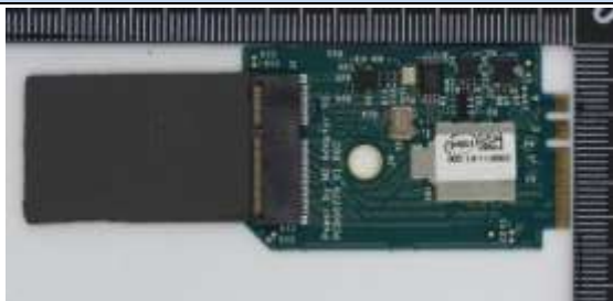
Socket front
