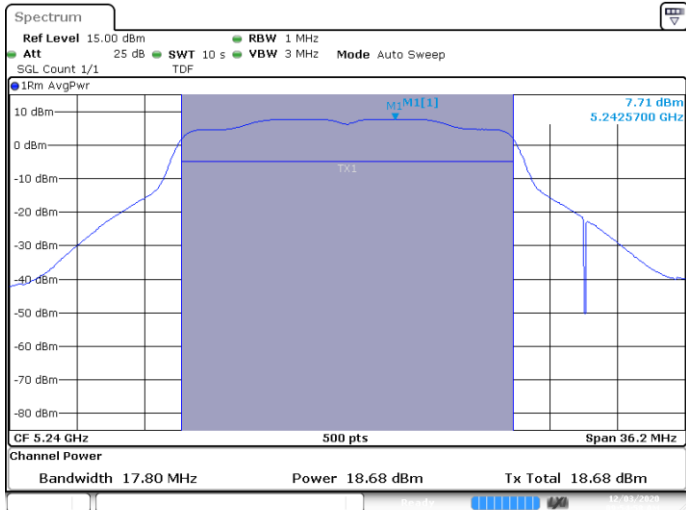
SISO A-802.11a-20MHz-Ch48-5240MHz-6
