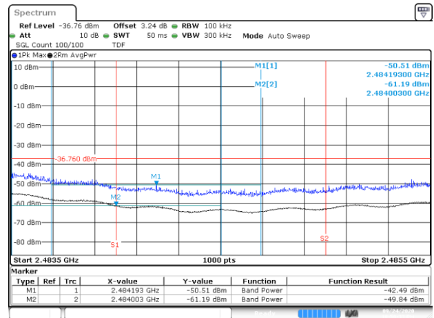
BE-R-HIGH-2MHz, MIMO-A, 802.11n40-HT0, Ch13
