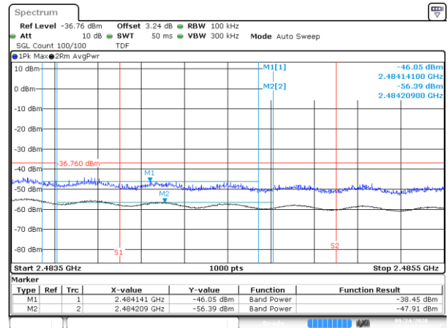
BE-R-HIGH-2MHz, MIMO-A, 802.11n40- HT8, Ch12
