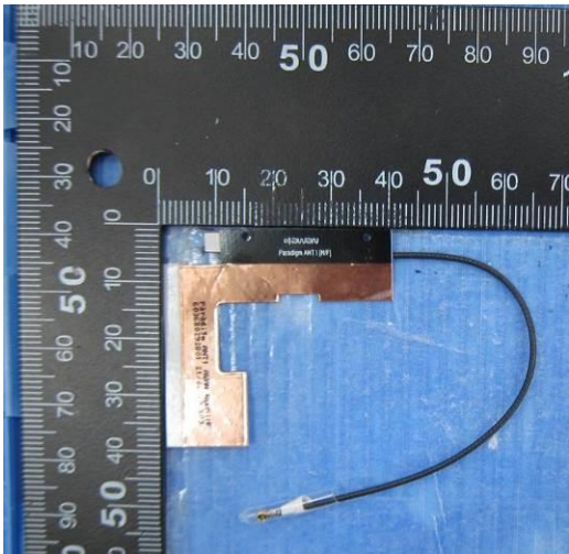
Tx1 Antenna Photo:
