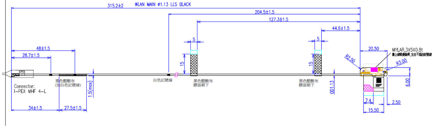
Tx1 Antenna Dimensioned Drawing:
