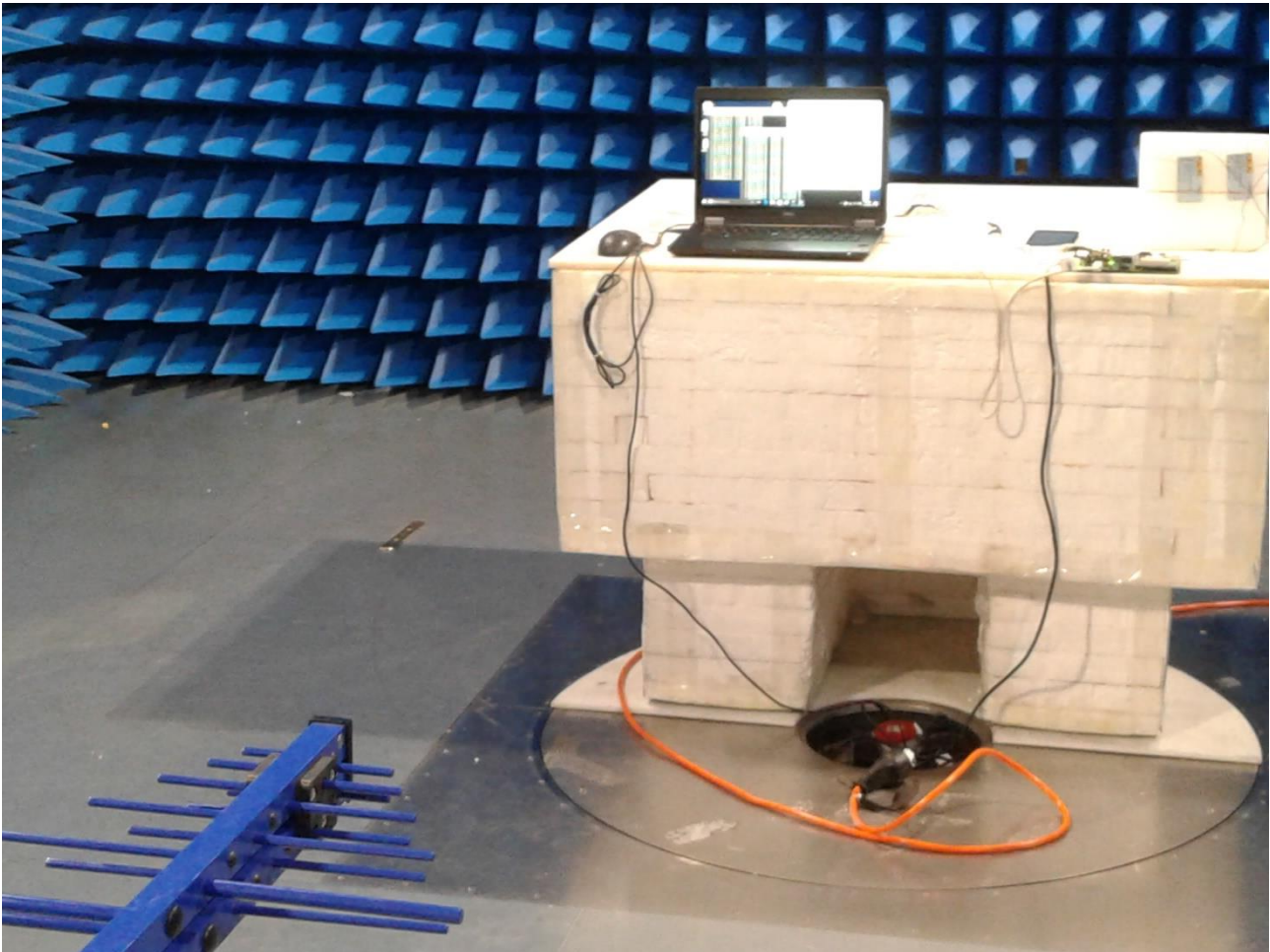
Photo 1 Photograph test setup radiated emissions 30-1000 MHz
