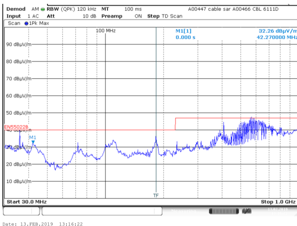
Plot 2: Pre-scan plot with peak detector. Radiated emissions from 30 MHz to 1000 MHz, 5GHz and BT mode.
