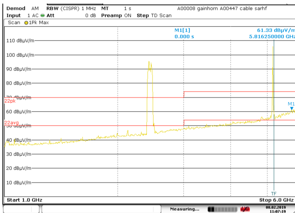
Plot 4: Pre-scan plot with peak detector. Radiated emissions from 1 GHz – 6 GHz, 5 GHz and BT mode
