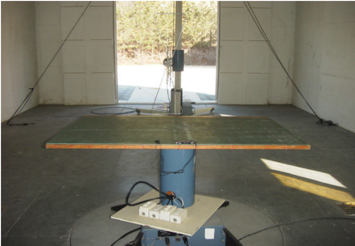
Play : Radiated Emission 30MHz ~ 1000MHz
