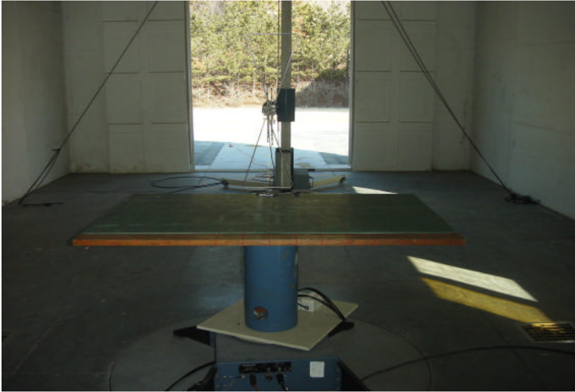
Play : Radiated Emission 30MHz ~ 1000MHz
