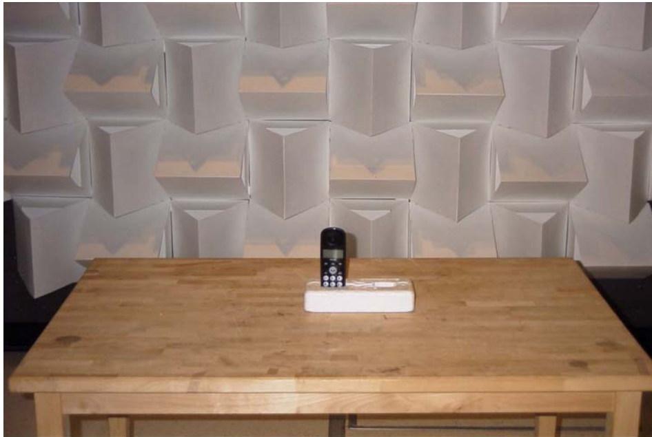
Radiated Test Set Up (Handset)
