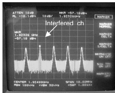
No TX on interfered channel
