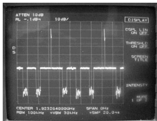
Interference injected on used time slots
