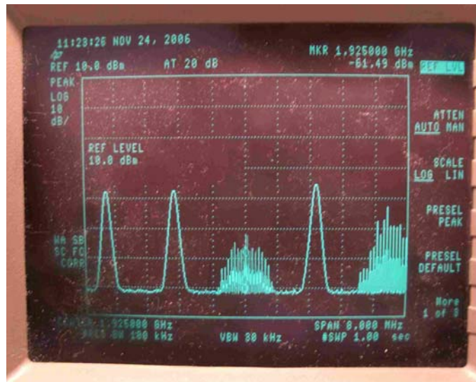
Link-up between base and handset on free channel
