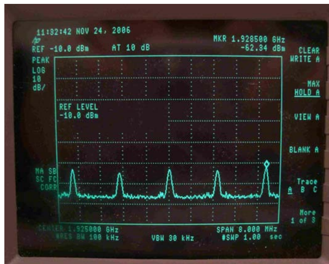
No TX when interference applied to whole frame period
