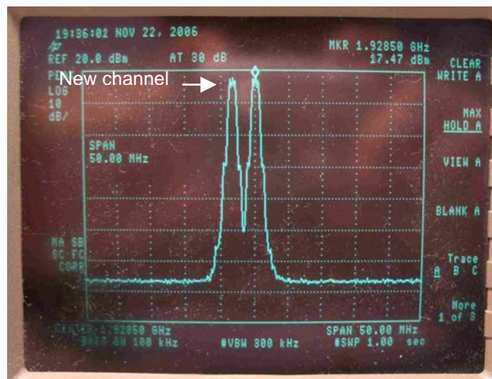
TX in transition to different channel in 3 hr 13 min.
