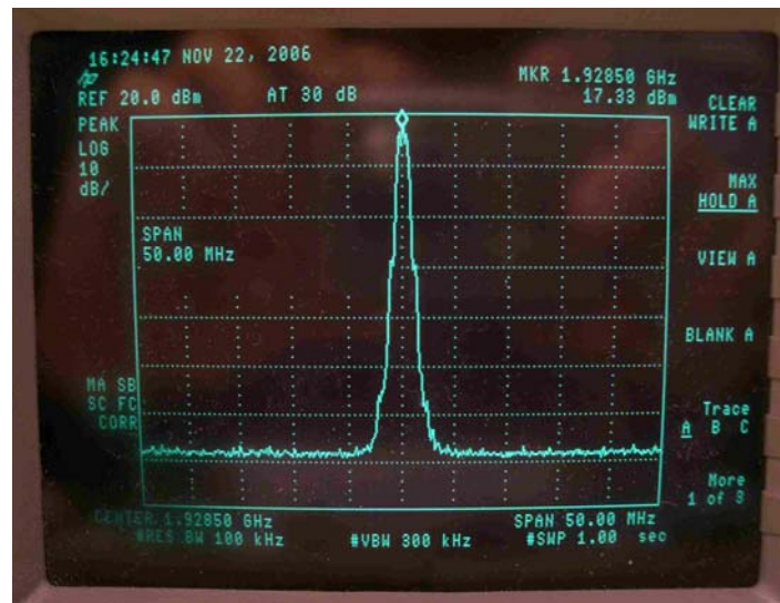
TX starting on high-frequency channel
