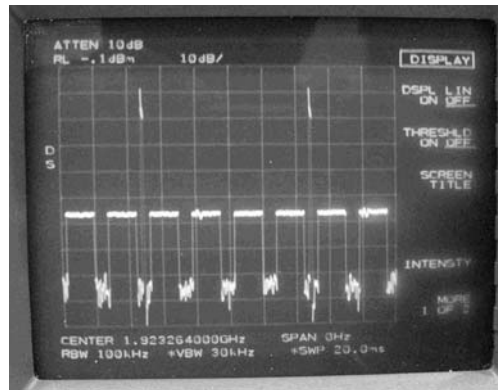
TX on free time slots of a channel
