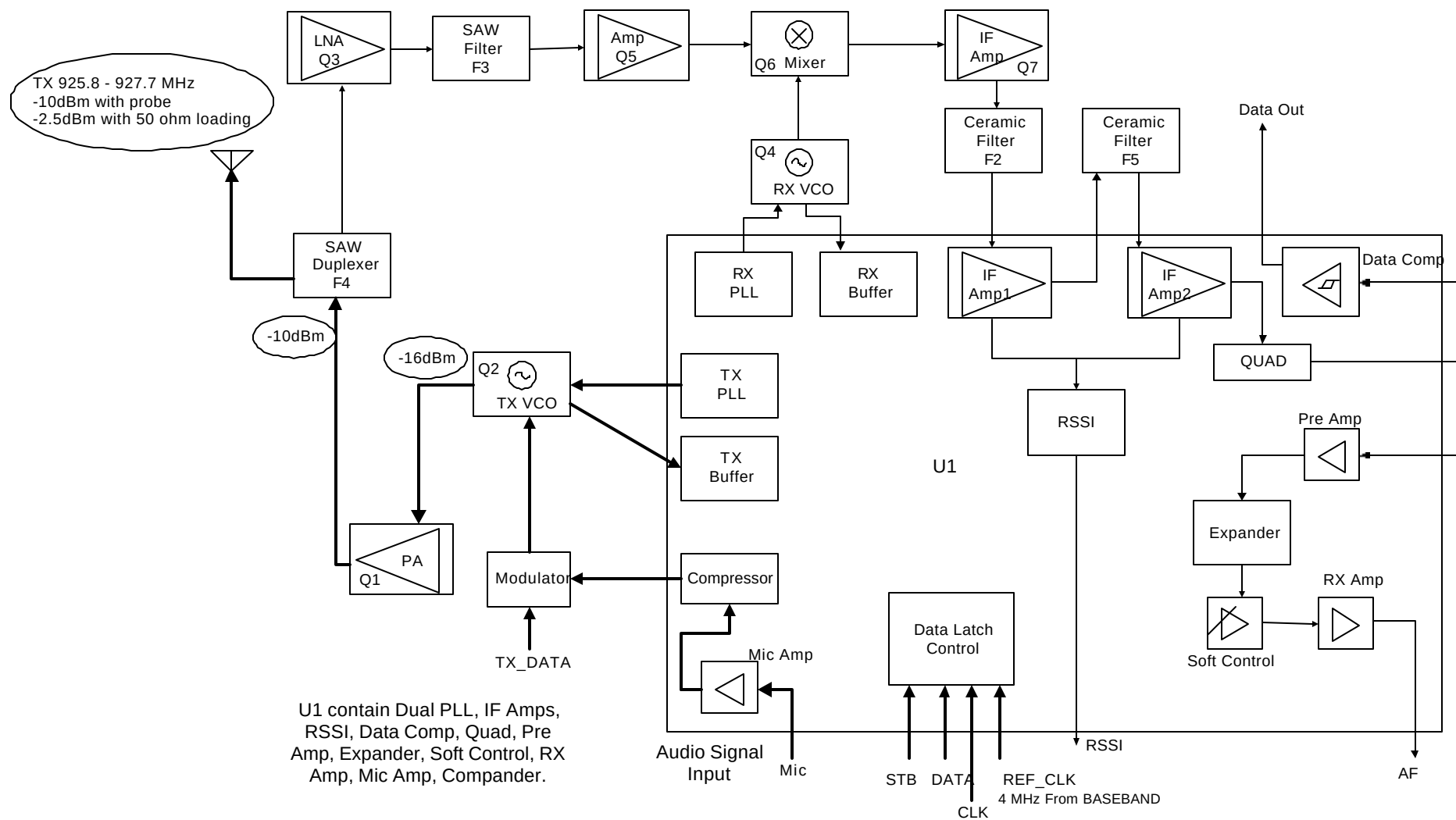
RF Signal Transmit Paths
