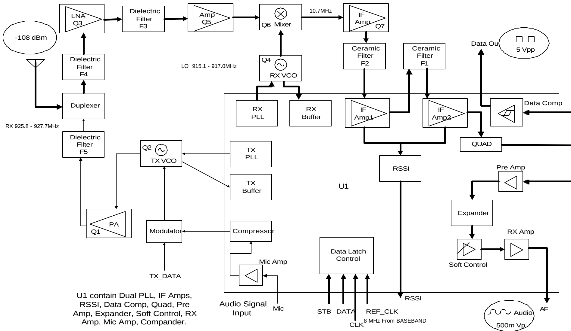
RF Signal Receive Paths
