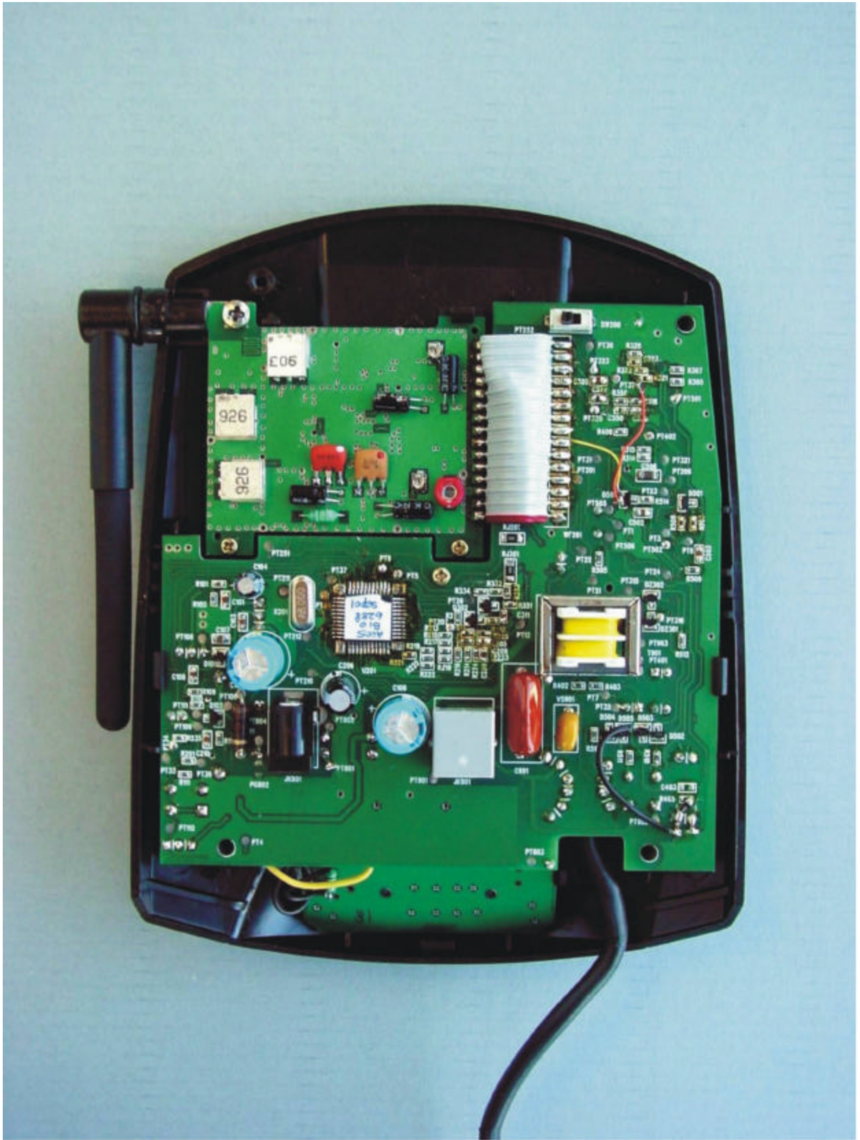
Base PCBA Bottom View
