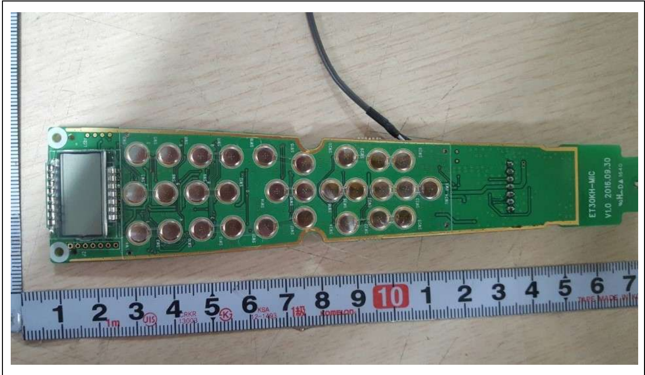
MIC Board – Front
