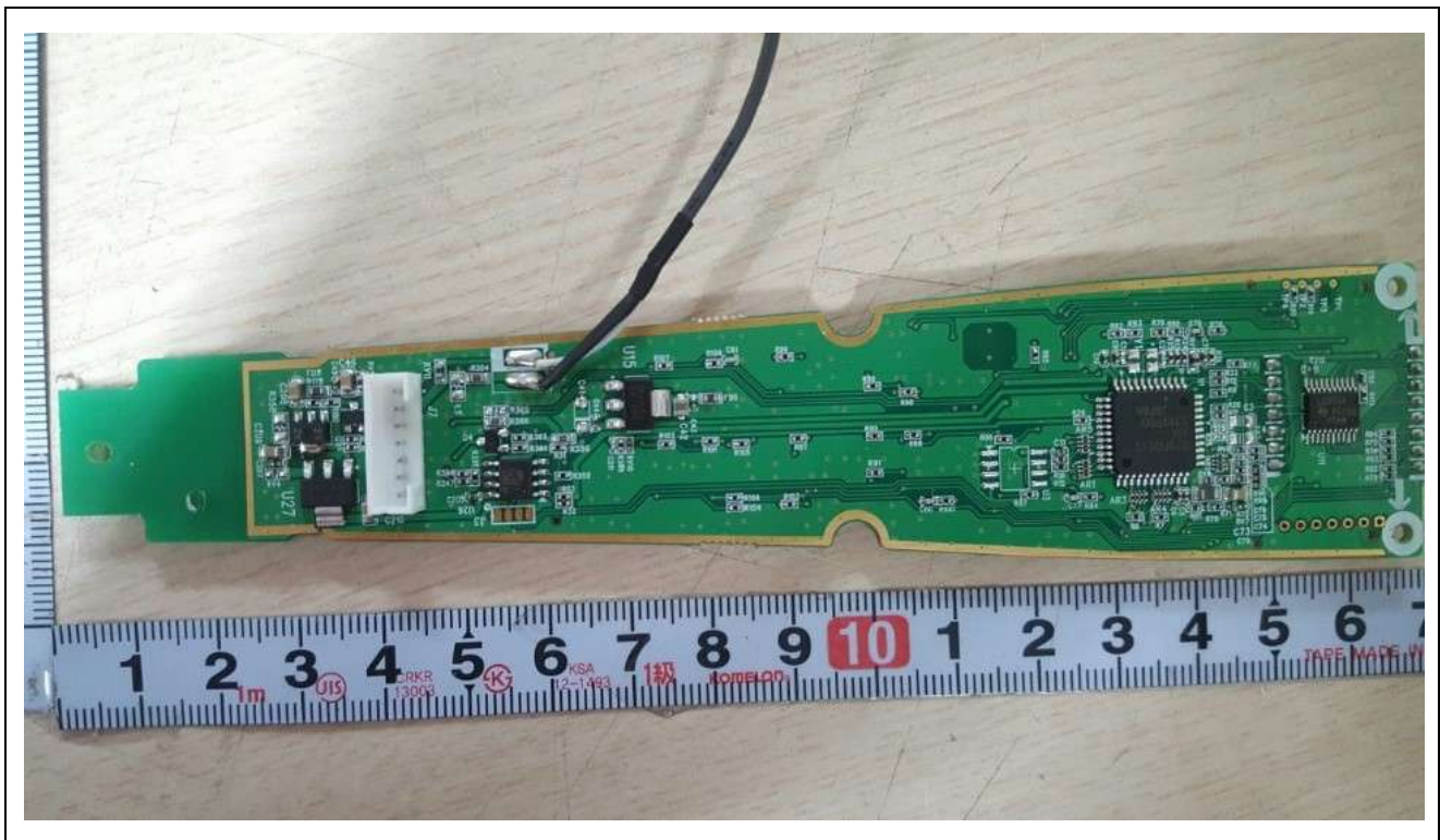
MIC Board – Rear
