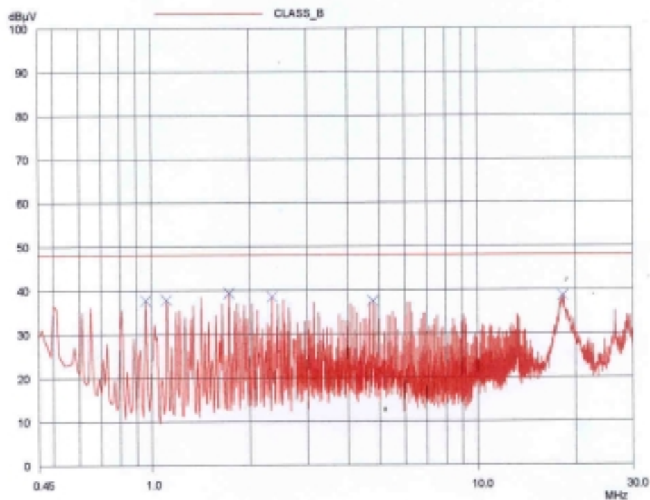
NEUTRAL LINE
