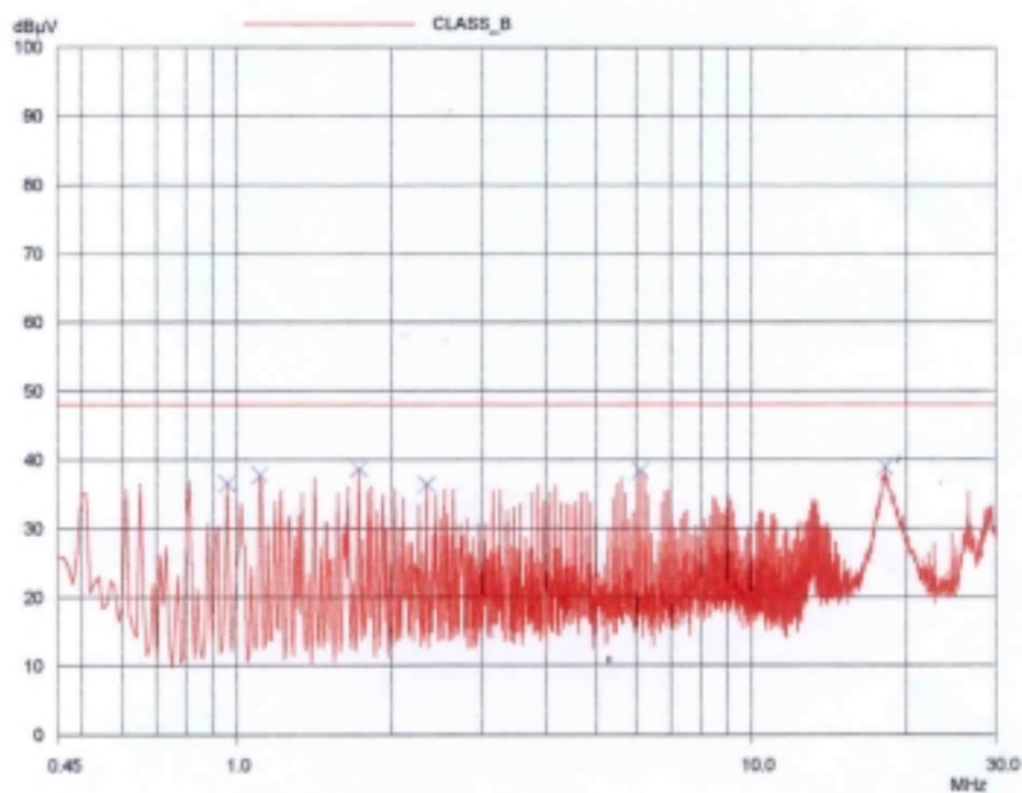
HOT LINE
