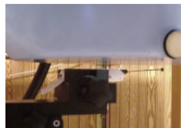
Body SAR Test Setup
