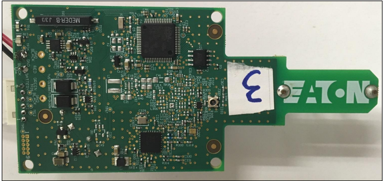
Photograph 2. EUT Photo, 2
