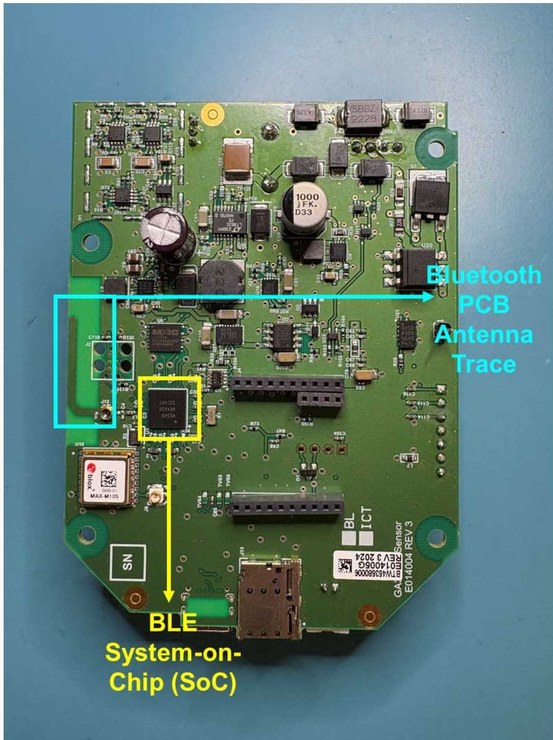
Figure 4: GridAdvisor 3 PCB – Top
