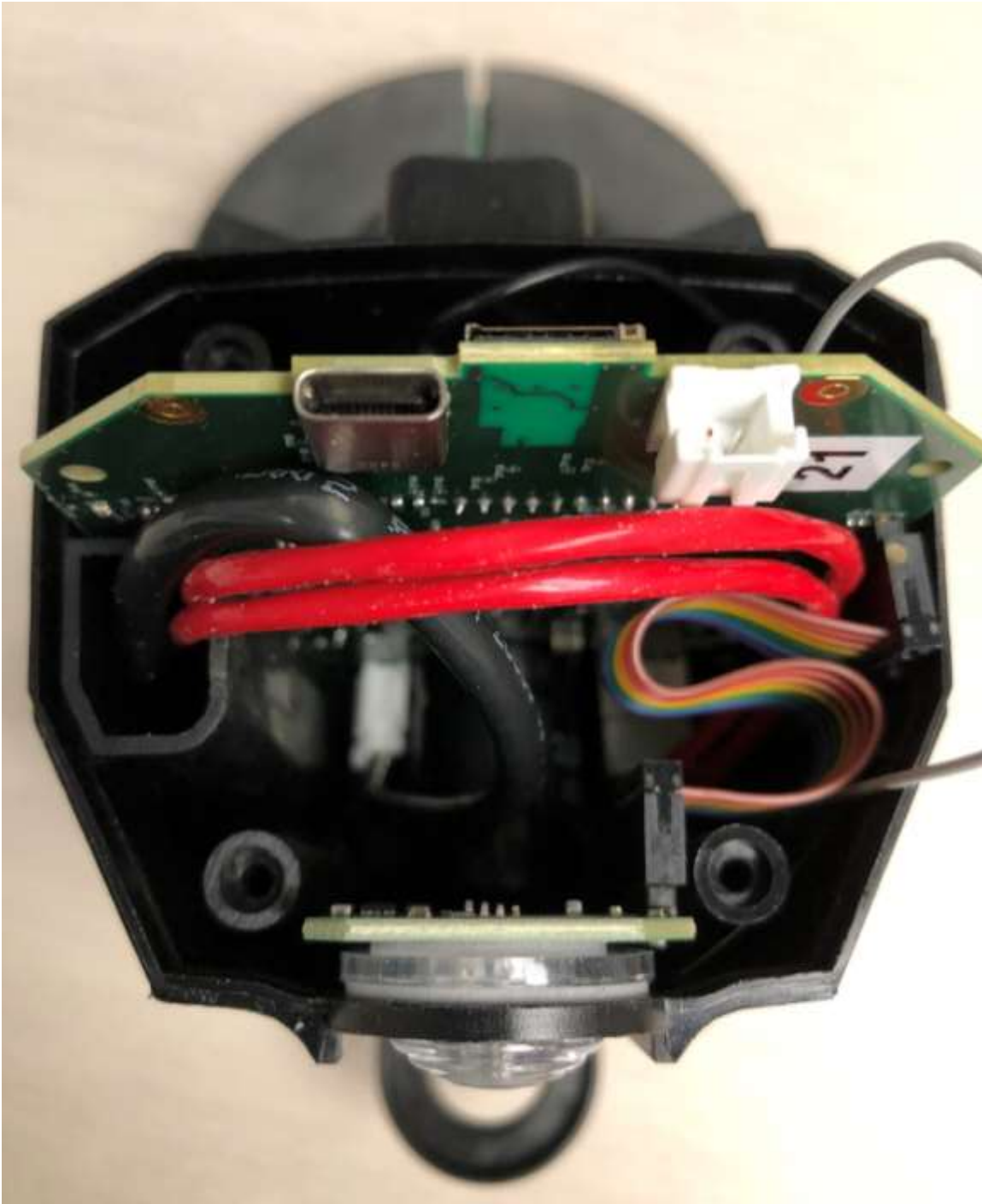
Figure 2: GridAdvisor 3 Internal View Without Cover
