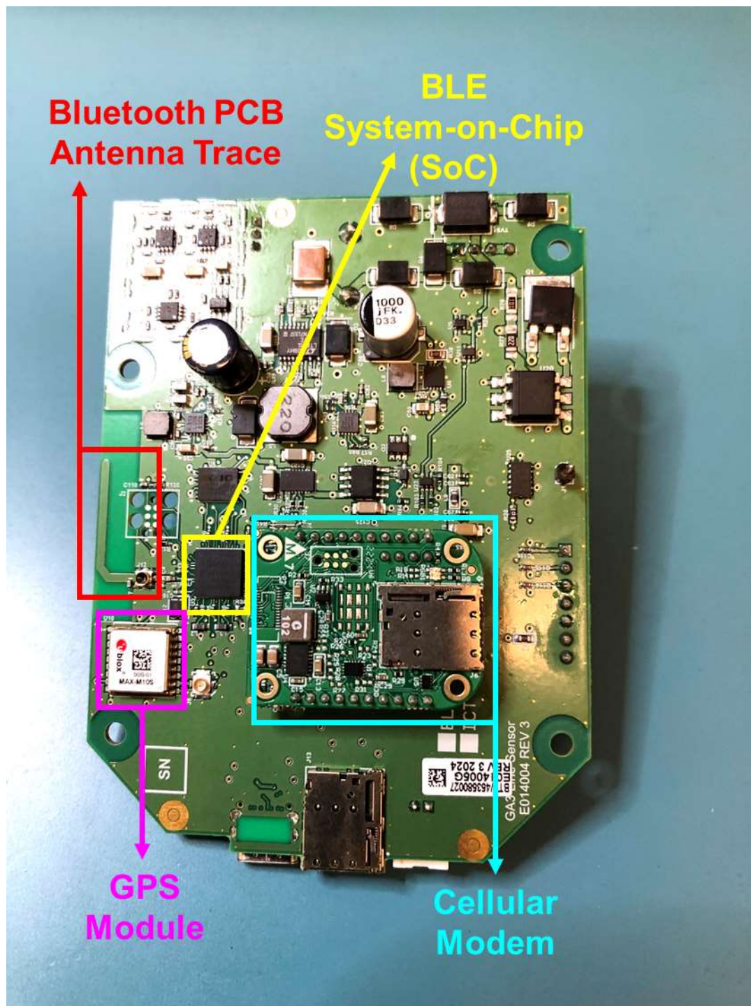
Figure 3: GridAdvisor 3 PCB – Top with Cellular Modem
