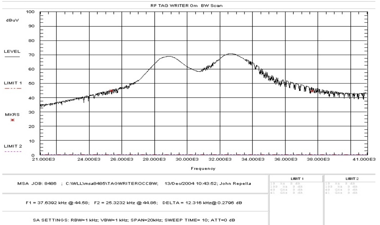
Figure 1. Occupied Bandwidth
