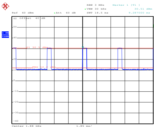
1880MHz - 80% AM
