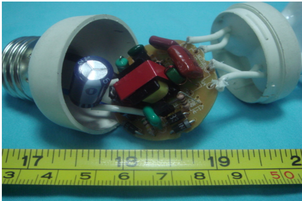
PCB-Front View for ELS-M13(ELS-M14)
