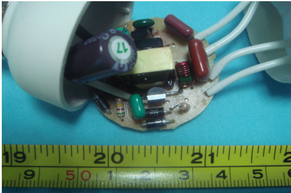
PCB-Back View for ELS-M9
