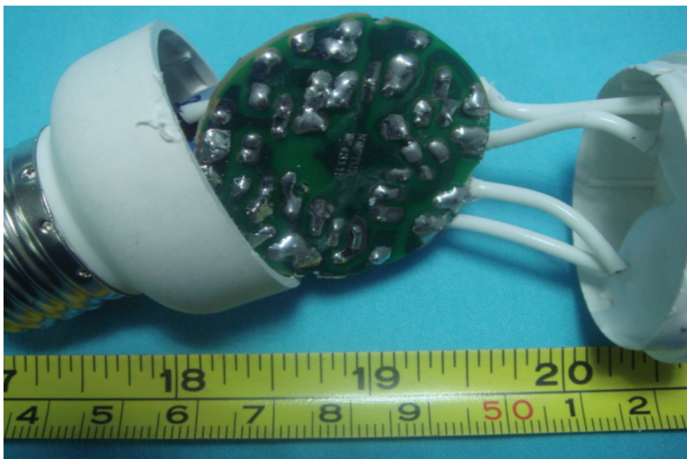
PCB-Back View for ELS-M13(ELS-M14)
