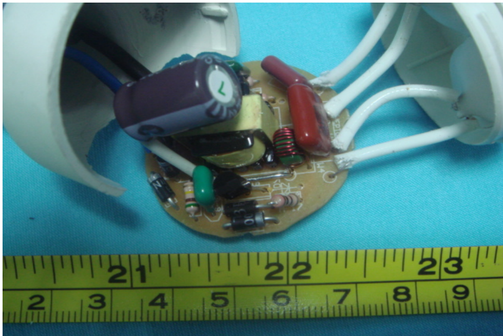
PCB-Back View for ELS-M7
