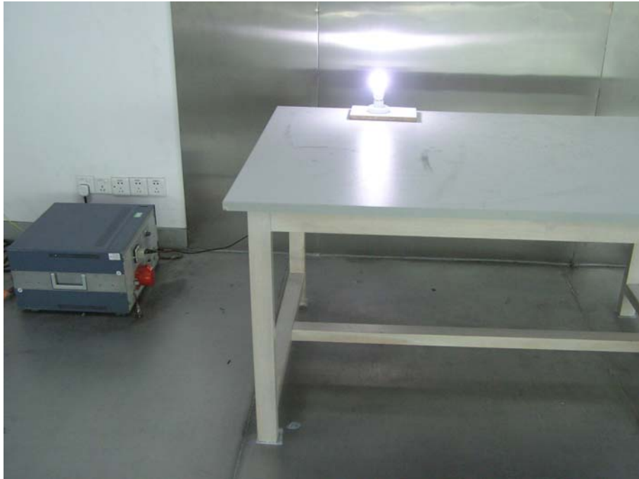
F611W: Conducted Emission - Front View
