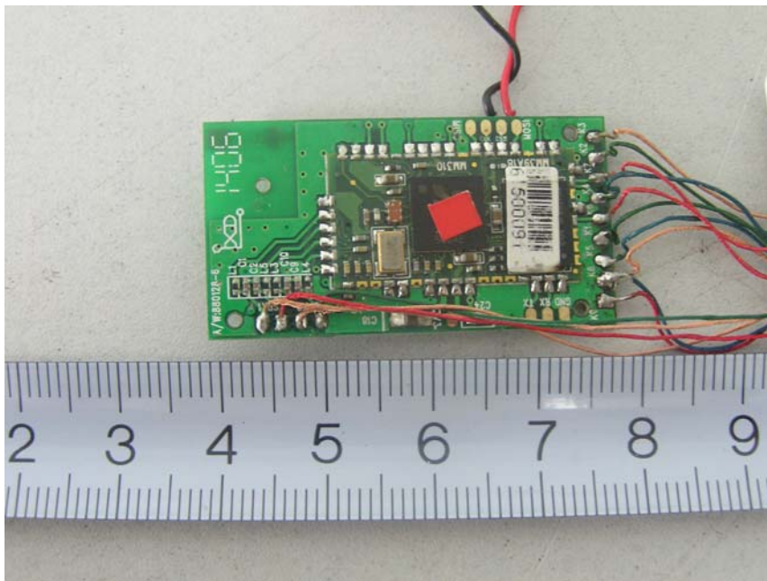
EUT- PCB Bottom View (1)
