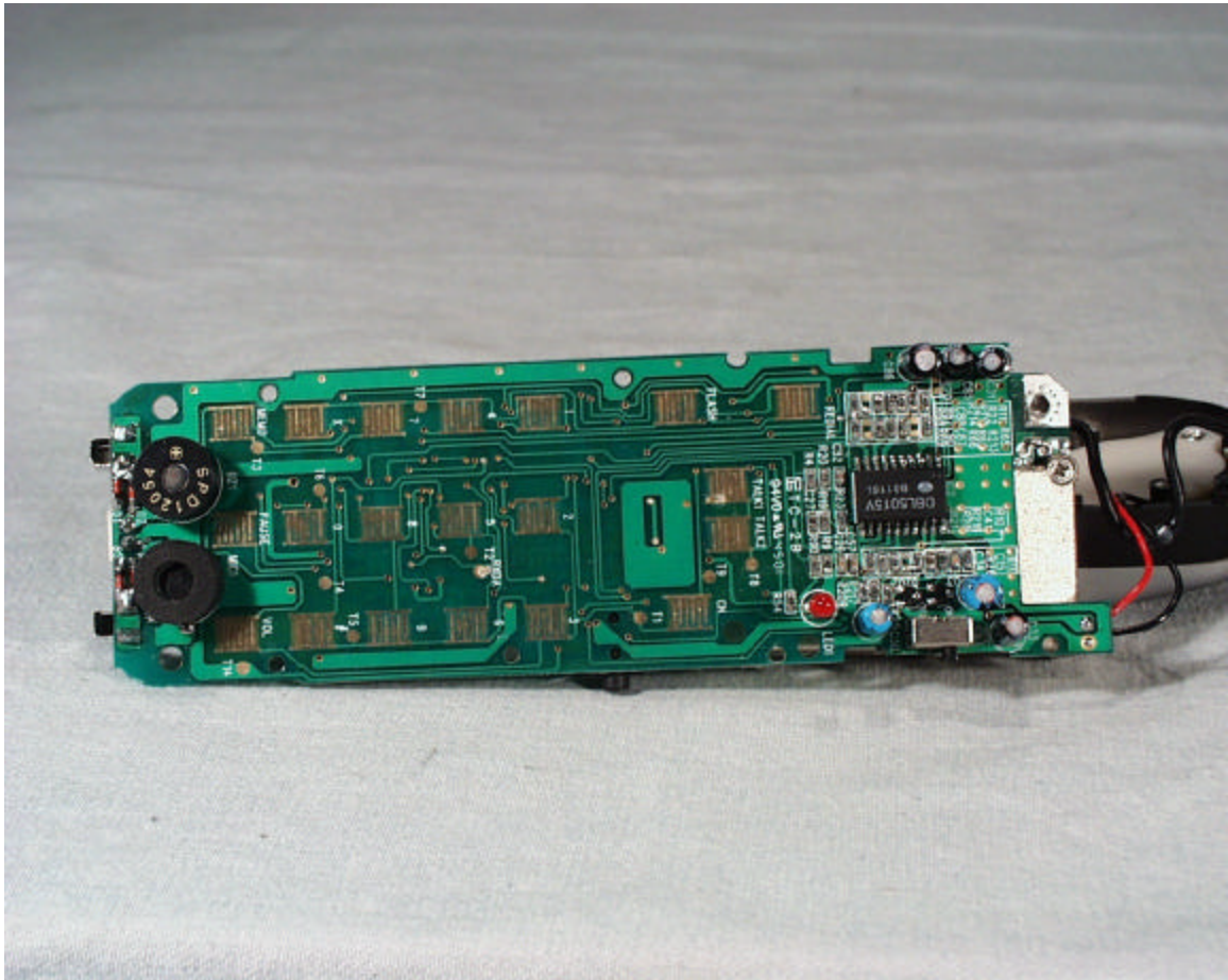
Bottom View of the Handset PCB
