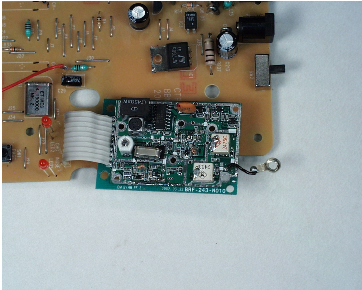
Side A of the Base RF PCB
