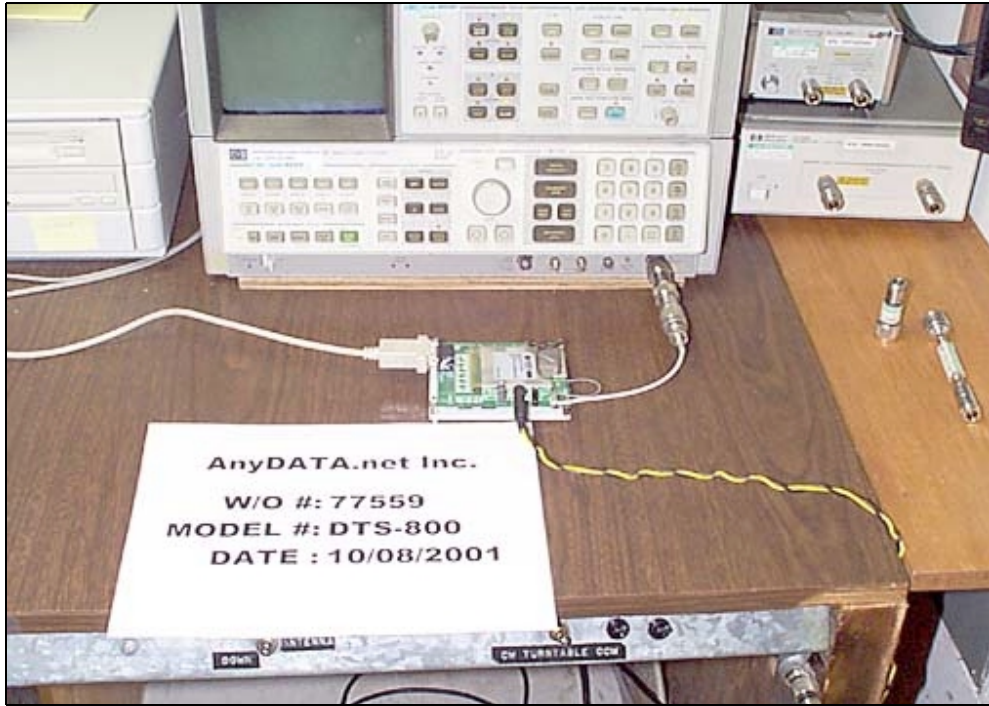
Setup for Bandwidth Testing
