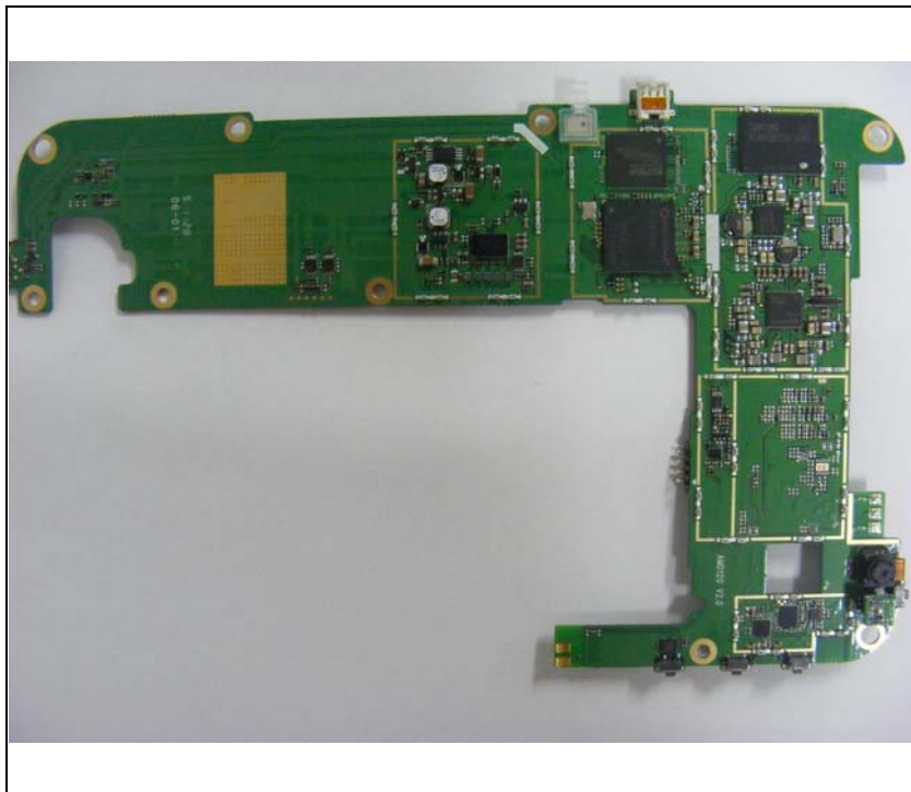
Top view of main board (without shield cap)
