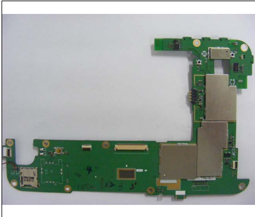
Bottom view of main board (without shield cap)
