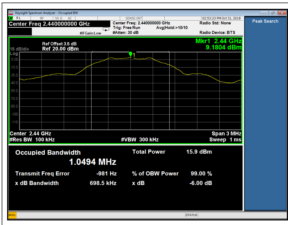
(Channel 19, 2440 MHz)
