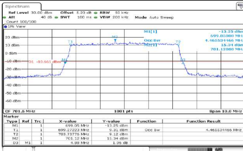
Band12-5MHz-16QAM-23035-25RB#0-4.466
