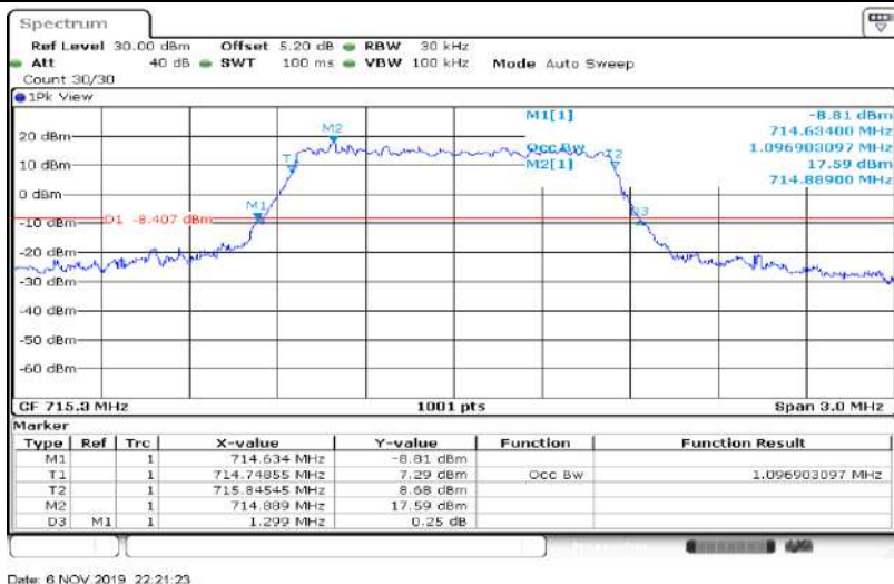
Band12-3MHz-QPSK-23025-15RB#0-2.697
