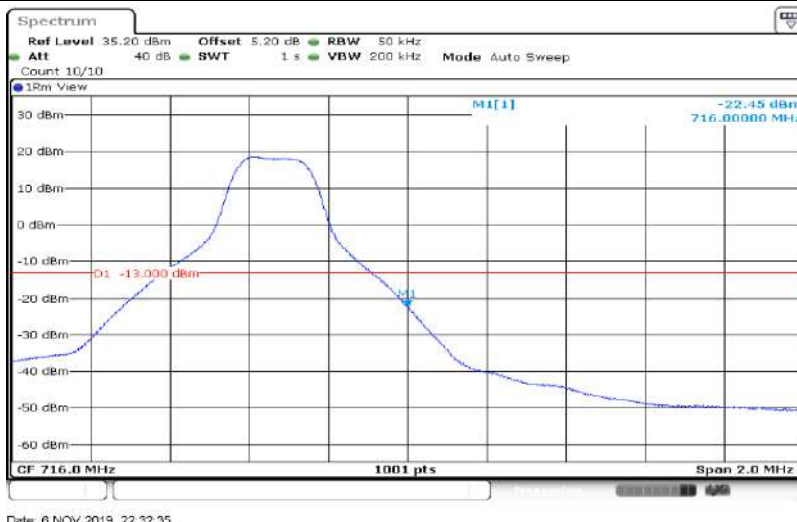
Band12-5MHz-QPSK-23155-25RB#0
