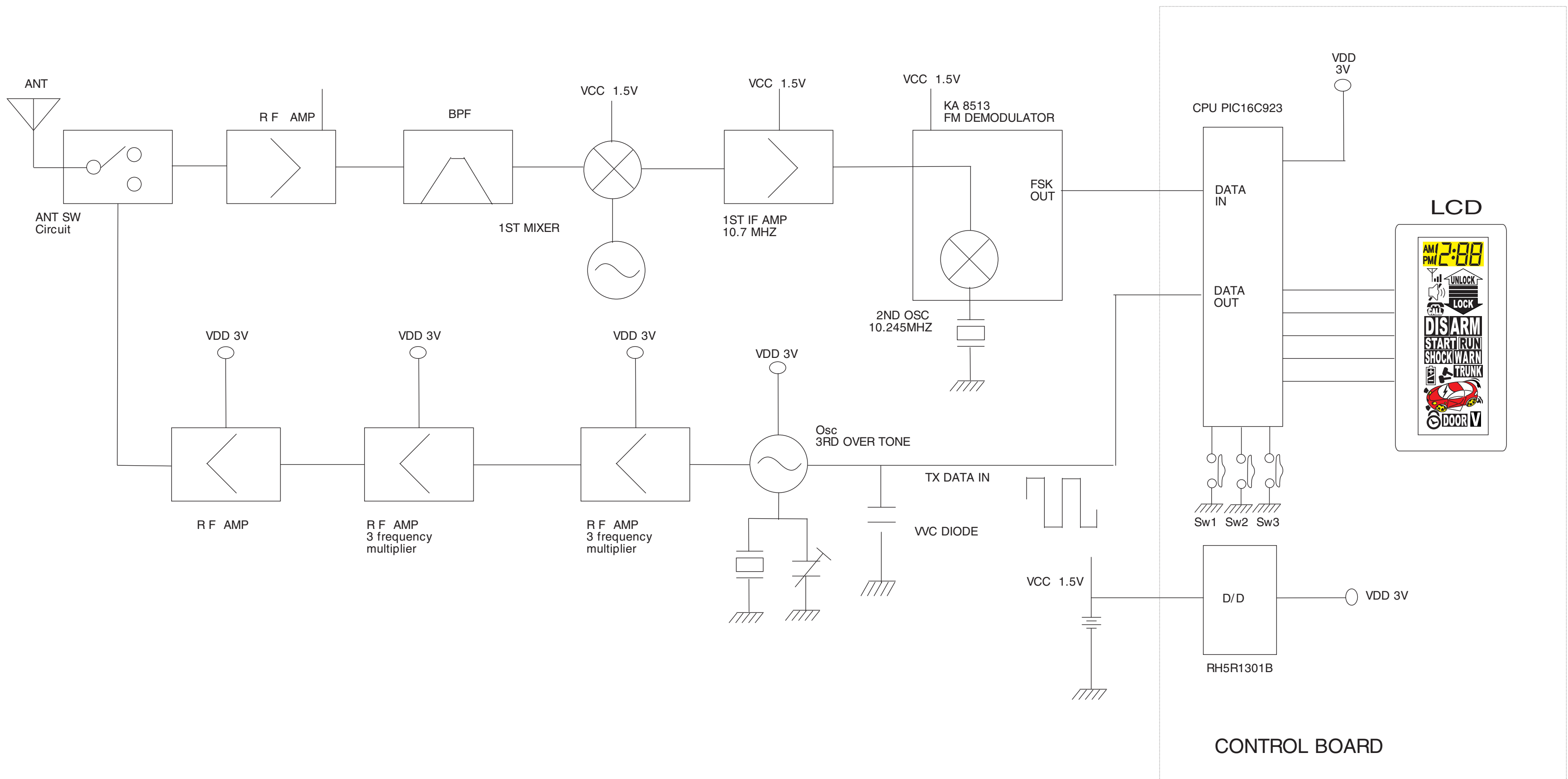
REMOCON BLOCK DIAGRAM
