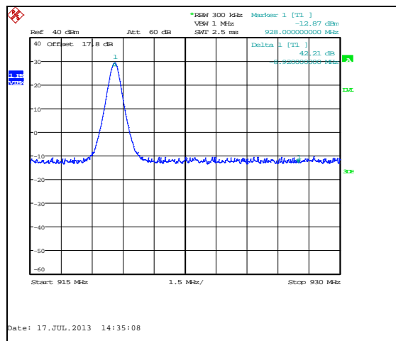
Figure 7.5.1.2-2: Upper Band-edge
