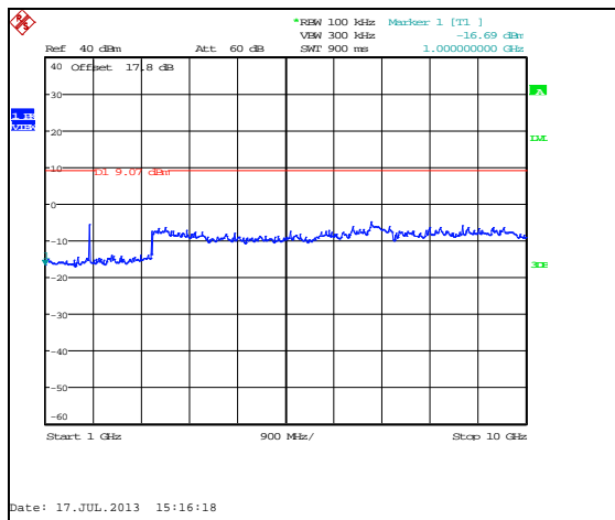
Figure 7.5.2.2-4: 1 GHz – 10 GHz – HCH
