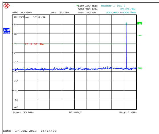
Figure 7.5.2.2-3: 30 MHz – 1 GHz – HCH
