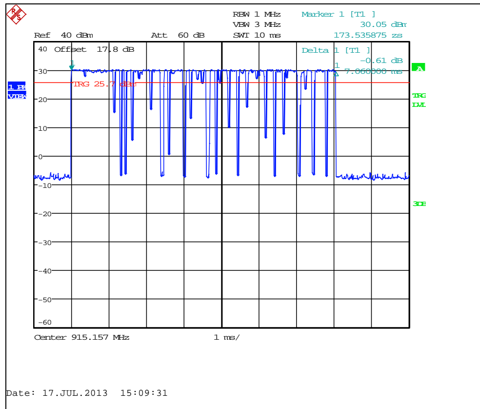
Figure 7.4.3.2-1: Dwell Time
