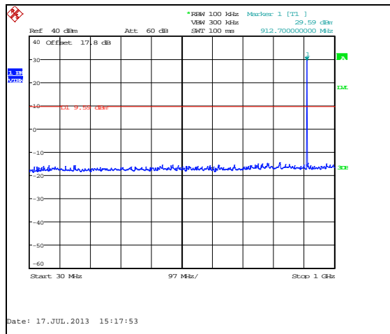
Figure 7.5.2.2-1: 30 MHz – 1 GHz – LCH
