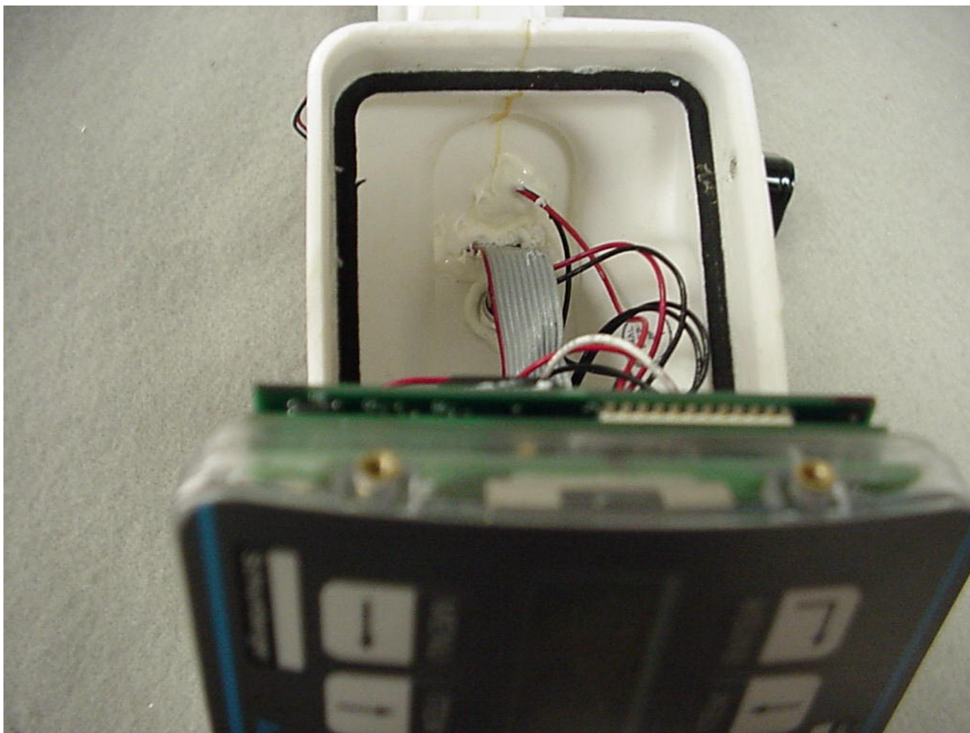
Photo 9. EUT, Top Portion of Product Opened
