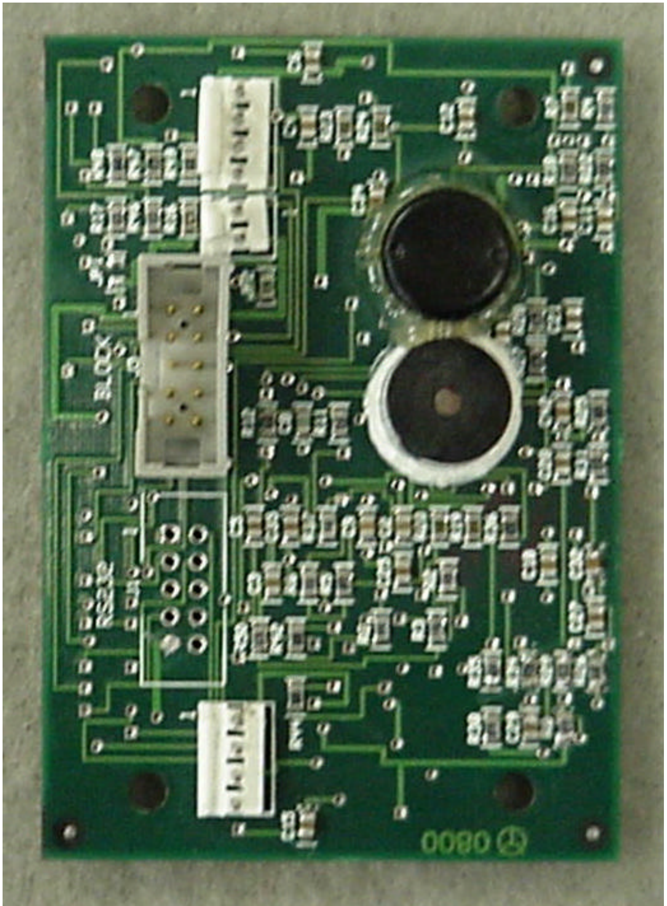
Photo 13, EUT, Bottom Side of Digital Board
