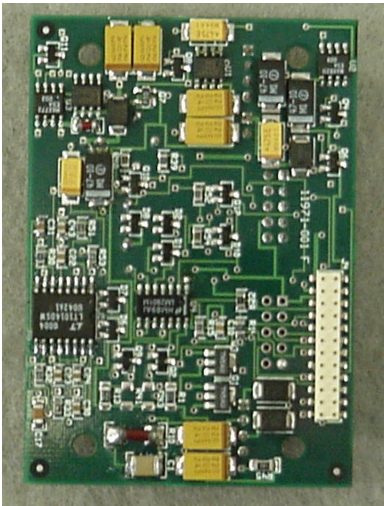
Photo 12, EUT, Top Side of Digital Board
