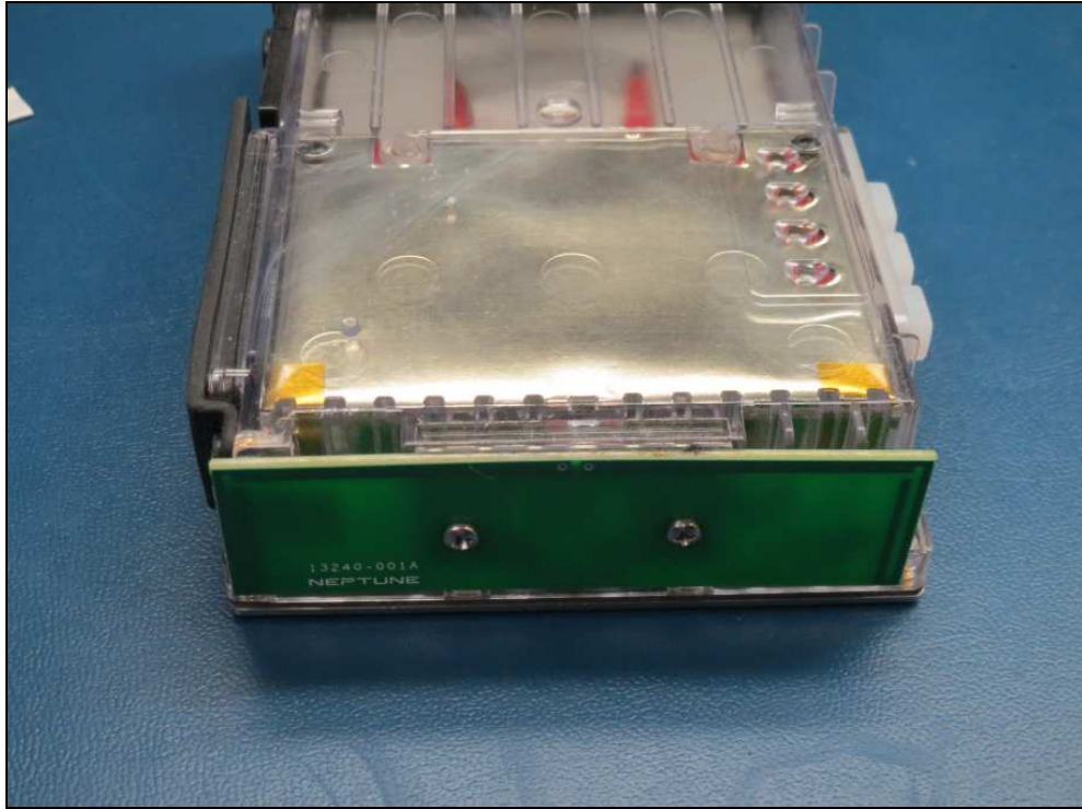
Figure 7: Internal Photo – PCB Stack Assembly, Antenna Board View
