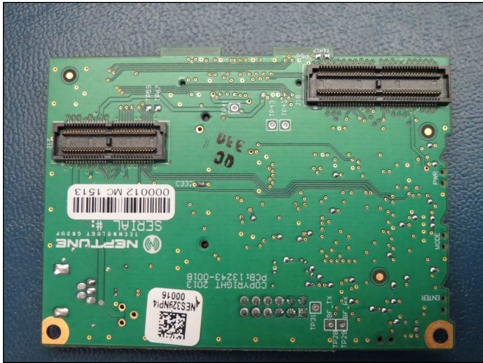
Figure 5: Internal Photo – I/O Board, Bottom
