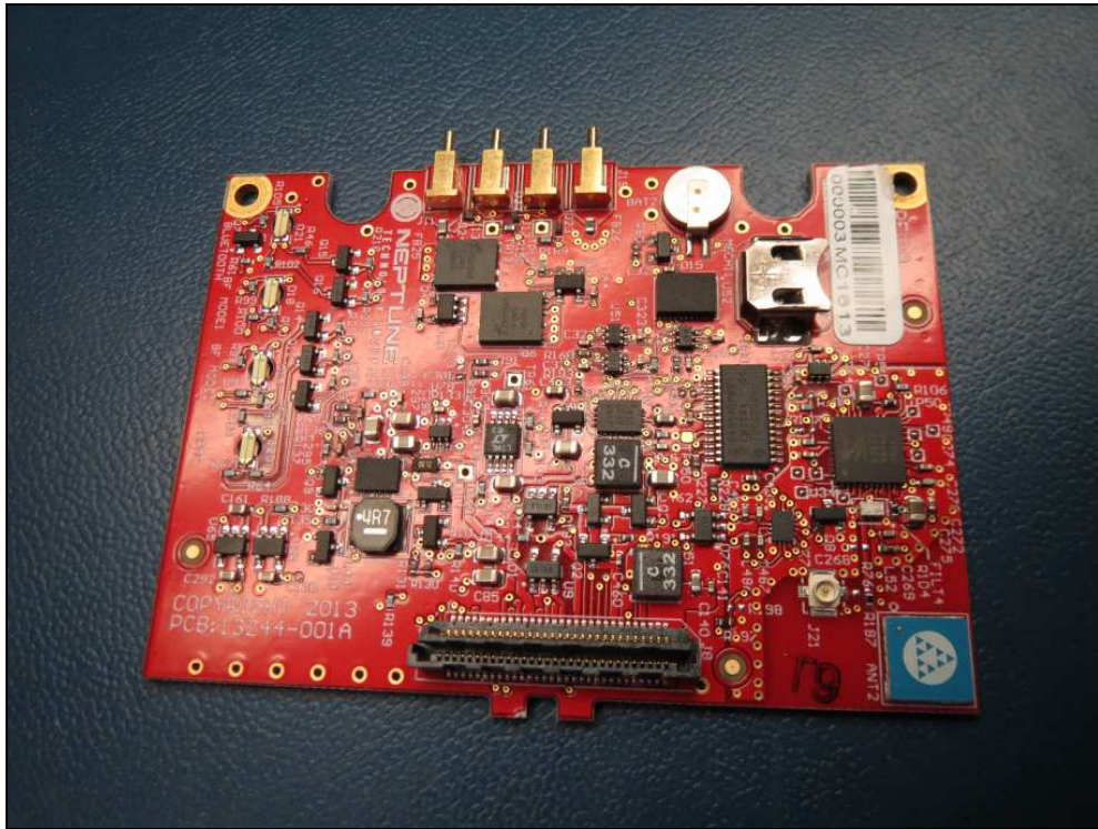
Figure 11: Internal Photo – Power Board, Top
