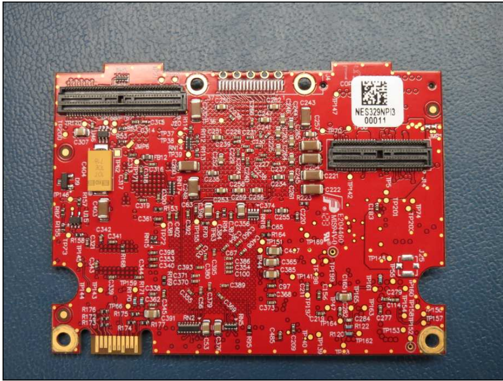
Figure 3: Internal Photo – Digital Board, Bottom
