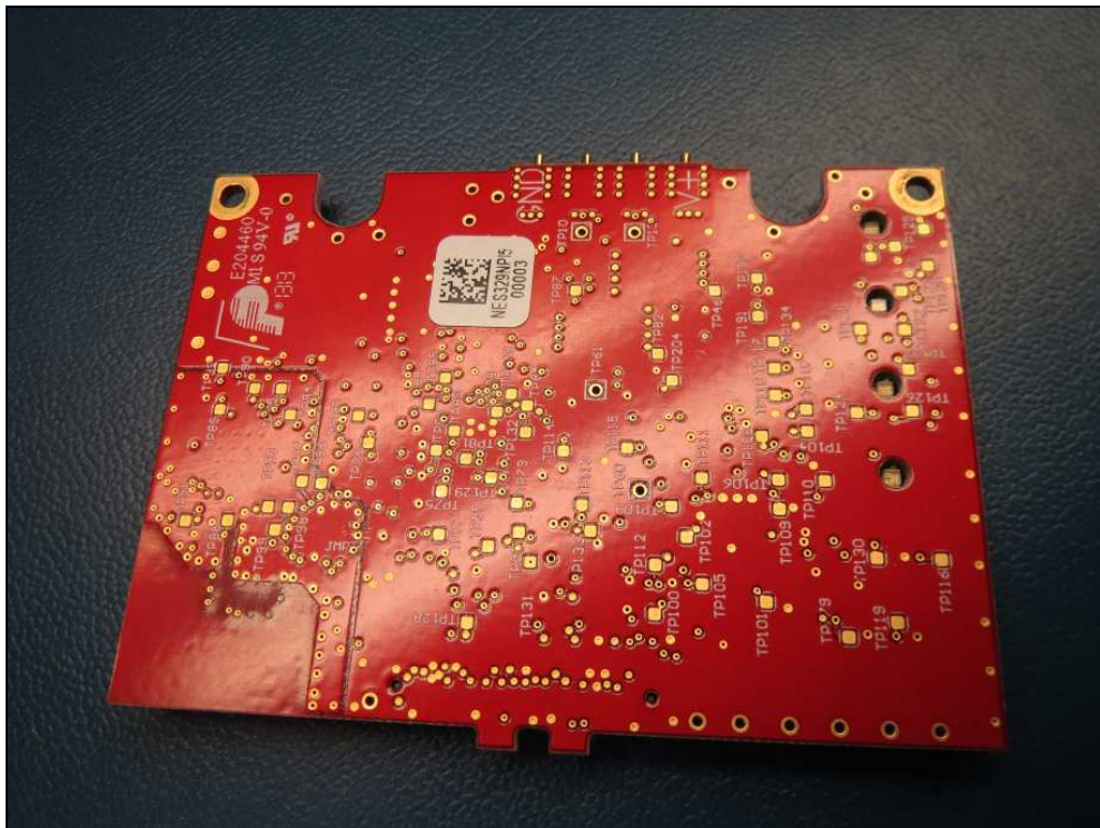
Figure 10: Internal Photo – Power Board, Bottom
