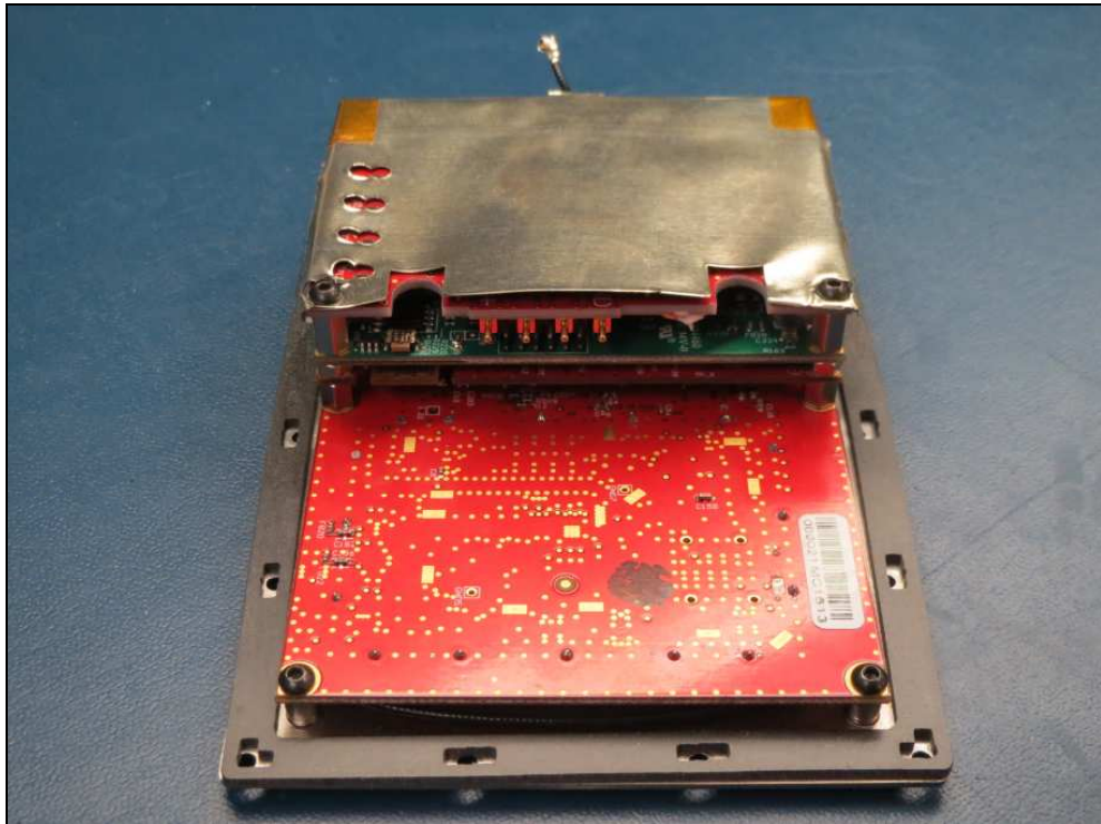
Figure 9: Internal Photo – PCB Stack Assembly, Top View
