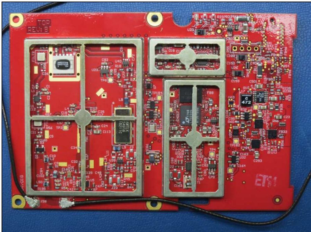
Figure 13: Internal Photo – RF Board, Top
