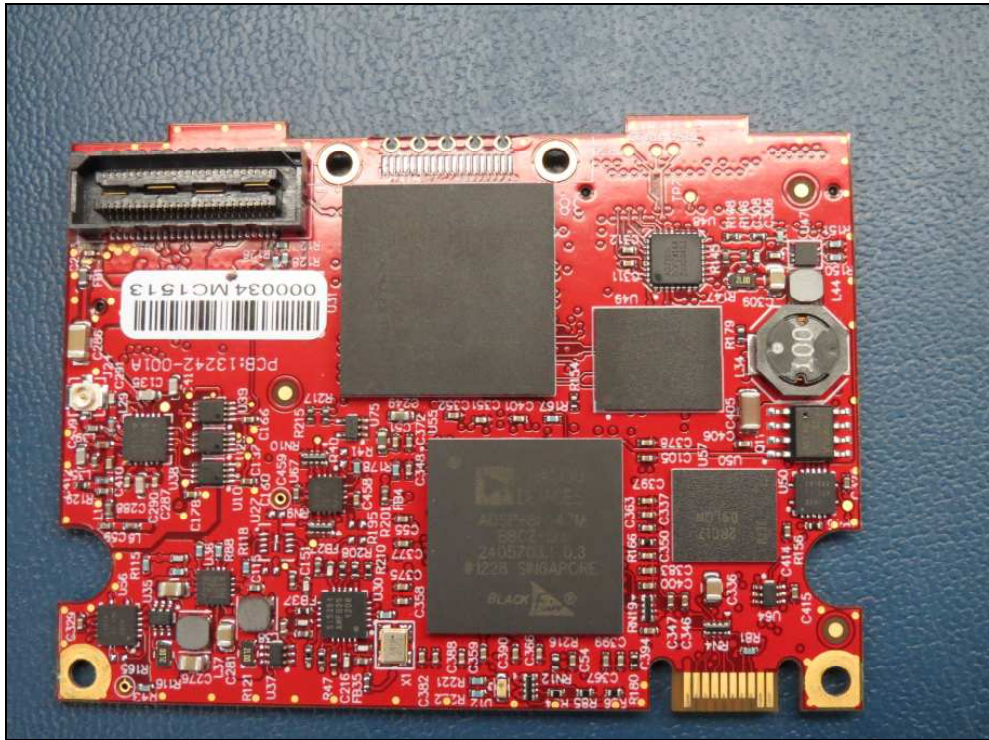
Figure 4: Internal Photo – Digital Board, Top
