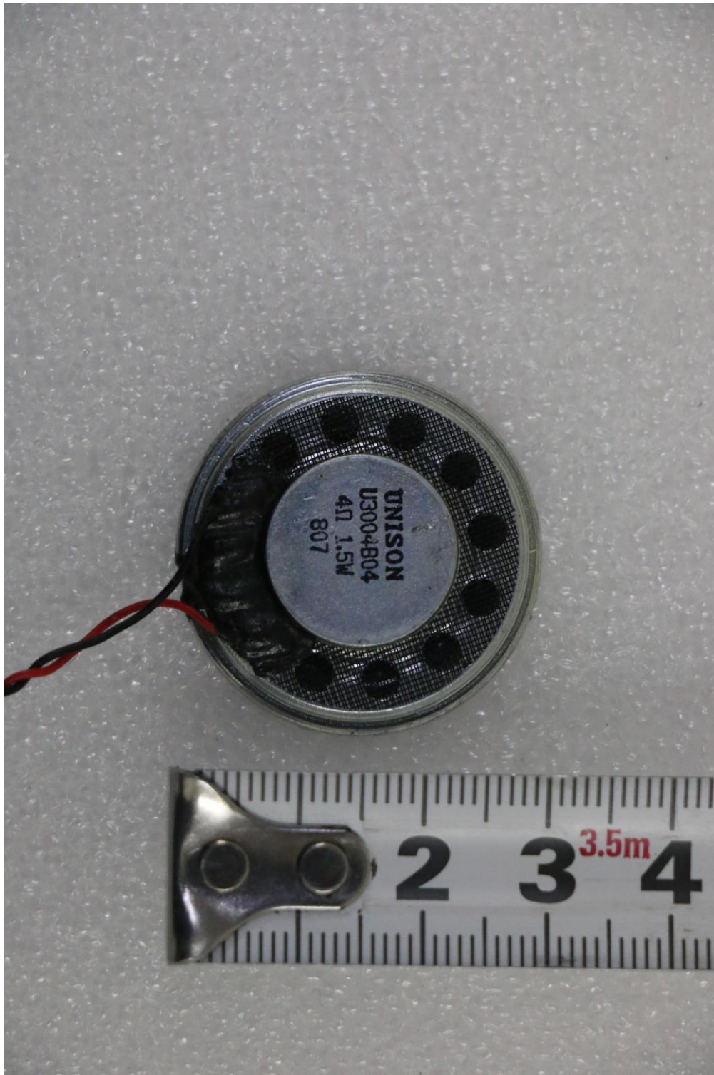
< Speaker bottom view >
