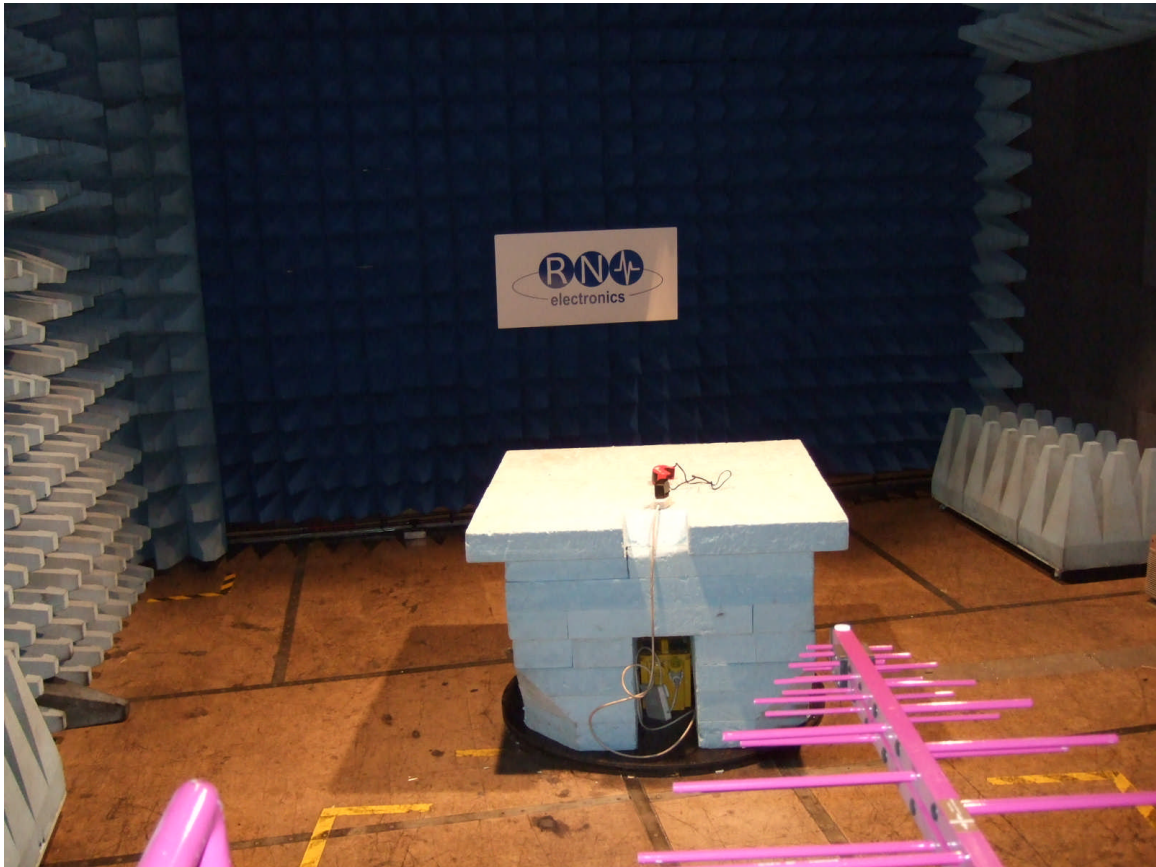
Radiated Emissions 2
