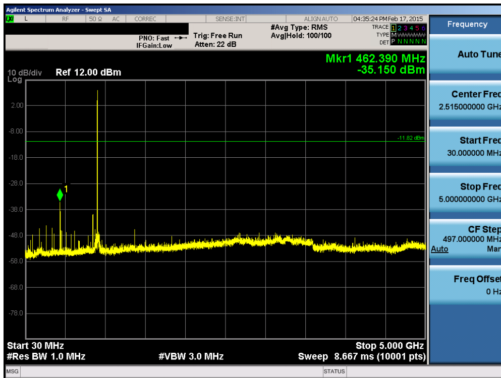
Plot 6-20. Conducted Spurious Plot (High Channel)
