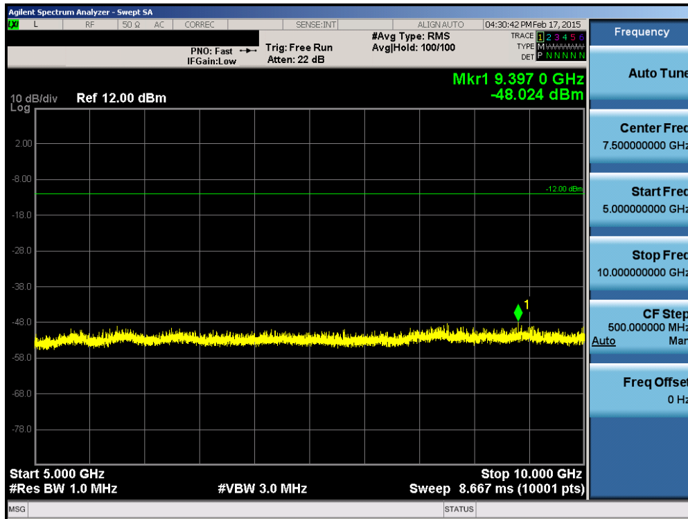
Plot 6-19. Conducted Spurious Plot (Mid Channel)
