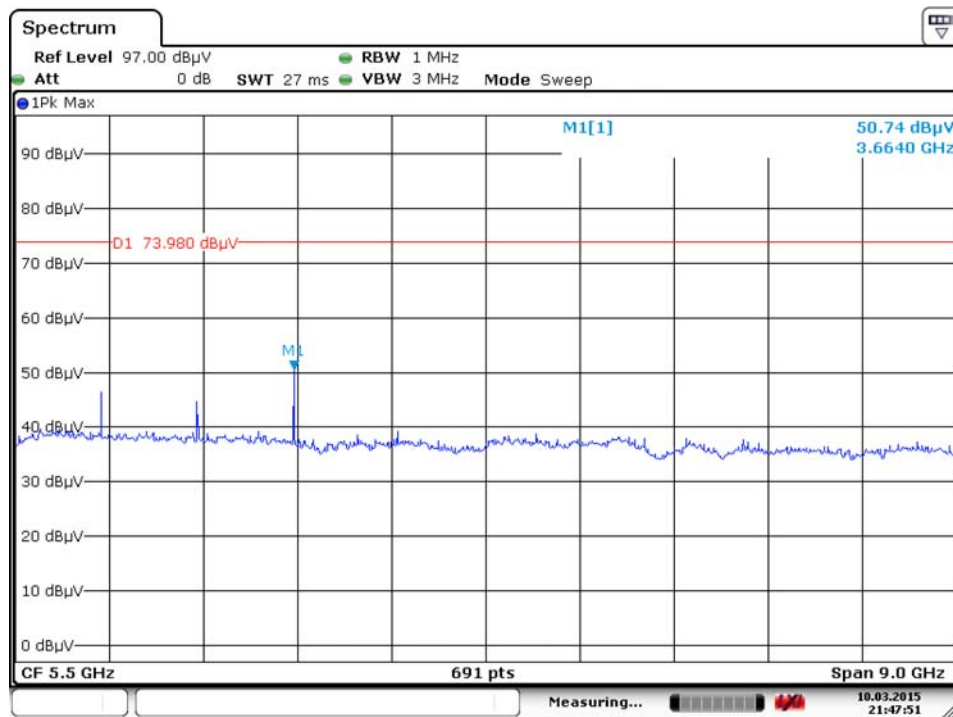
Plot 6-25. Radiated Spurious Plot above 1GHz (Mid Channel) (Pol. V)
