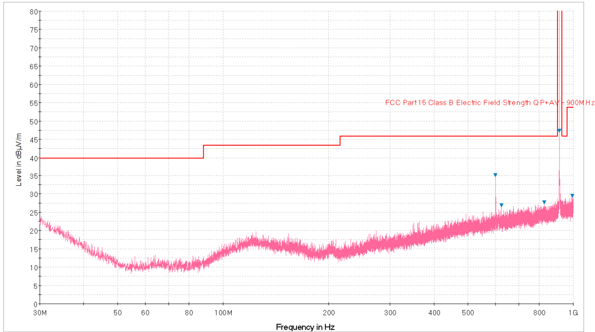
Plot 7-7. Radiated Spurious Plot below 1GHz (Pol. H)
