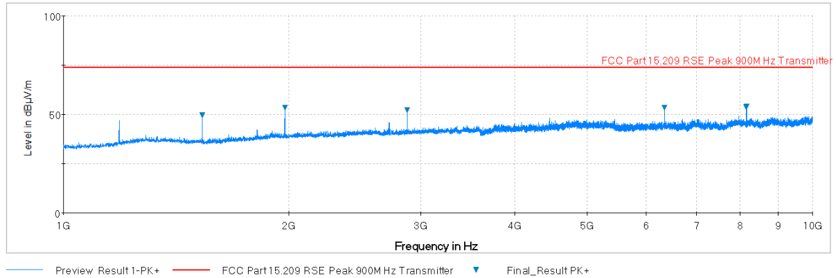
Plot 7-1. Radiated Spurious Plot above 1GHz (Low Channel) (Pol. H)
