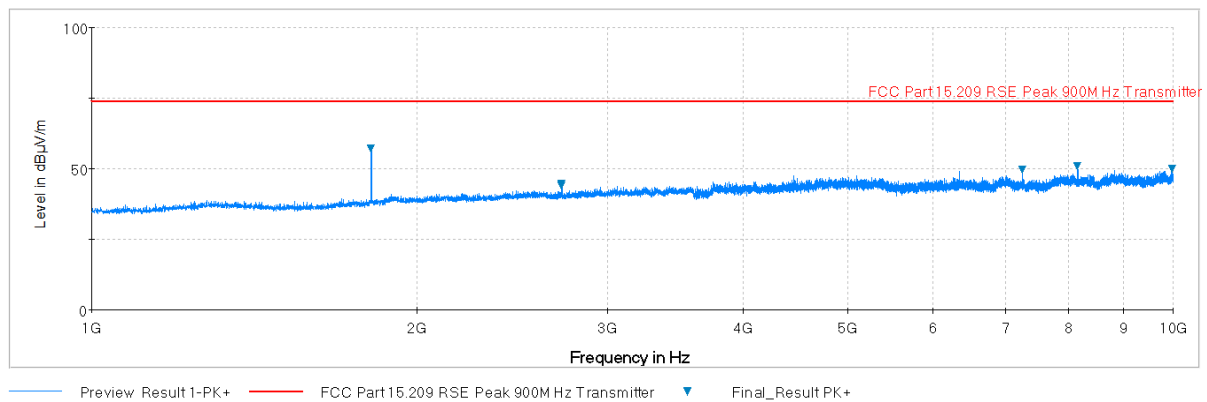
Plot 7-2. Radiated Spurious Plot above 1GHz (Low Channel) (Pol. V)
