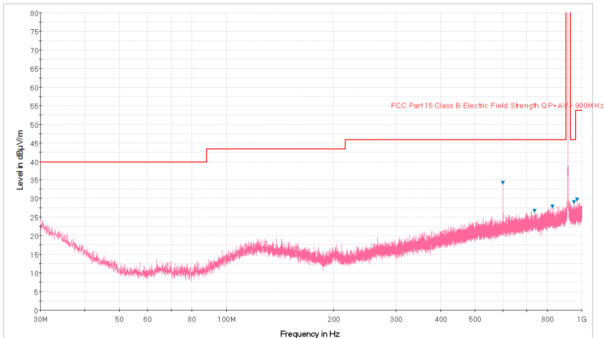
Plot 7-8. Radiated Spurious Plot below 1GHz (Pol. V)
