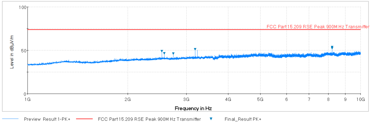
Plot 7-4. Radiated Spurious Plot above 1GHz (Mid Channel) (Pol. V)
