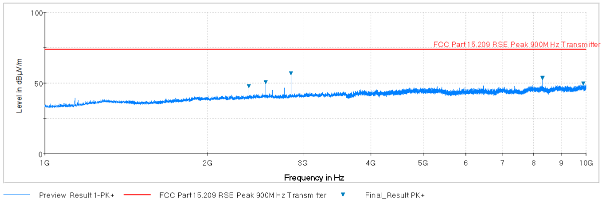
Plot 7-6. Radiated Spurious Plot above 1GHz (High Channel) (Pol. V)
