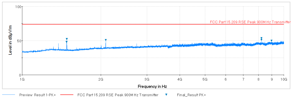
Plot 7-3. Radiated Spurious Plot above 1GHz (Mid Channel) (Pol. H)
