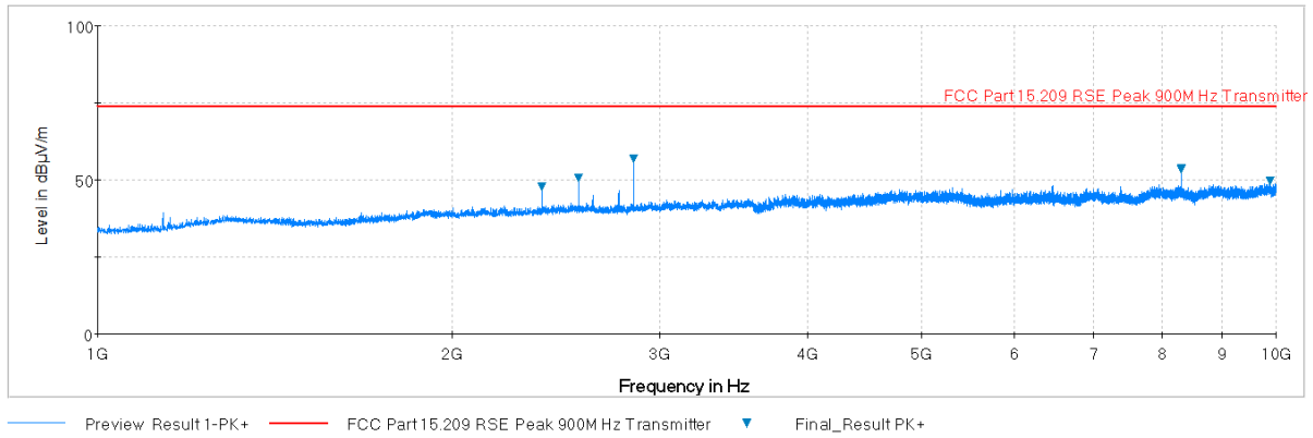
Plot 7-5. Radiated Spurious Plot above 1GHz (High Channel) (Pol. H)
