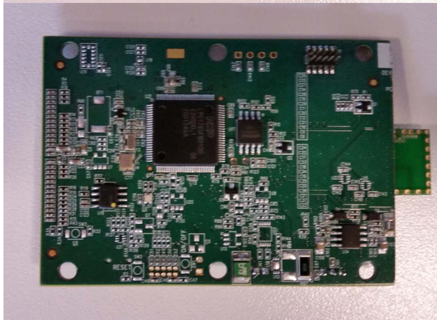
OXW-DS0028 WiFi Board (PA0021)
