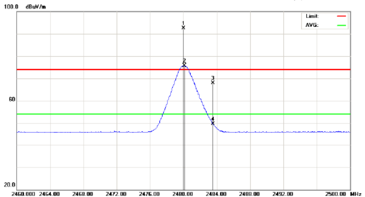
TX CH 05 (Restricted Bands Requirements, Horizontal)
