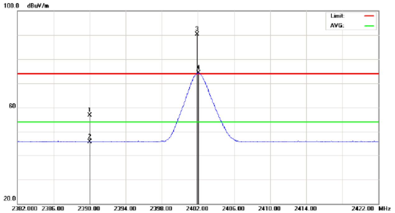
TX CH 05 (Restricted Bands Requirements, Vertical)
