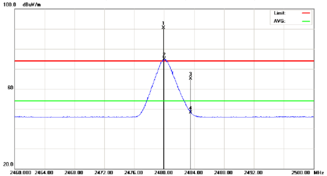
TX CH 05 (Restricted Bands Requirements, Vertical)
