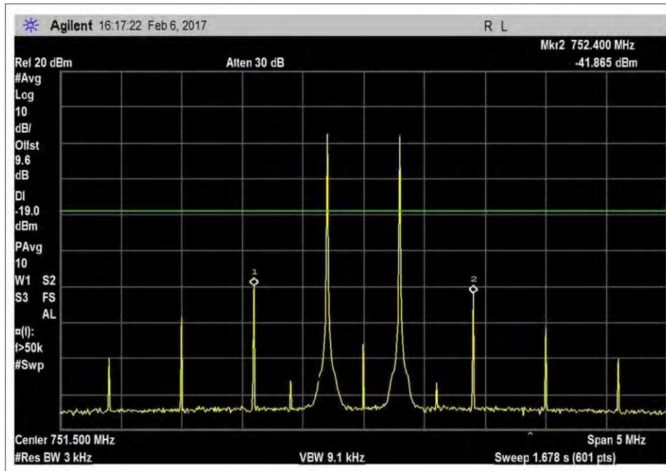
7.4_Intermod_DL_746-757MHz
