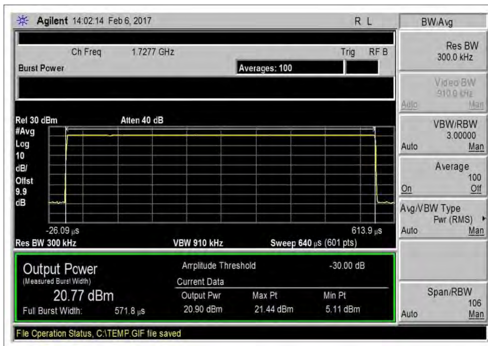
7.2_Power_UL_1710-1755MHz-Max
