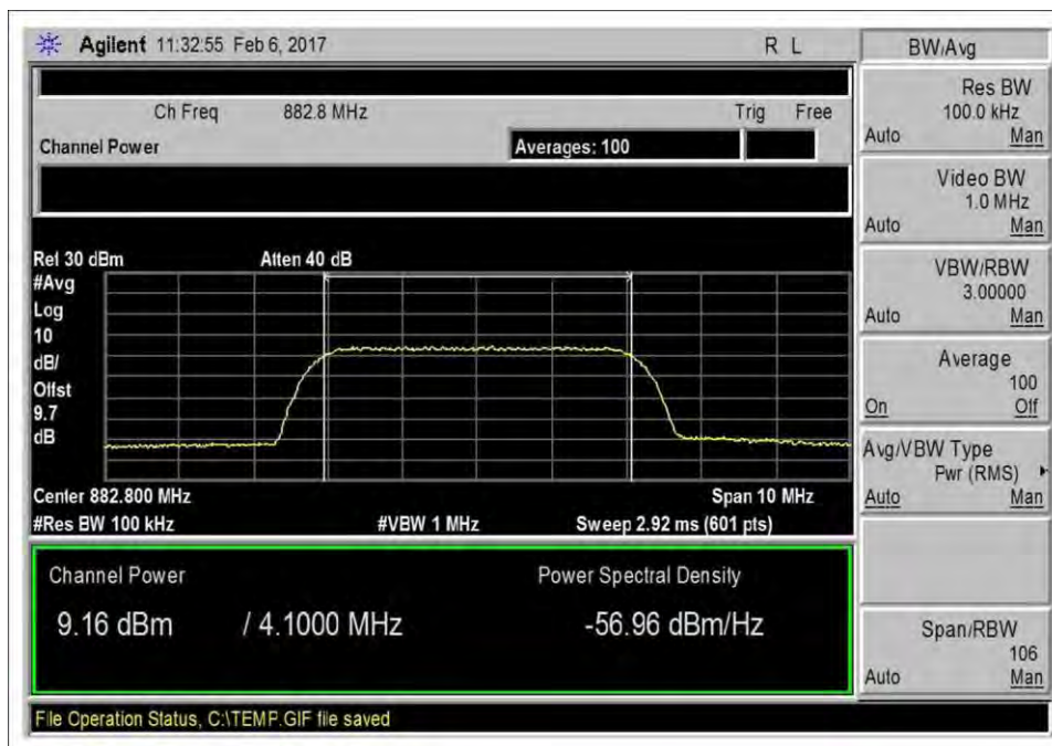
7.2_Power_DL_869-894MHz-Max
