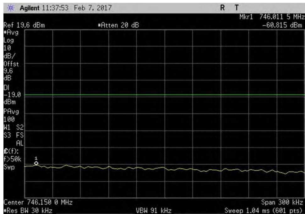
7.5_OBE_DL_728-746MHz_H_PreAGC_CDMA
