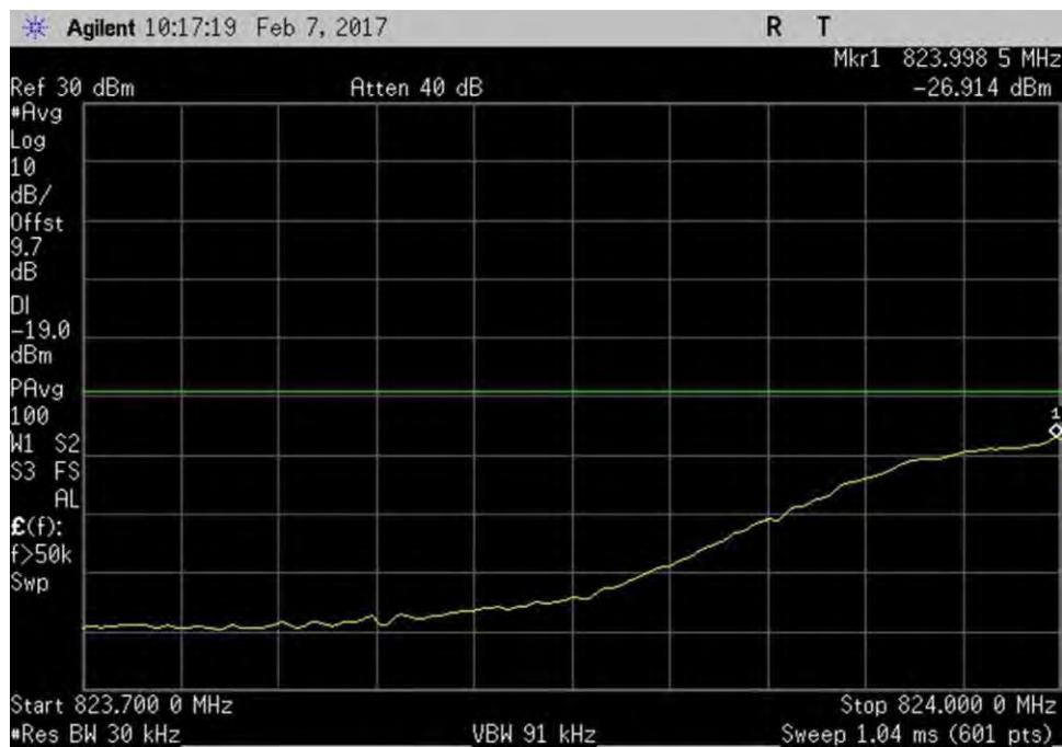
7.5_OBE_UL_824-849MHz_L_PreAGC_GSM
