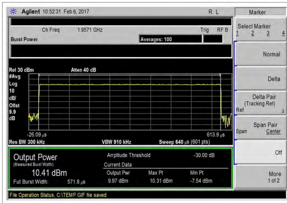
7.2_Power_DL_1930-1995MHz
