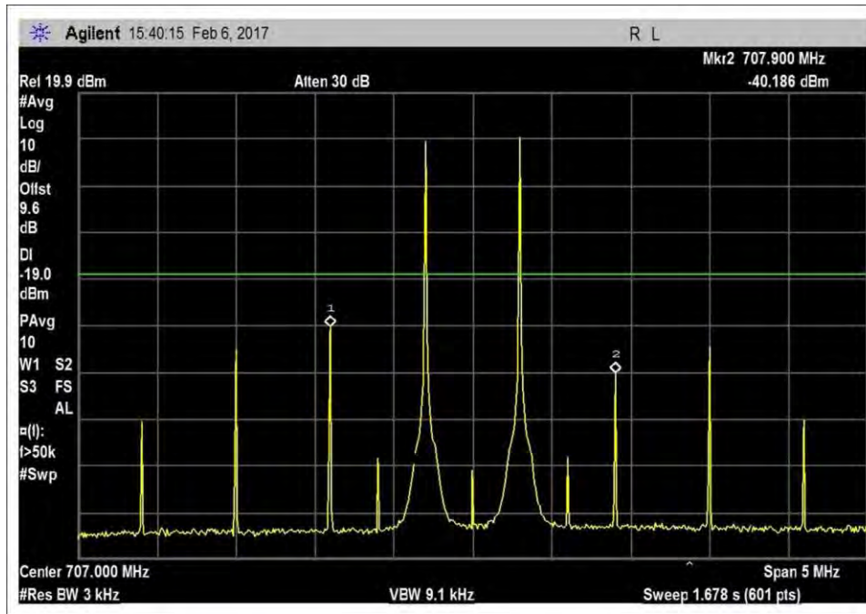
7.4_Intermod_UL_698-716MHz
