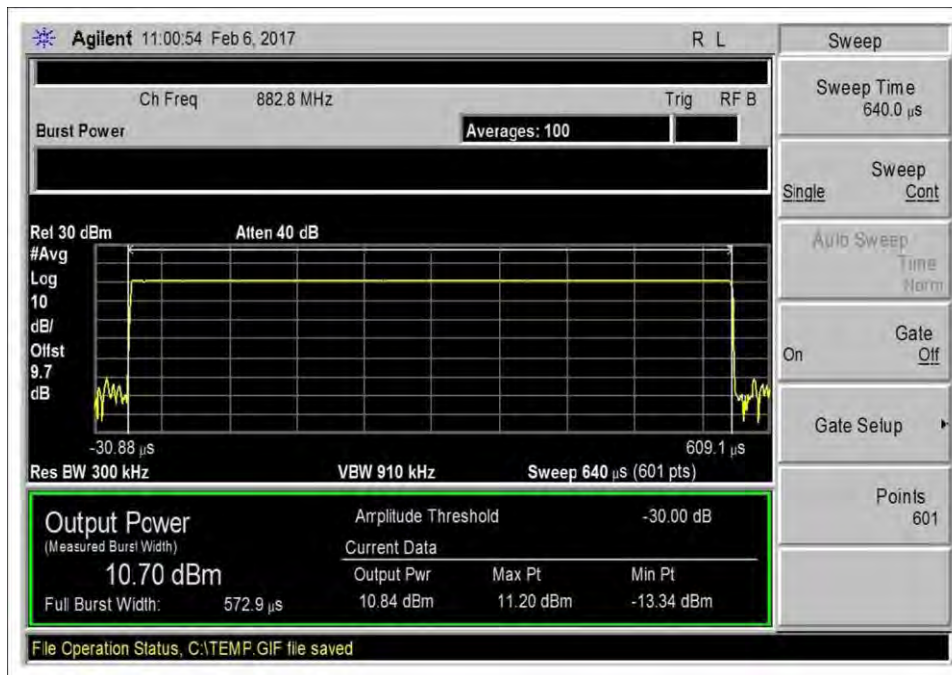
7.2_Power_DL_869-894MHz
