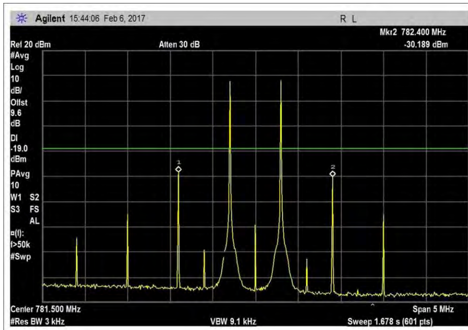
7.4_Intermod_UL_776-787MHz
