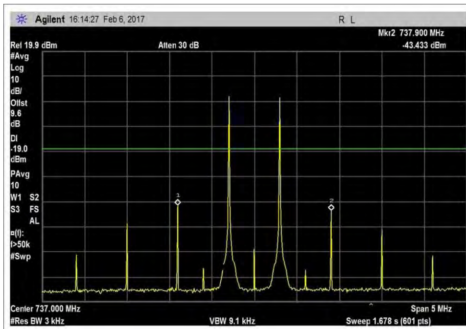
7.4_Intermod_DL_728-746MHz
