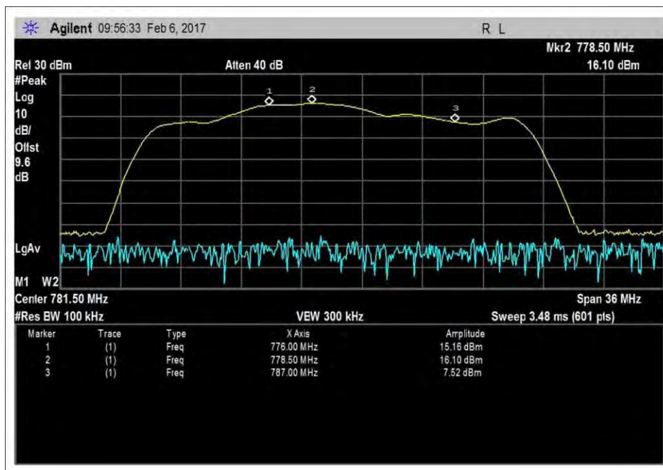
7.1_Band Verify_UL_776-787MHz-Zoom
