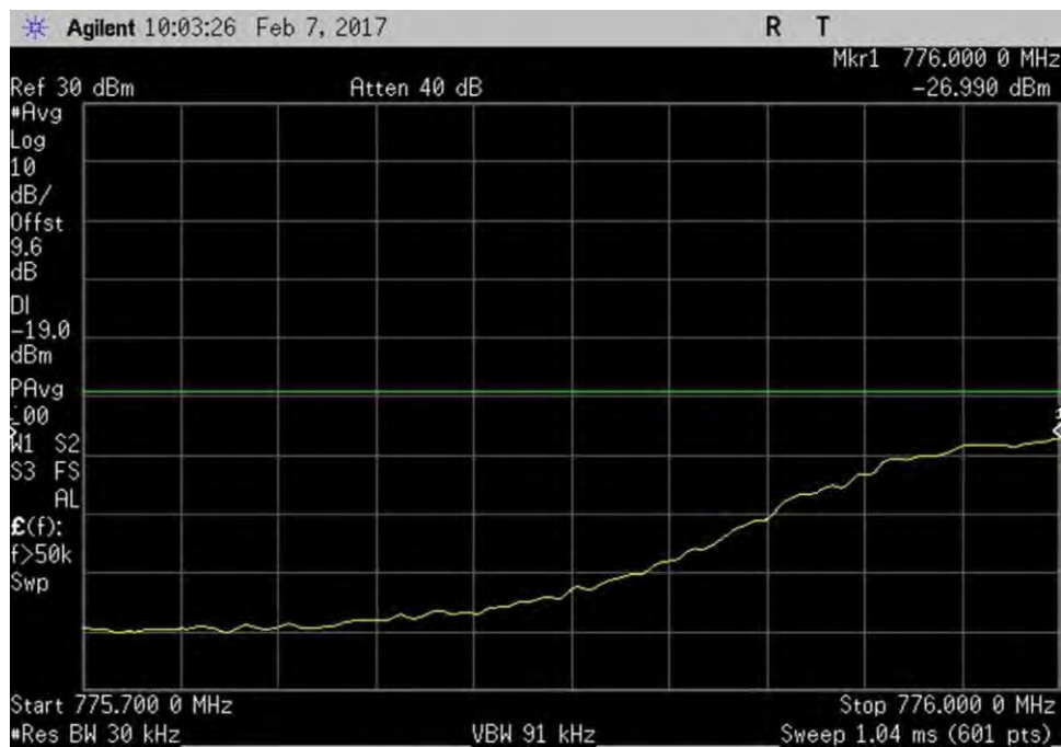
7.5_OBE_UL_776-787MHz_L_PreAGC_GSM
