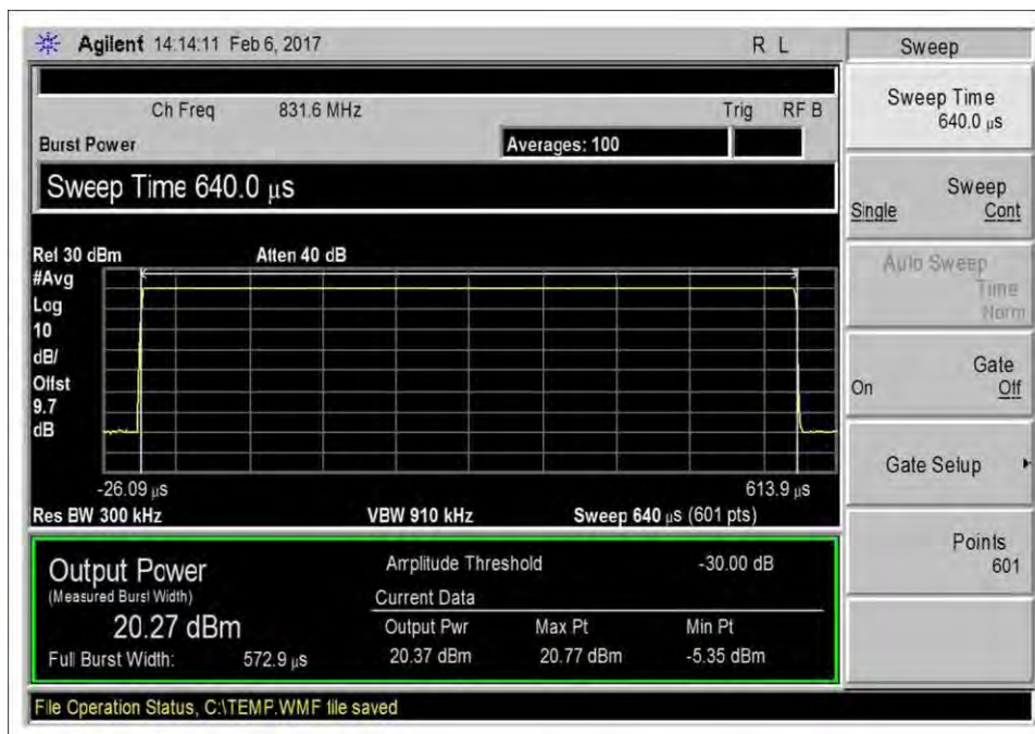
7.2_Power_UL_824-849MHz-Max
