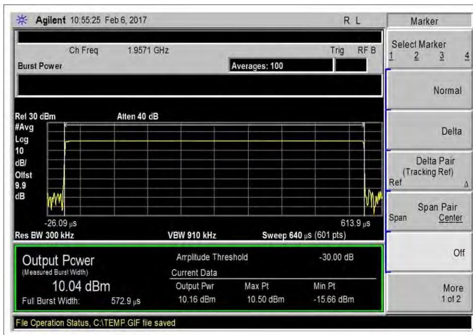
7.2_Power_DL_1930-1995MHz-Max
