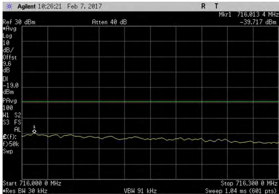
7.5_OBE_UL_698-716MHz_H_PreAGC_CDMA
