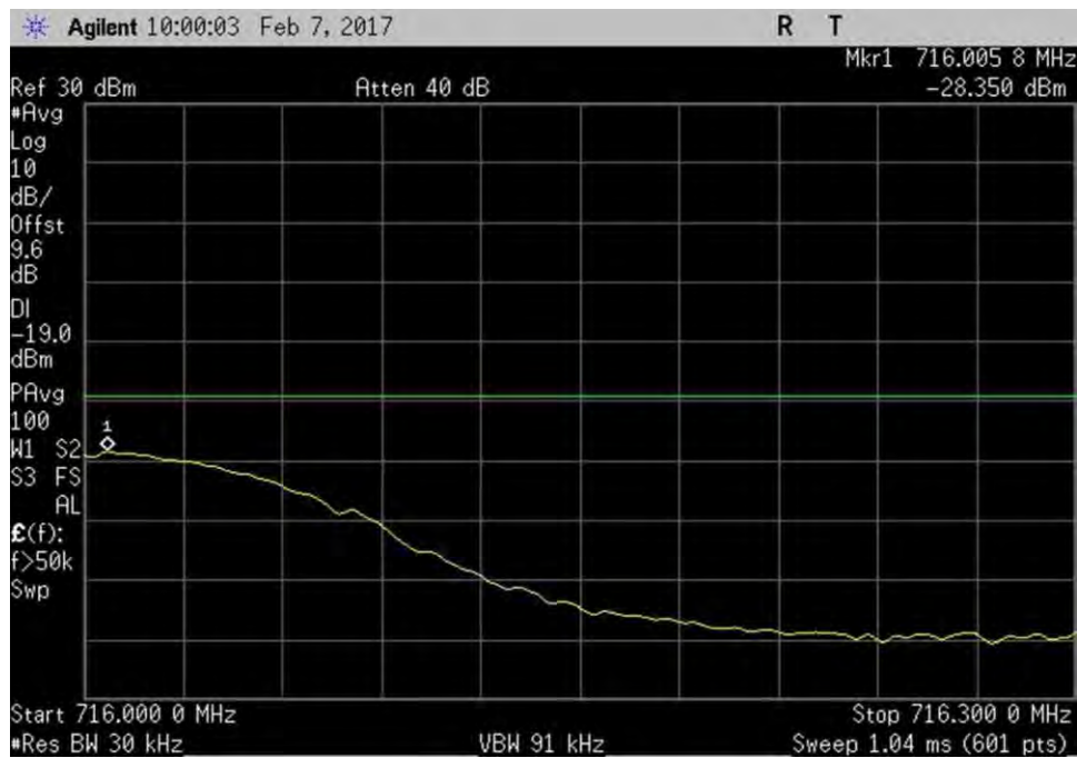
7.5_OBE_UL_698-716MHz_H_PreAGC_GSM
