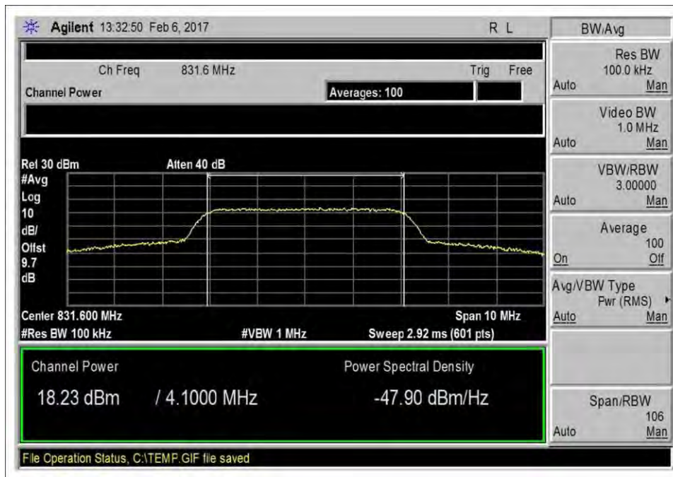
7.2_Power_UL_824-849MHz
