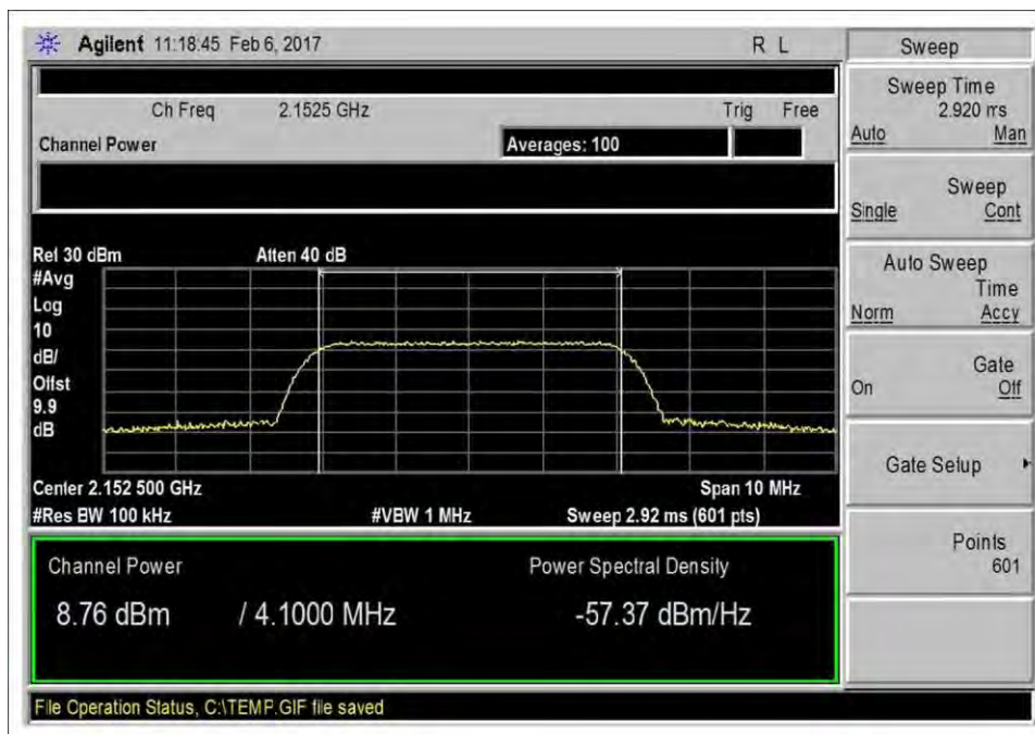
7.2_Power_DL_2110-2155MHz-Max
