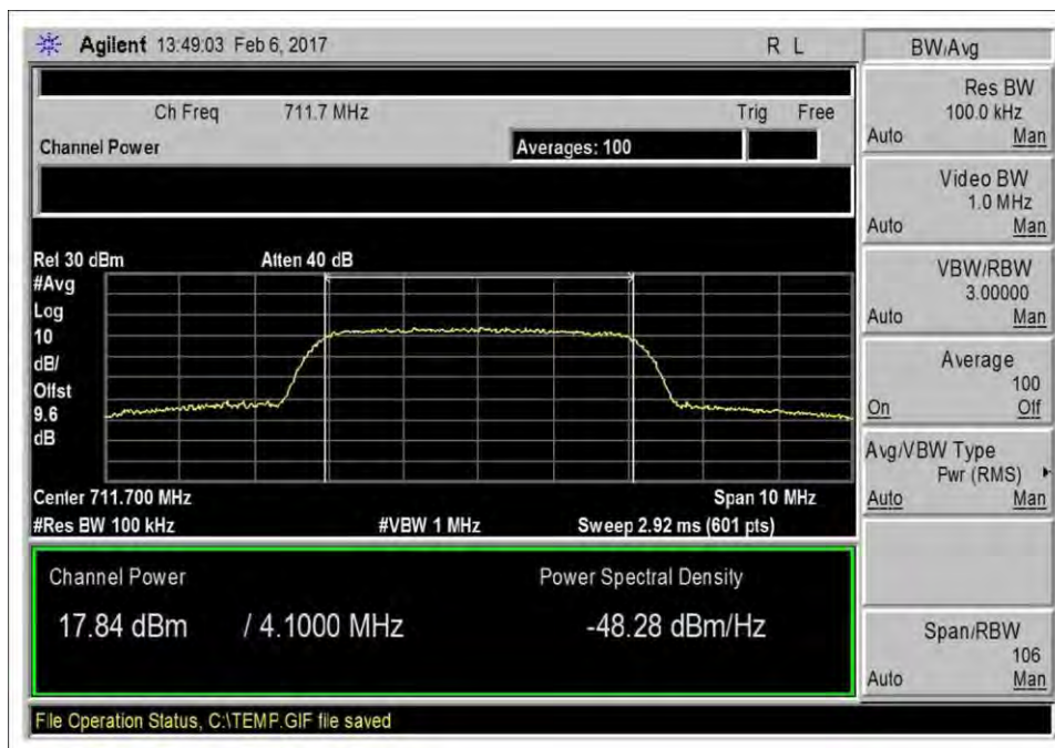
7.2_Power_UL_698-716MHz-Max
