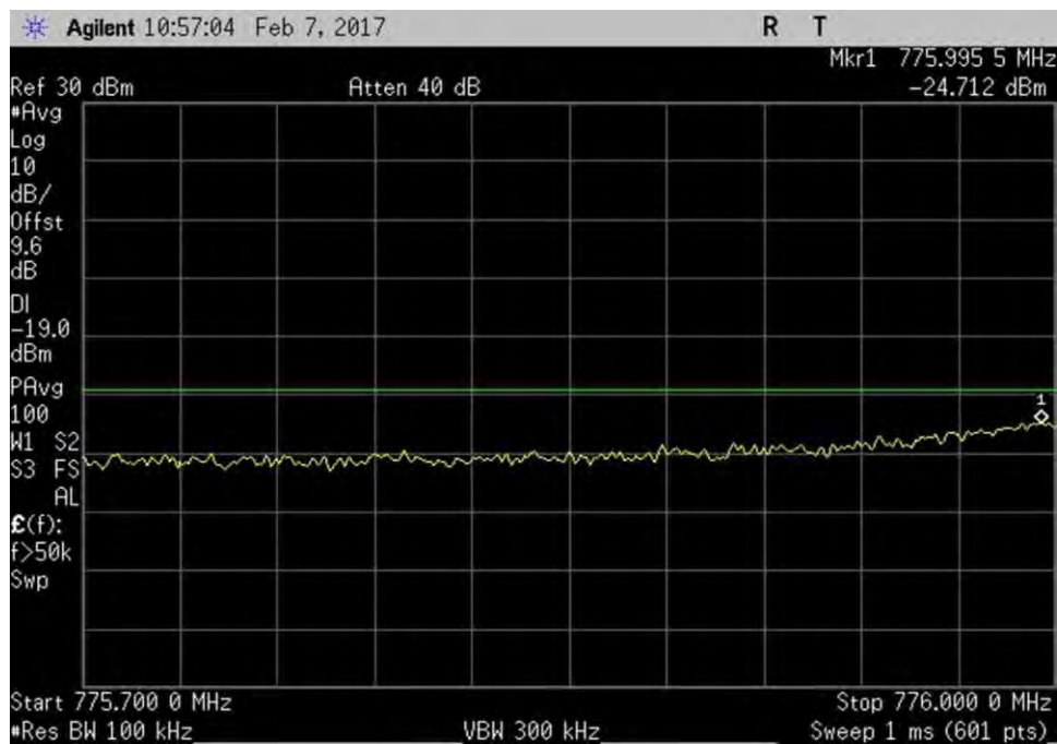
7.5_OBE_UL_776-787MHz_L_PreAGC_LTE
