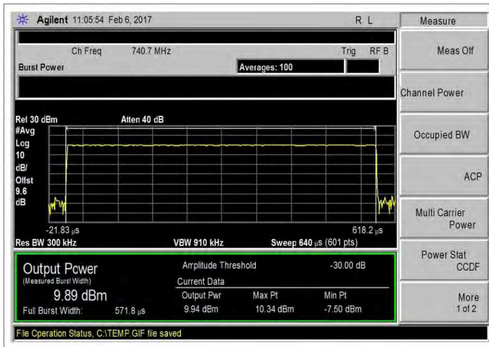
7.2_Power_DL_728-746MHz
