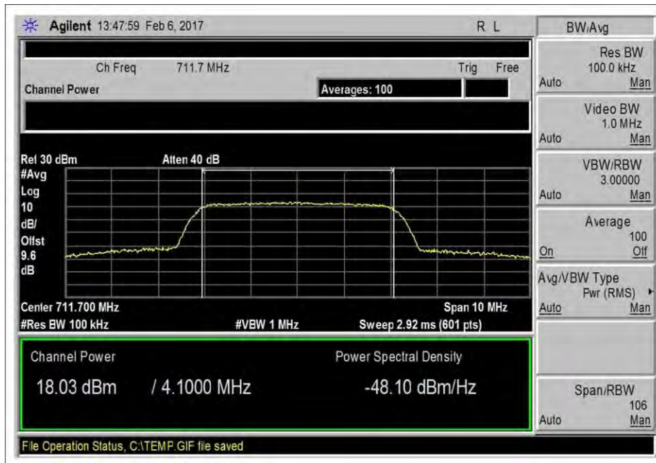
7.2_Power_UL_698-716MHz
