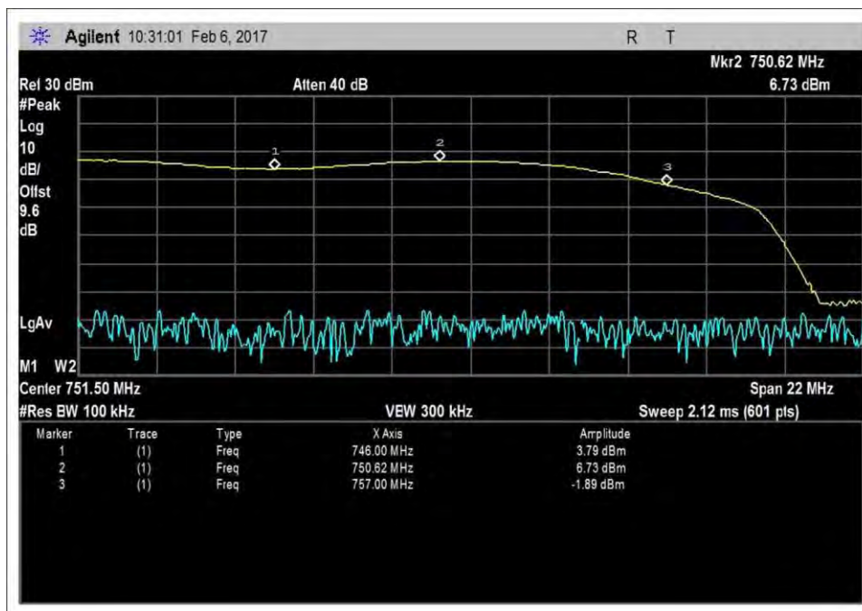
7.1_Band Verify_DL_746-757MHz
