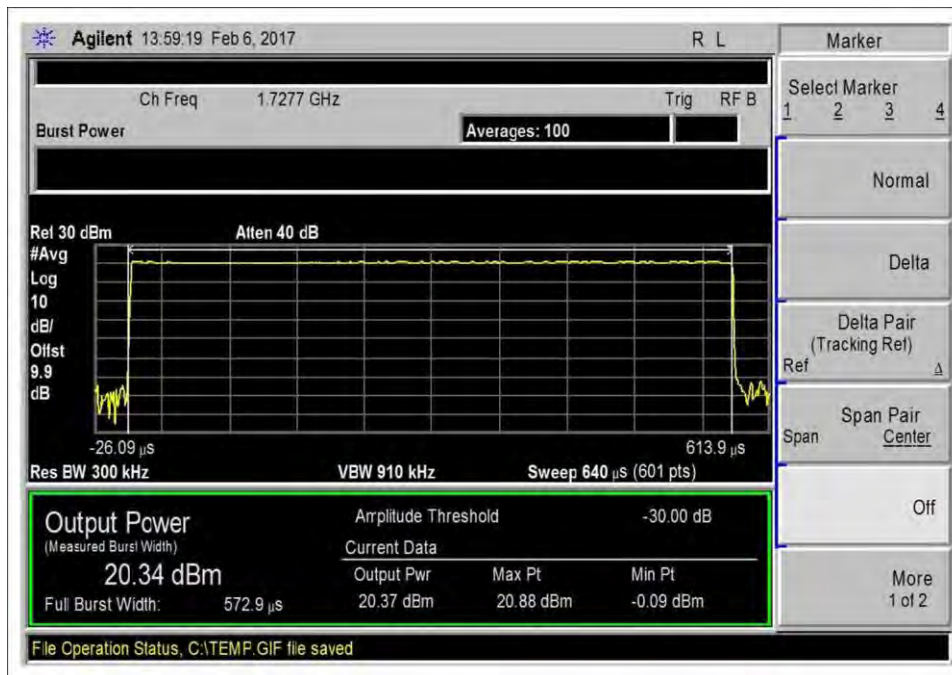
7.2_Power_UL_1710-1755MHz
