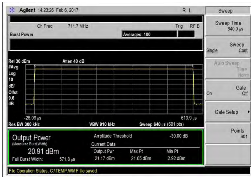
7.2_Power_UL_698-716MHz-Max
