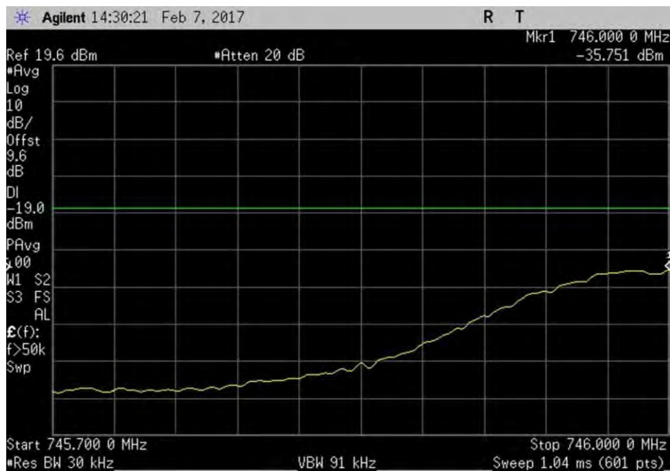
7.5_OBE_DL_746-757MHz_L_PreAGC_GSM
