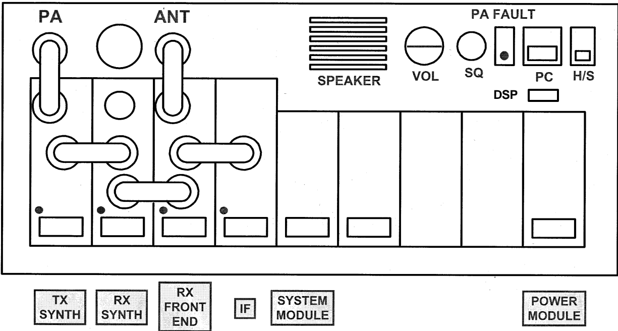
Figure 3-2: Module Configuration
