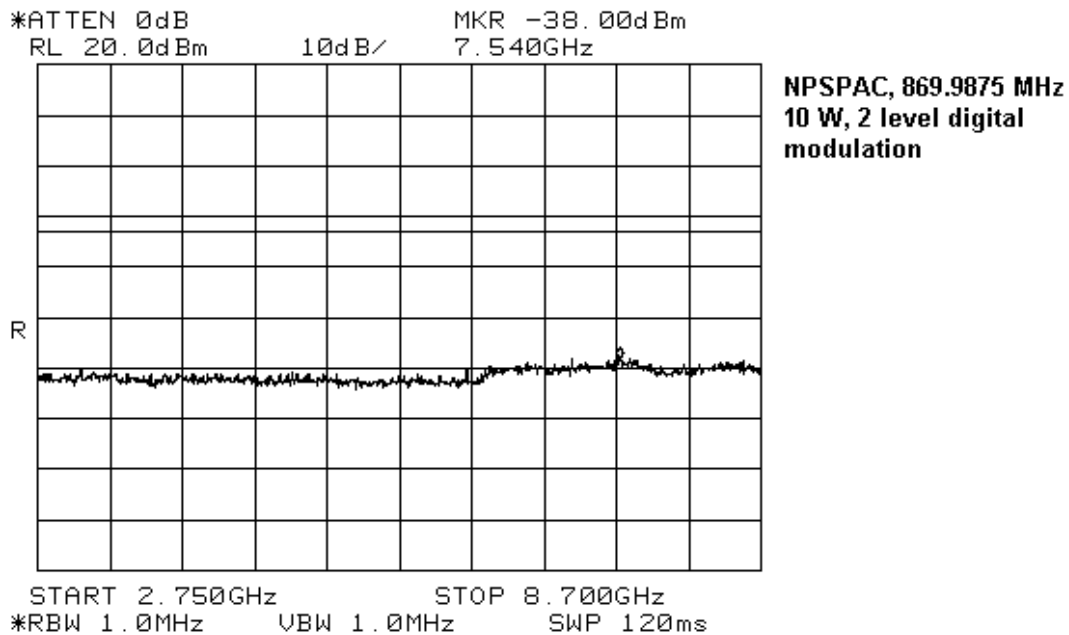
Figure 7-13: Tx at 869.9875 MHz, 10 W Power, 2.75 GHz to 8.7 GHz
