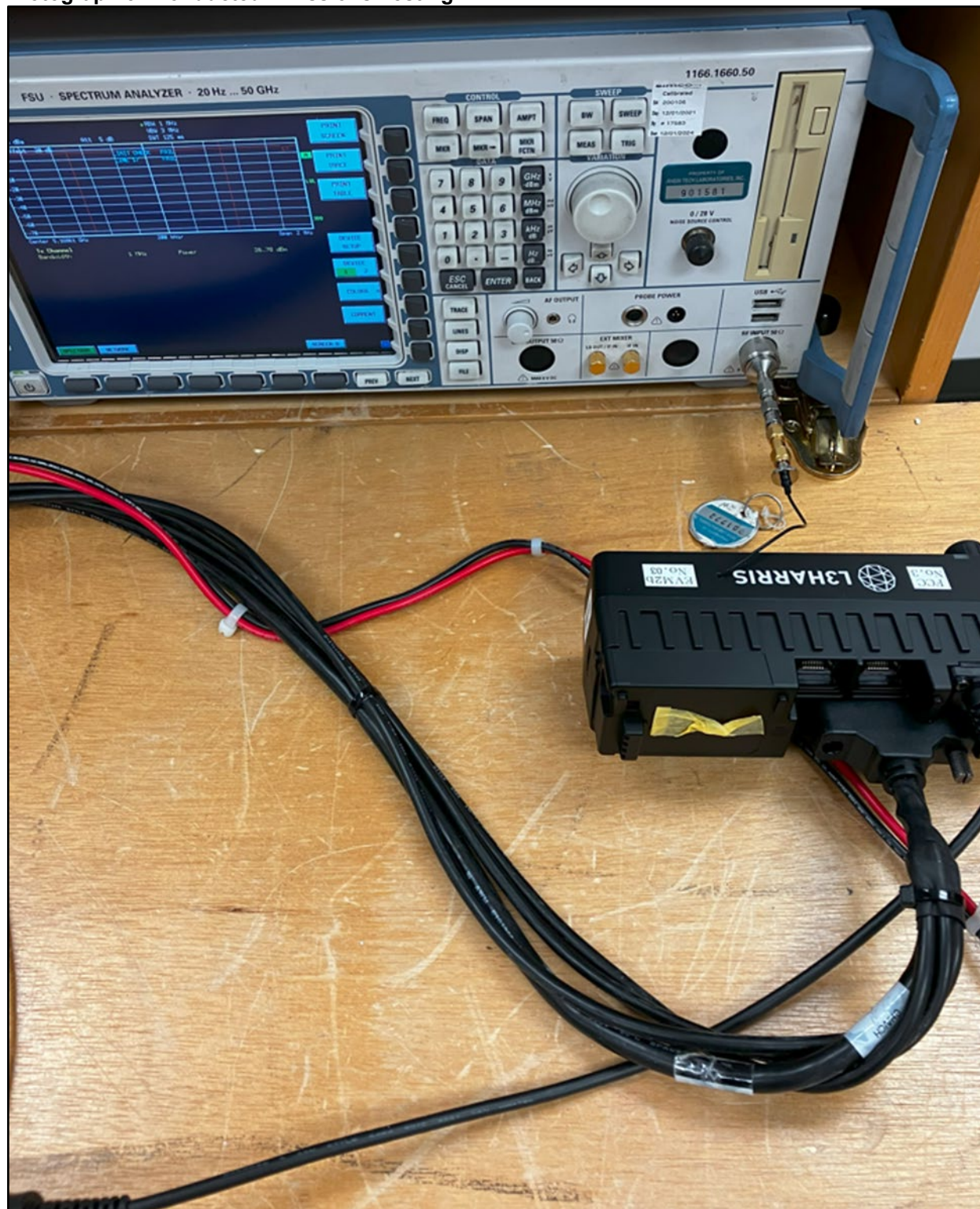
Photograph 5: Conducted Emissions Testing
