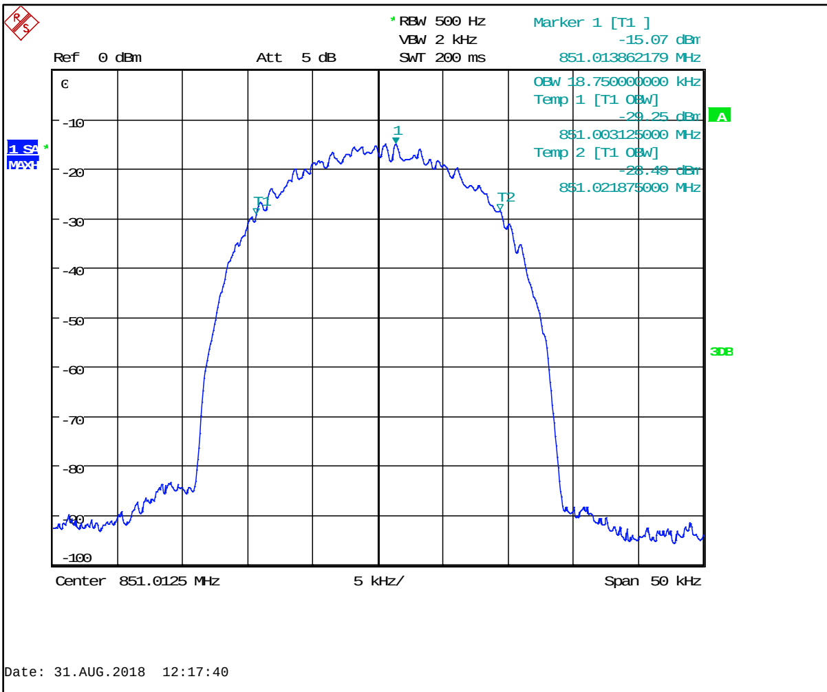
Plot 5-4: Occupied Bandwidth – 851.0125 MHz; HVD SMR; 99% BW
