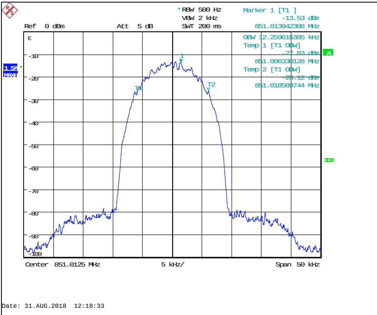
Plot 5-5: Occupied Bandwidth – 851.0125 MHz; HVD NPSPAC; 99% BW
