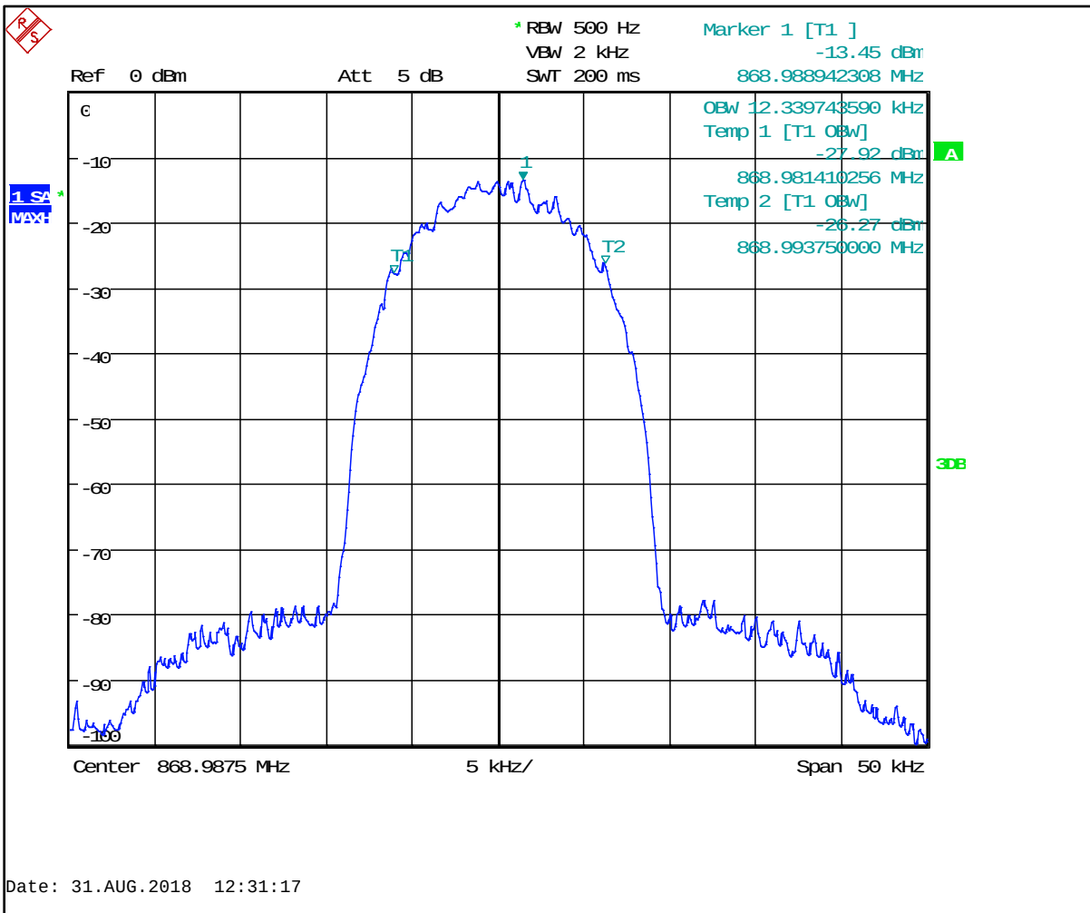
Plot 5-7: Occupied Bandwidth – 868.9875 MHz; HVD NPSPAC; 99% BW
