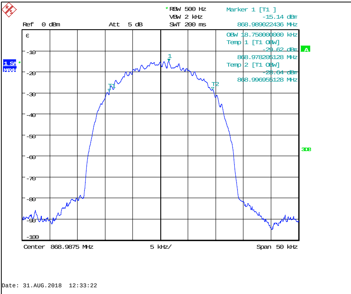
Plot 5-6: Occupied Bandwidth – 868.9875 MHz; HVD SMR 99% BW
