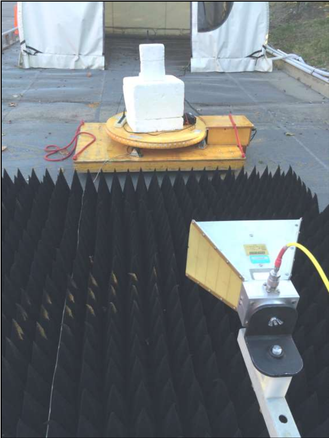
Photograph 6: Radiated Emissions – Back View
