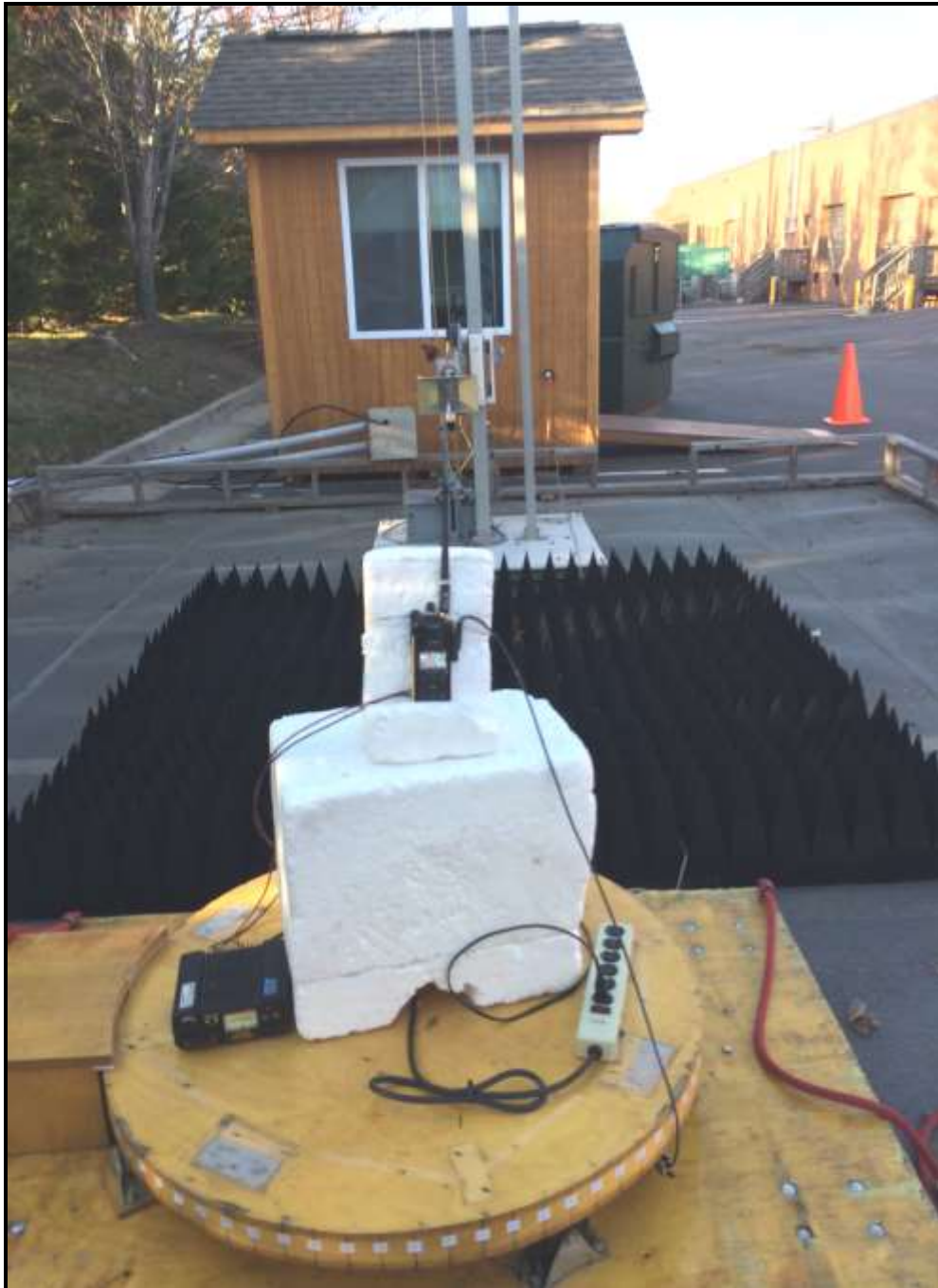
Photograph 5: Radiated Emissions – Front View
