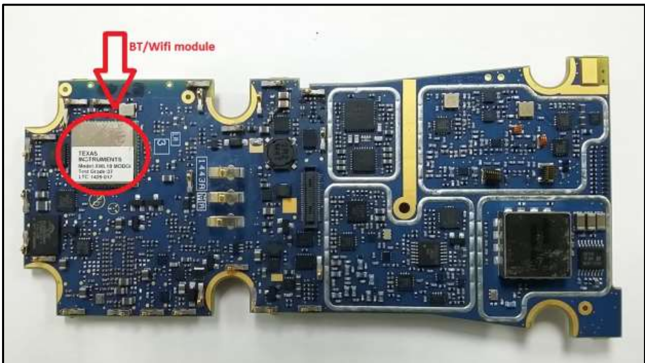
Photograph 4: Bottom View without Shields
