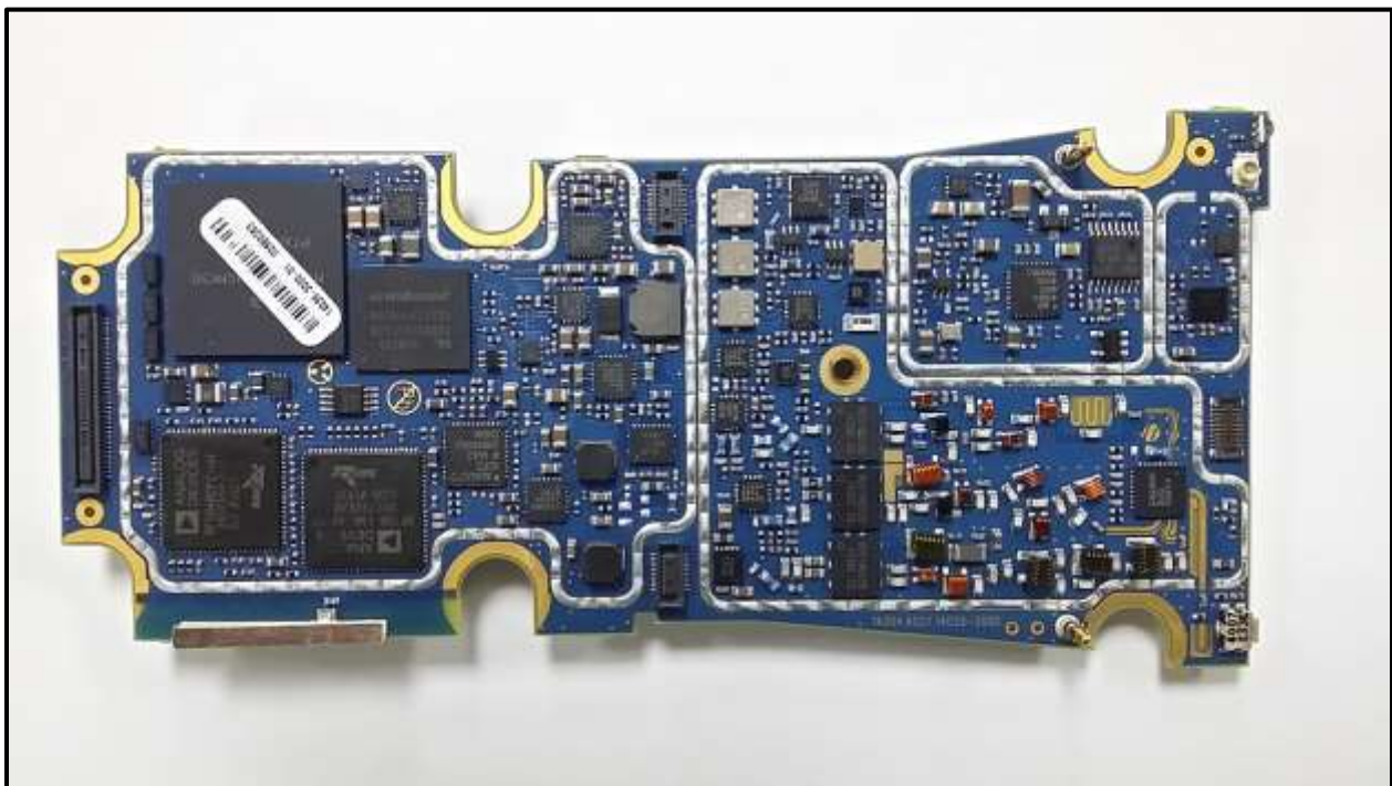
Photograph 2: Top View without Shields
