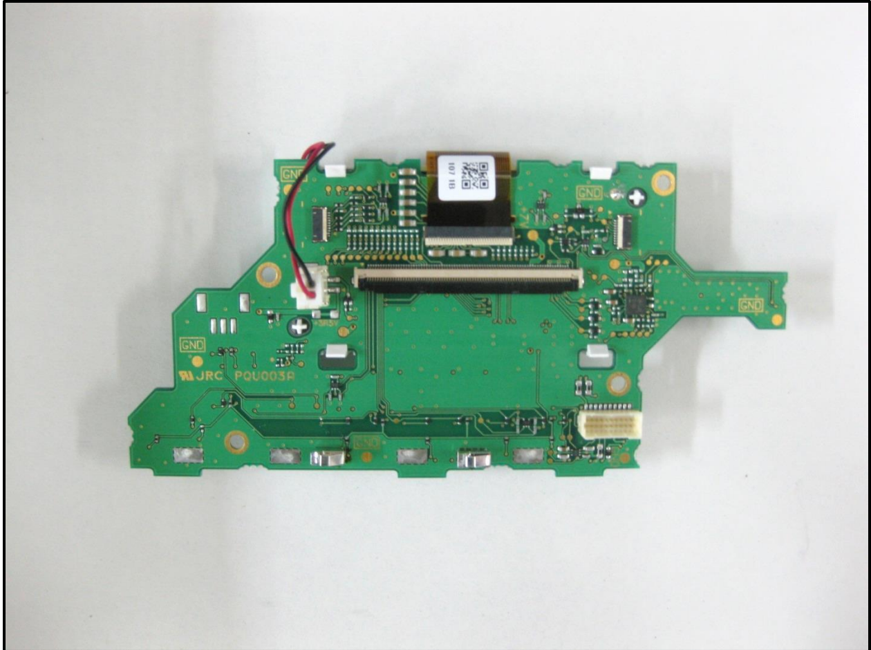
Photograph 23: Solder Side
