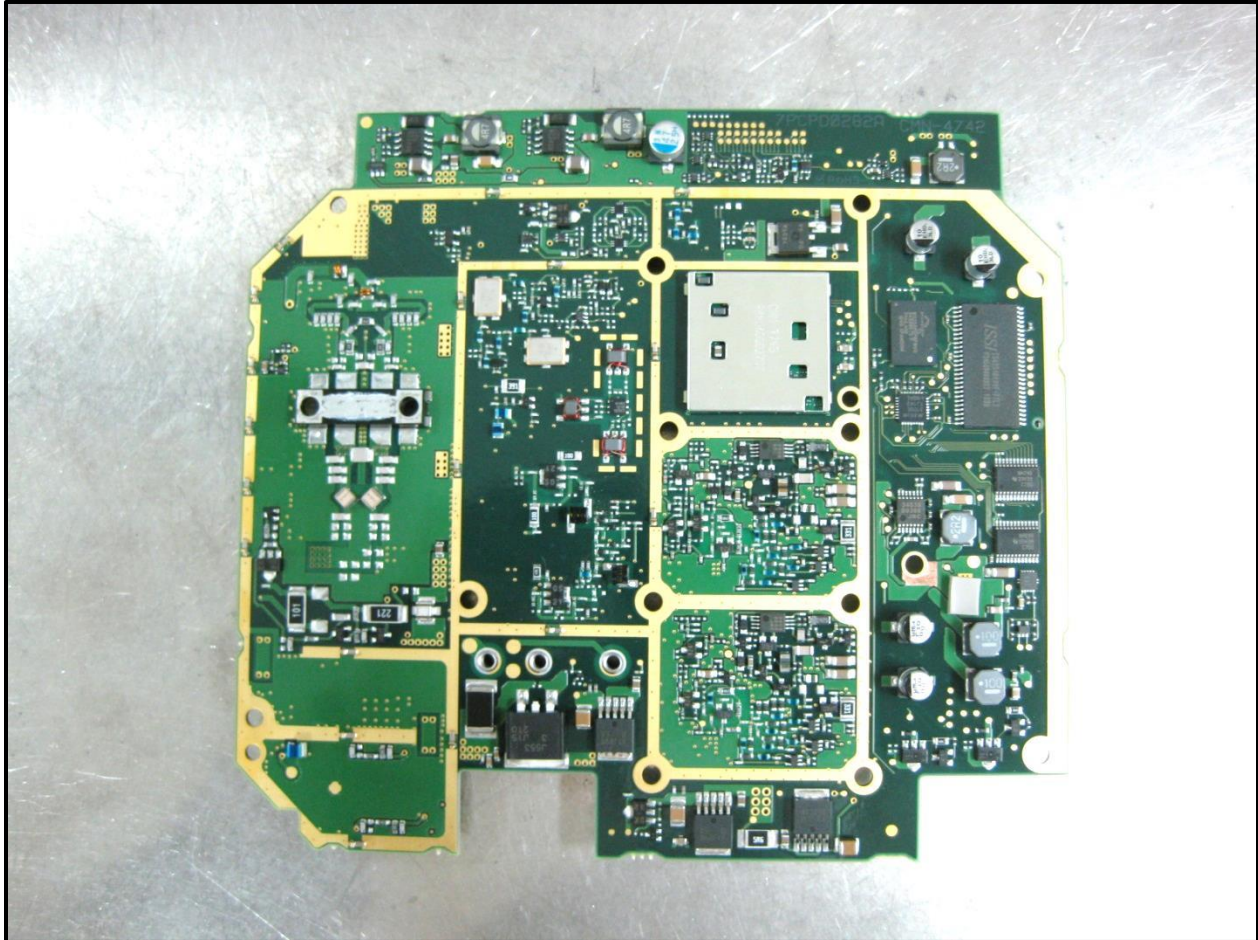
Photograph 16: Solder Side
