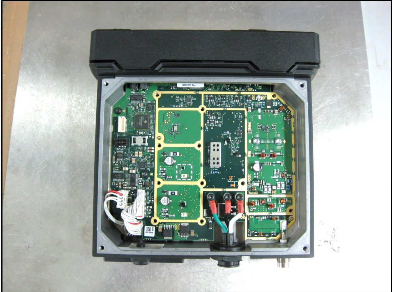
Photograph 14: Bottom Cover and Shield Removed
