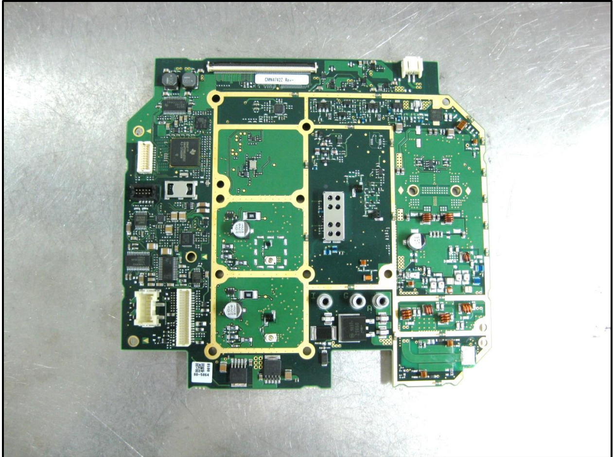
Photograph 15: PCB Side
