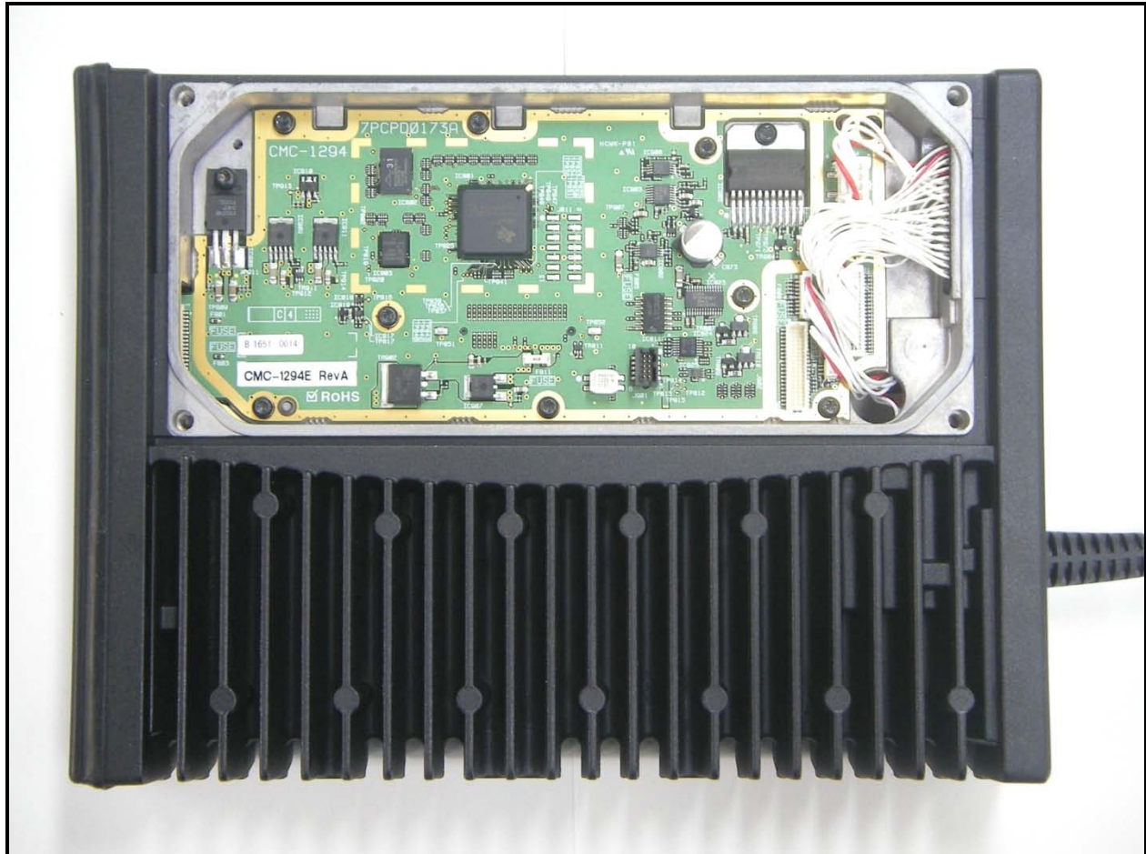
Photograph 13: HB – Top Cover Removed
