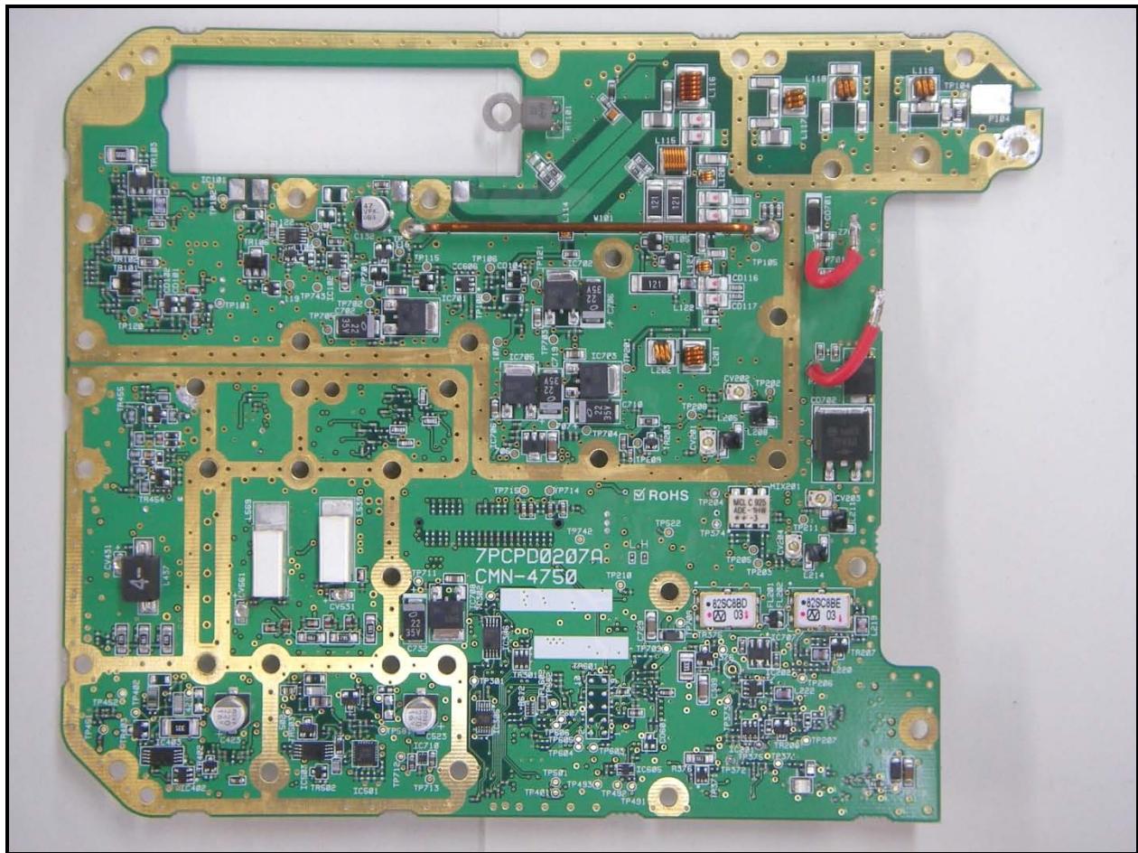
Photograph 16: HB RF Processor Board Component Side
