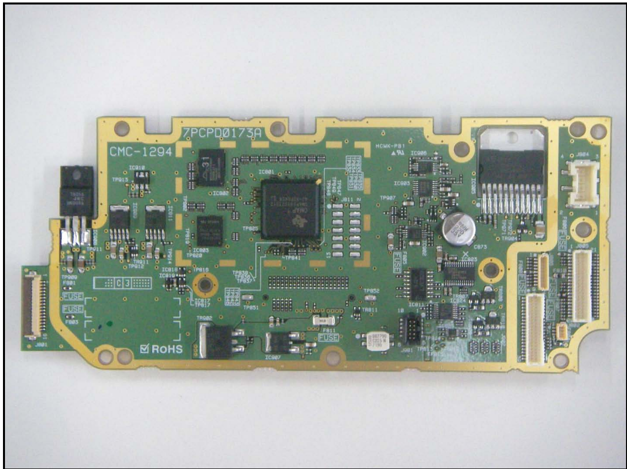
Photograph 18: HB PK Board Component Side
