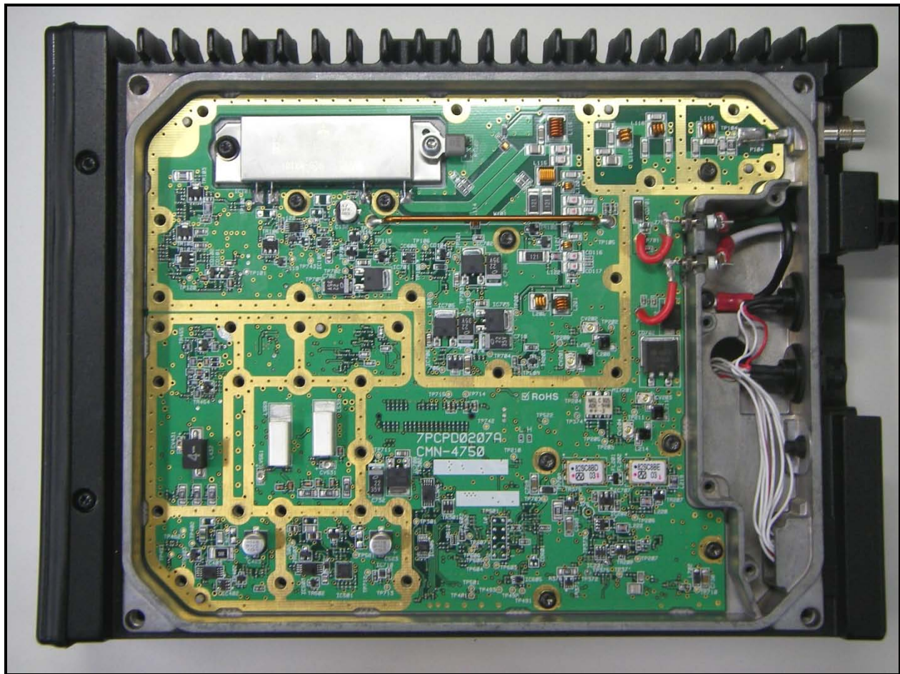
Photograph 15: HB Bottom Cover and Shield Removed
