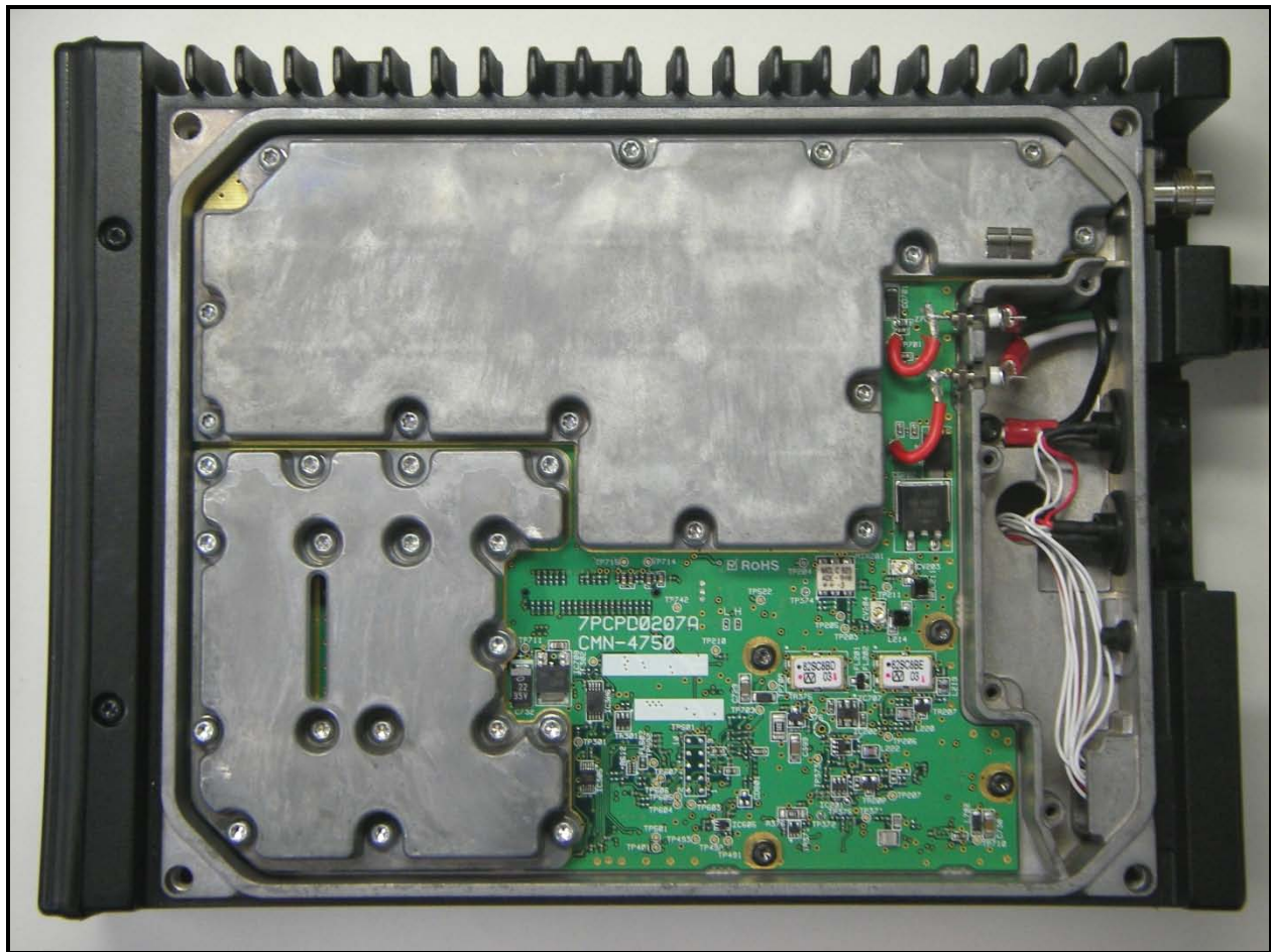
Photograph 14: HB Bottom Cover Removed
