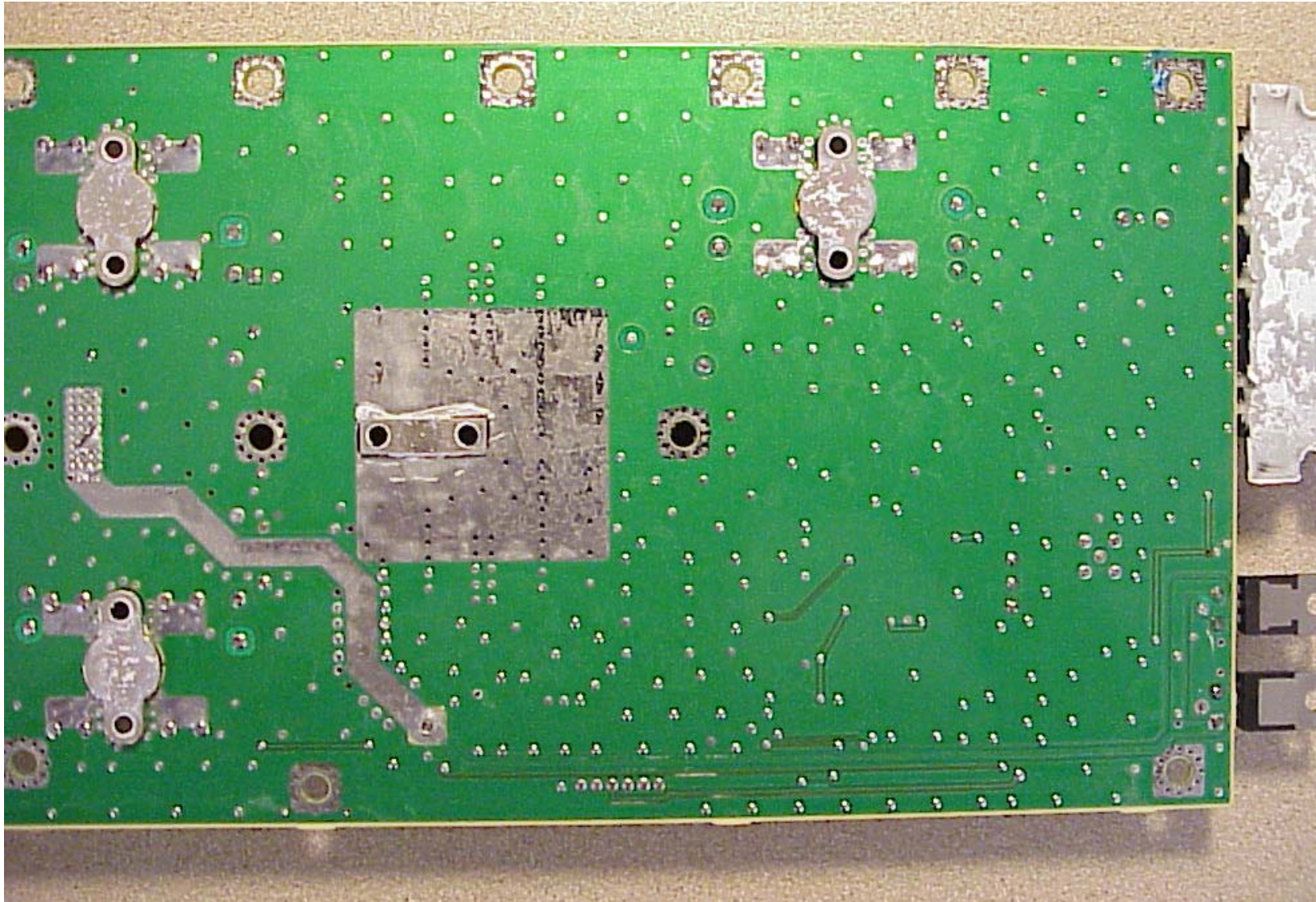
Figure 23 - PA board bottom - input end
