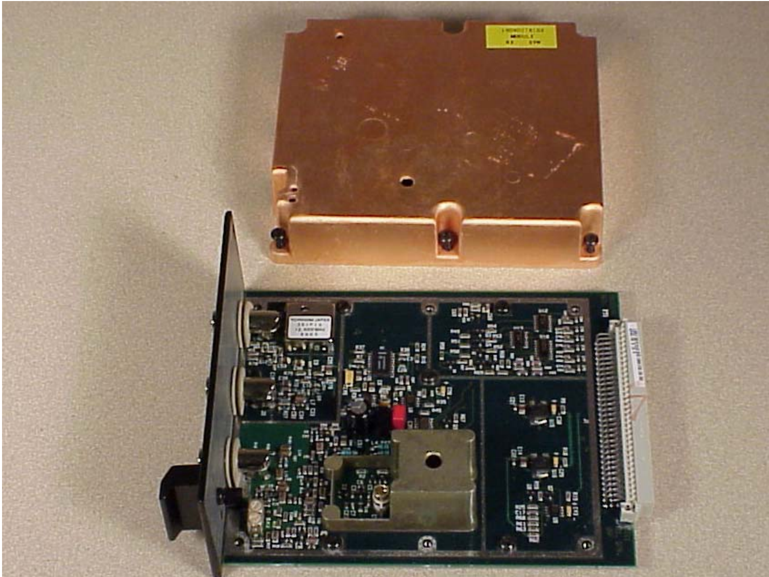
Figure 29 - Rx Synthesizer cover removed
