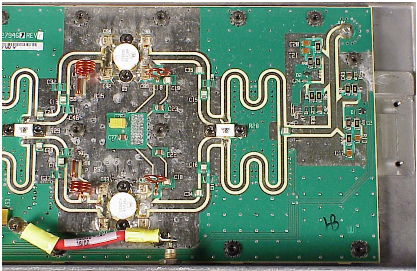
Figure 21 - PA board top, output end
