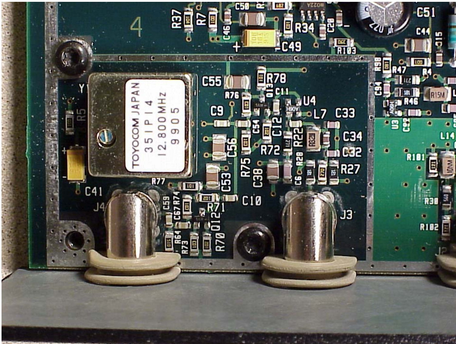
Figure 32 - Rx Synthesizer frequency reference
