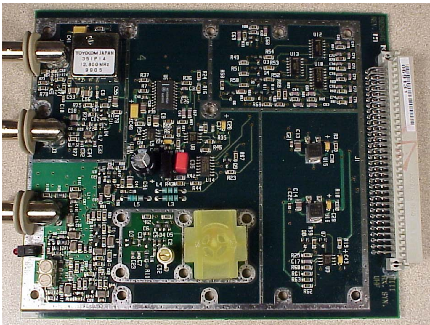
Figure 30 - Rx Synthesizer board top
