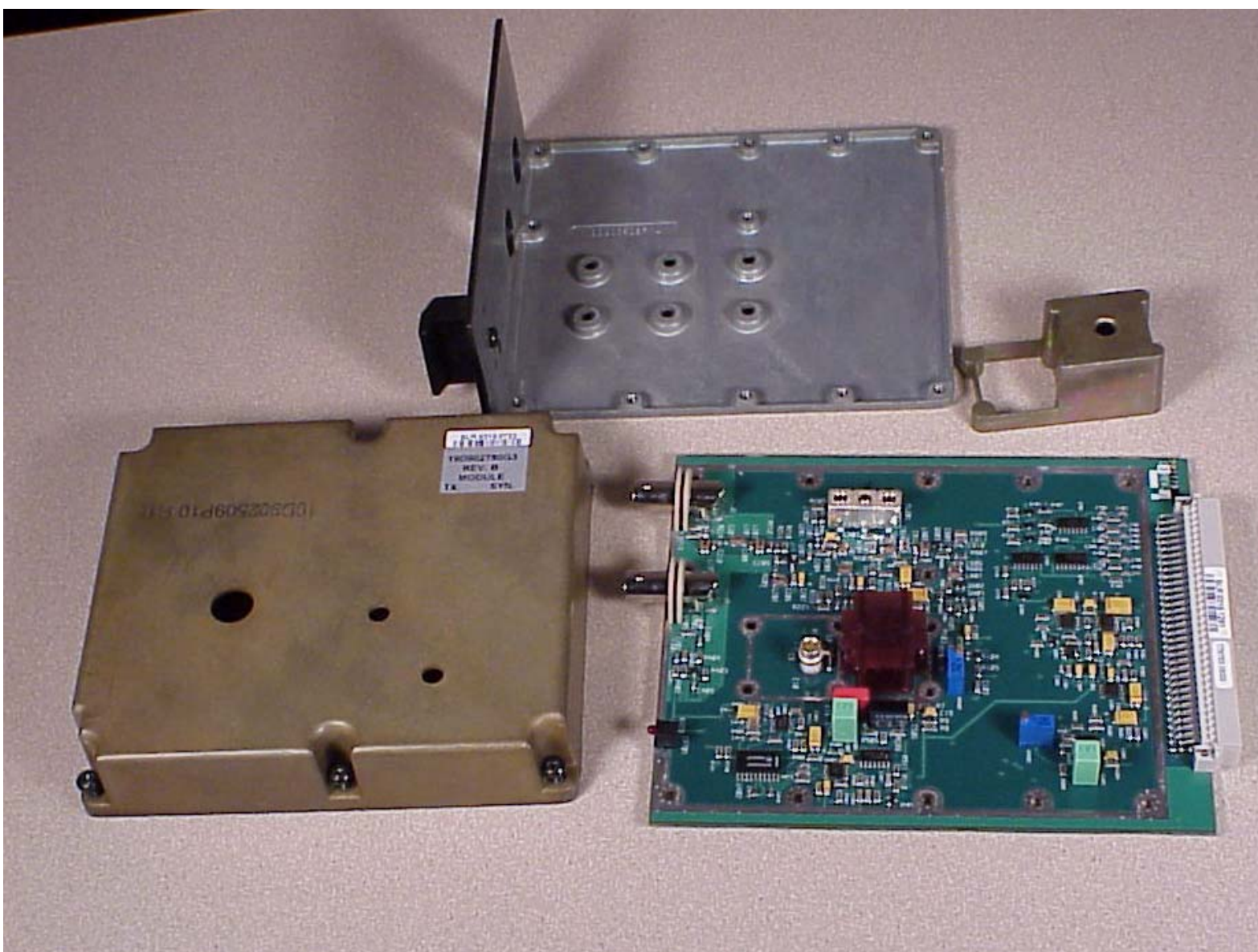
Figure 17 - Tx Synthesizer disassembled
