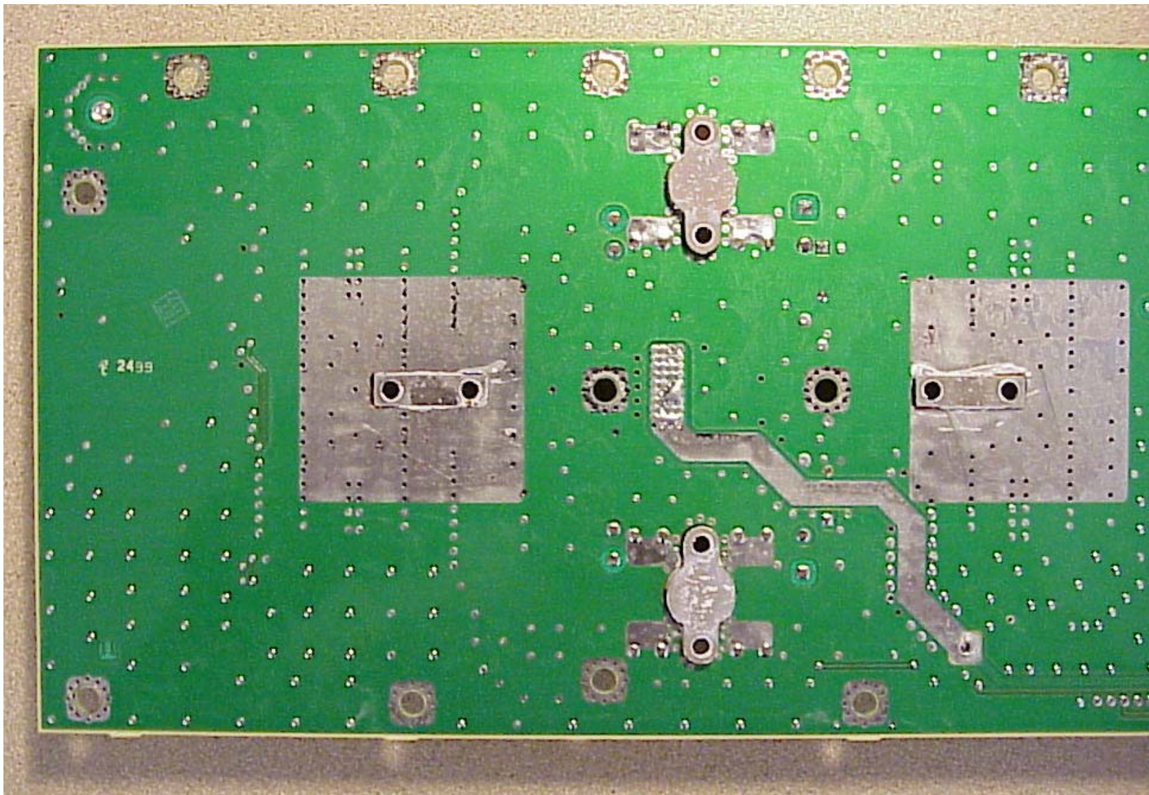
Figure 24 - PA board bottom - output end
