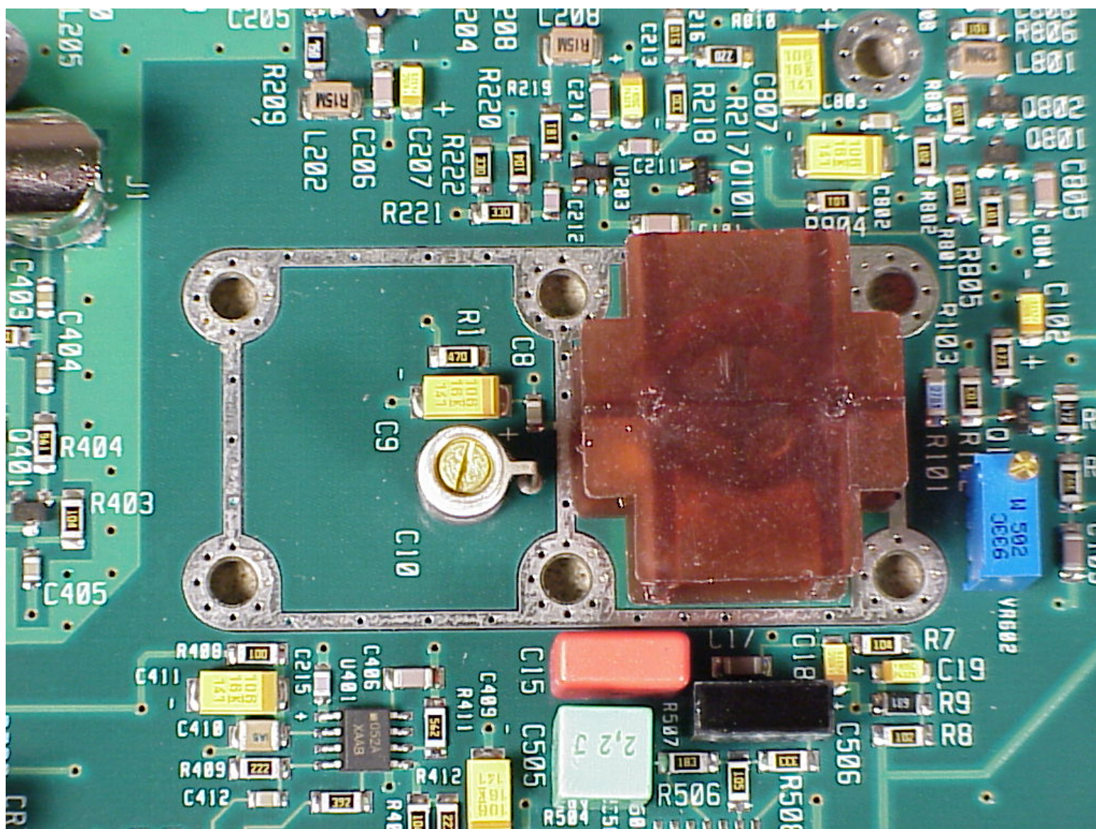
Figure 15 - Tx Synthesizer VCO top
