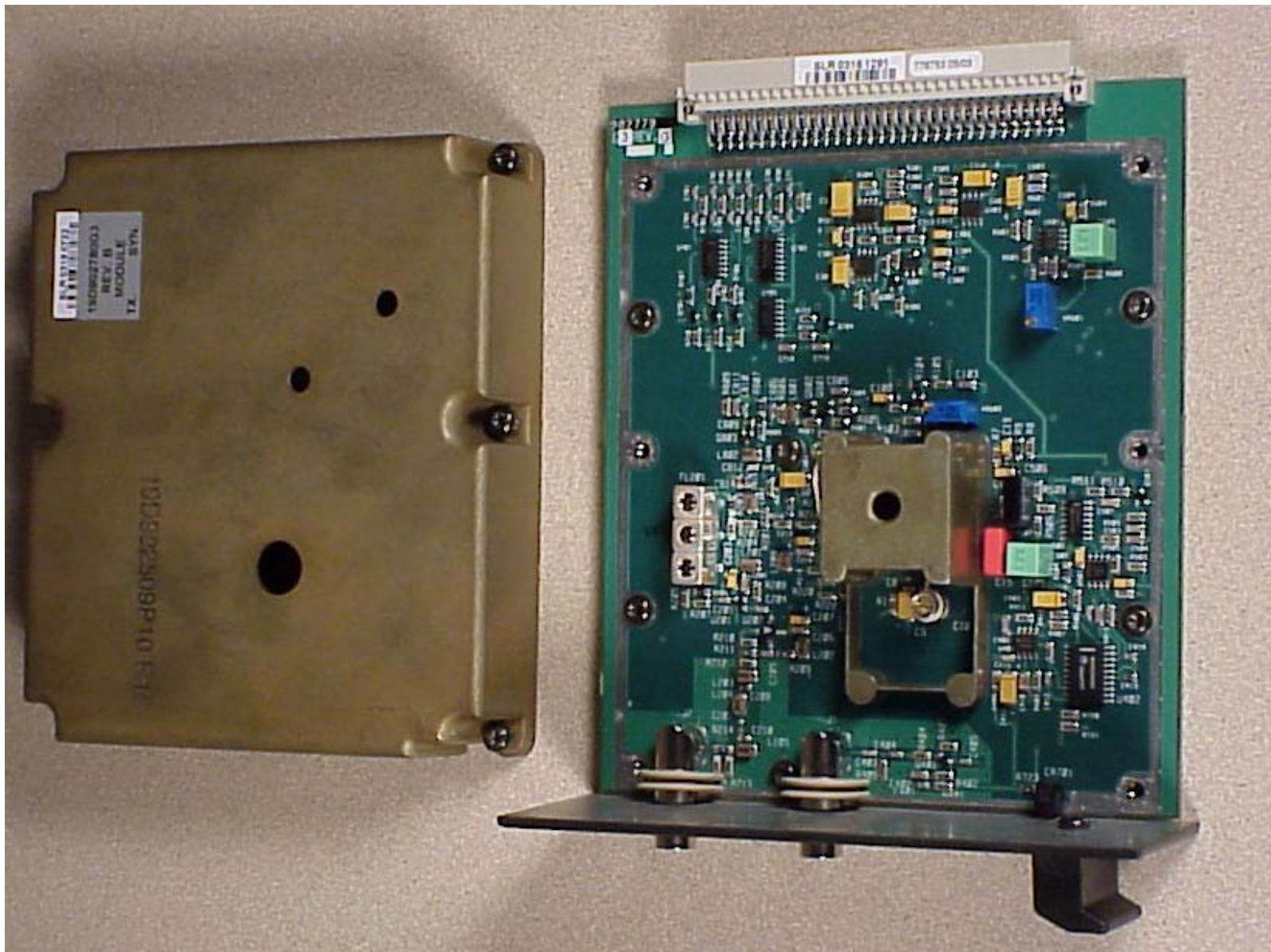
Figure 12 - Tx Synthesizer - cover removed
