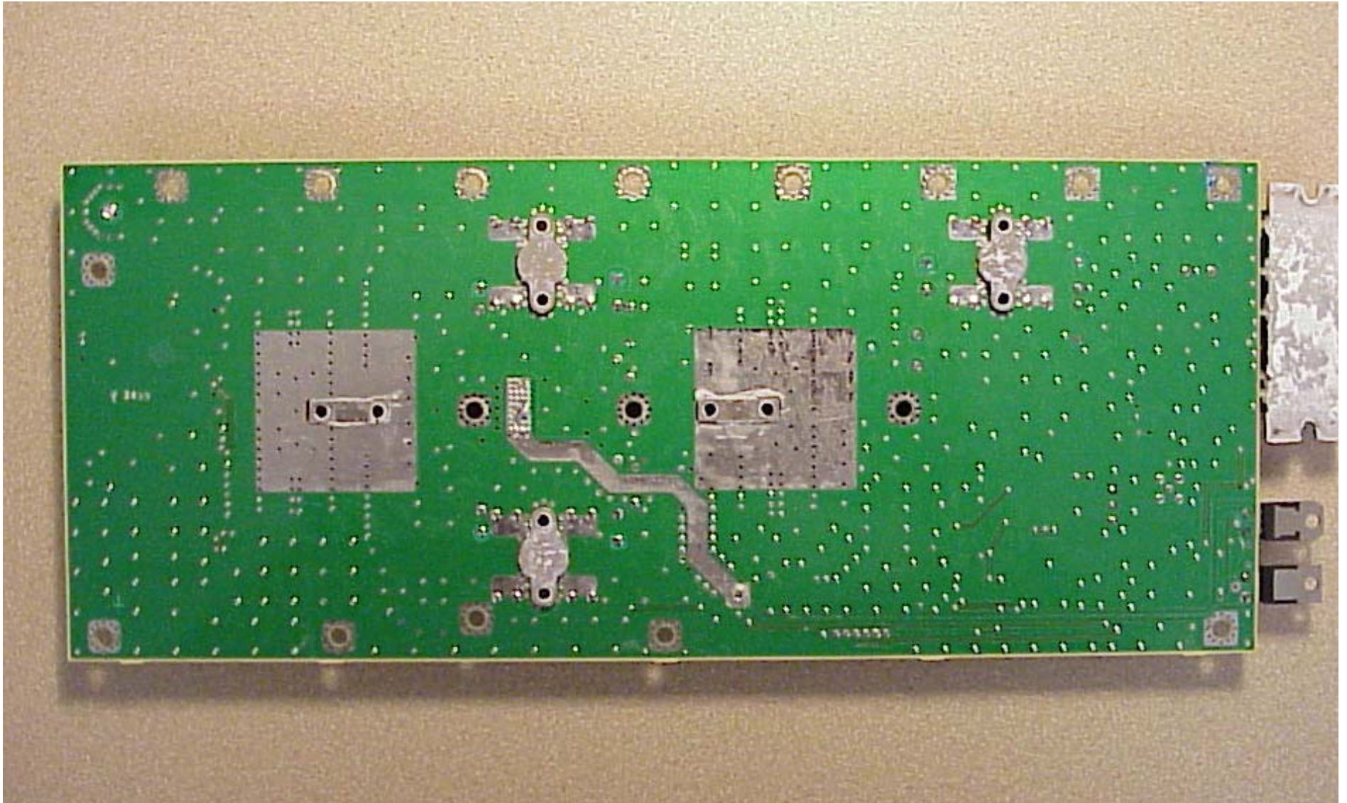
Figure 22 - PA board bottom
