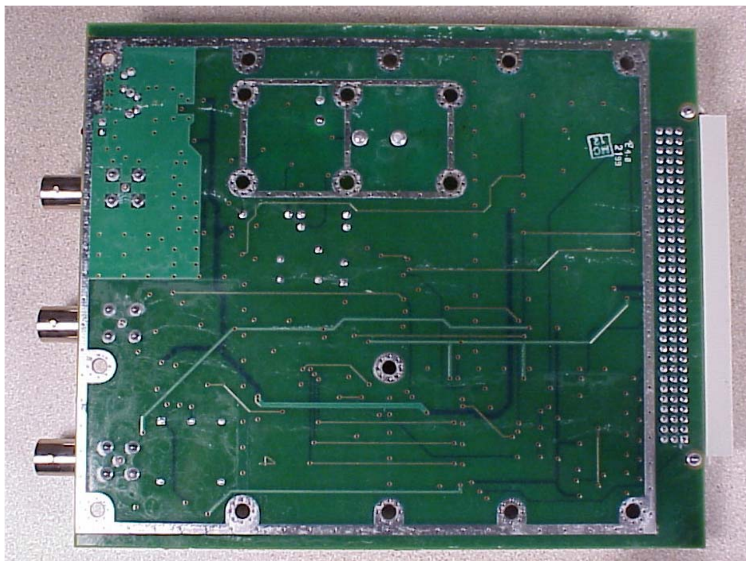
Figure 31 - Rx Synthesizer board bottom
