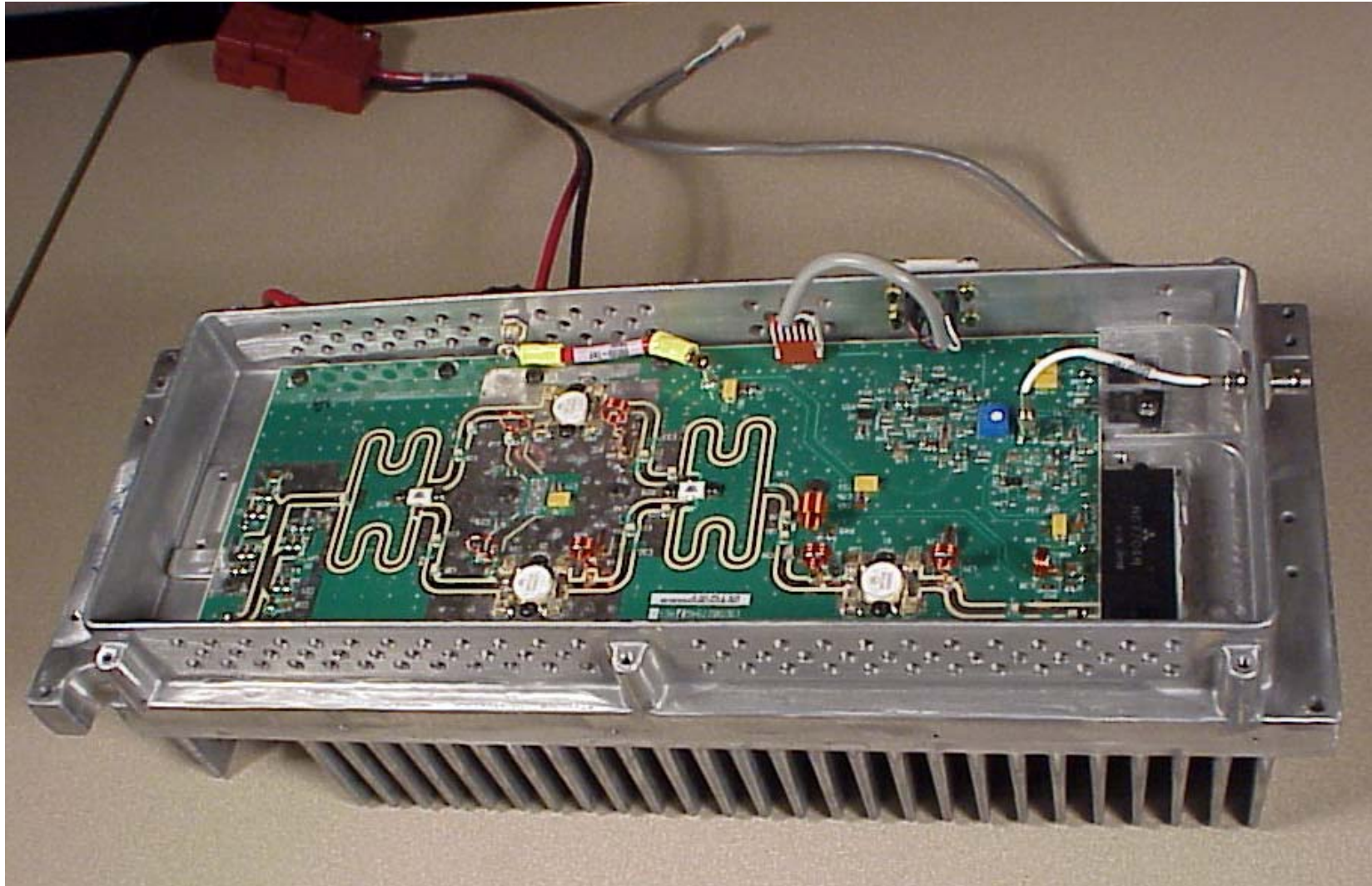
Figure 19 - PA with cover removed
