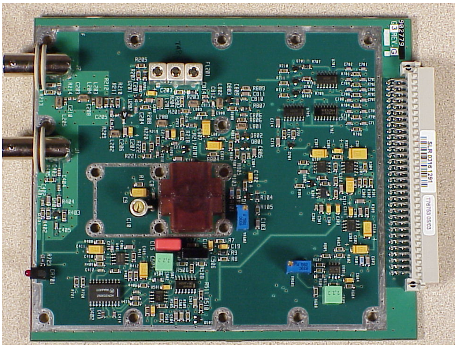
Figure 13 - Tx Synthesizer board top
