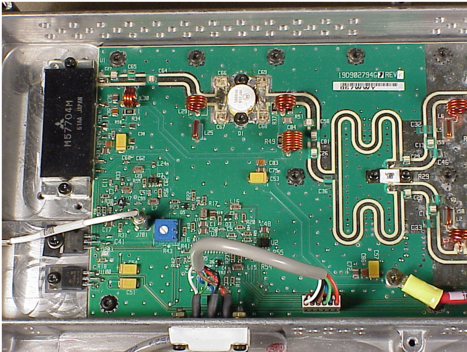
Figure 20 - PA board top, input end
