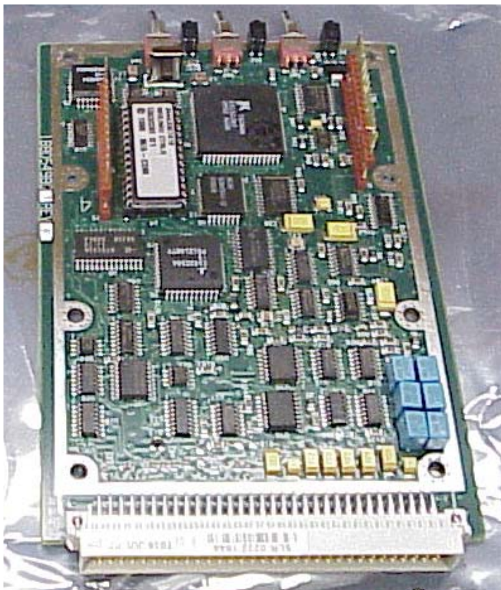
Figure 7 - System Module, main board top
