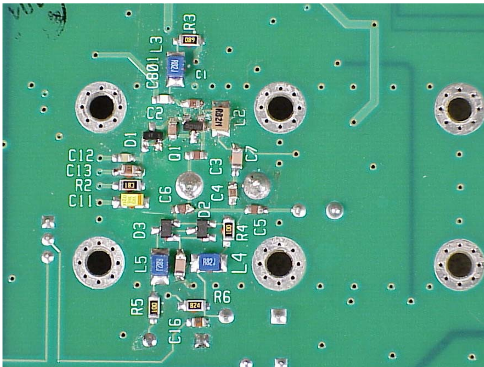
Figure 16 - Tx Synthesizer VCO bottom
