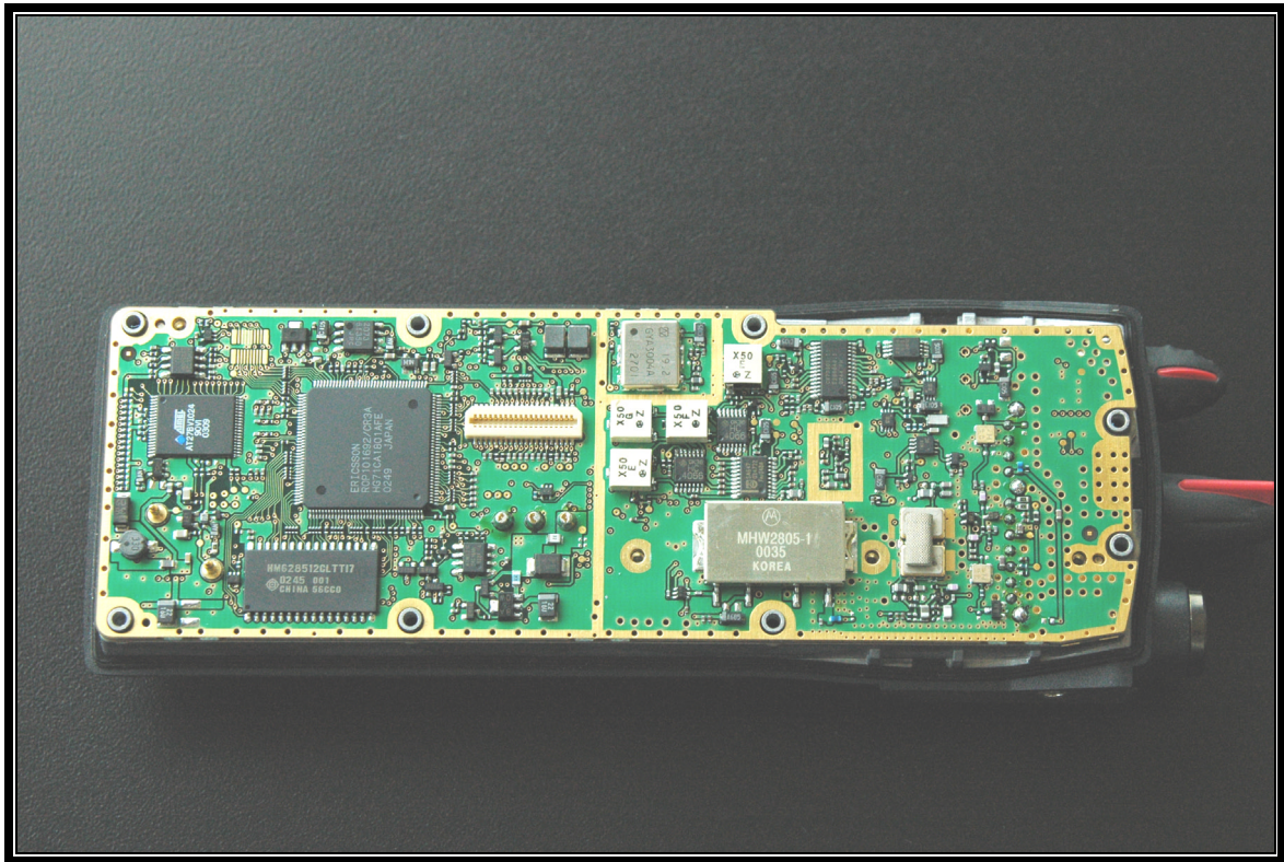
PHOTOGRAPH 9: VIEW OF TOP OF MAIN BOARD WITH RF SHIELD REMOVED
