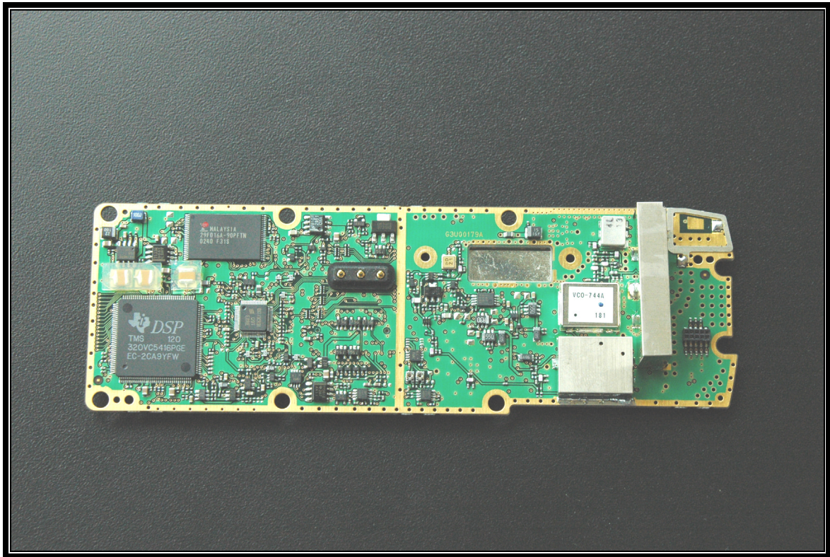
PHOTOGRAPH 10: VIEW OF BOTTOM OF MAIN BOARD
