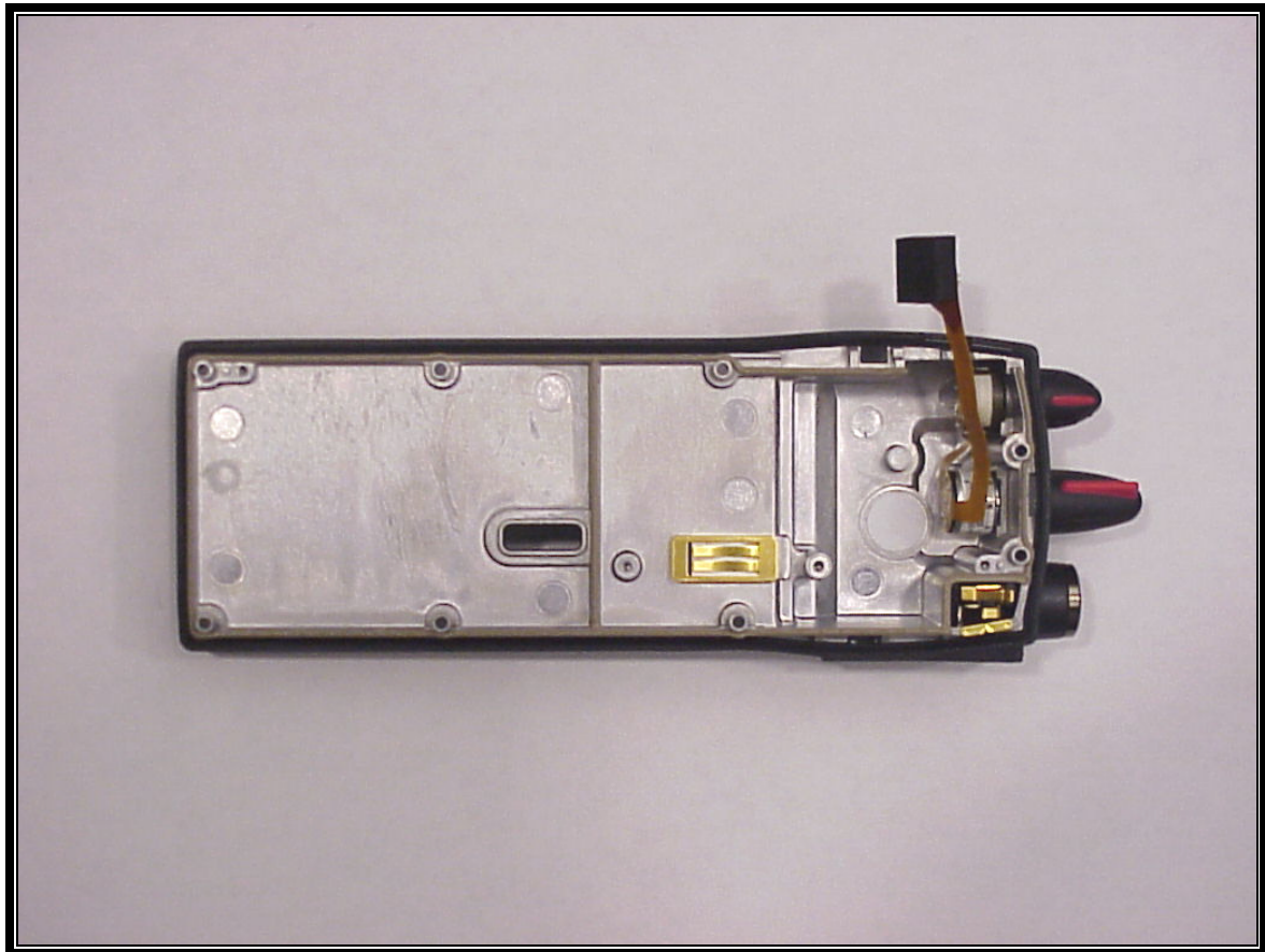
PHOTOGRAPH 11: VIEW OF INSIDE WALL OF REAR CASTING WITH MAIN BOARD REMOVED
