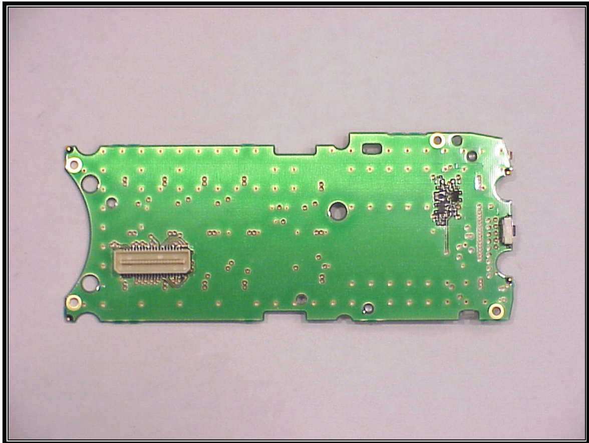
PHOTOGRAPH 7: VIEW OF BOTTOM OF INTERFACE BOARD
