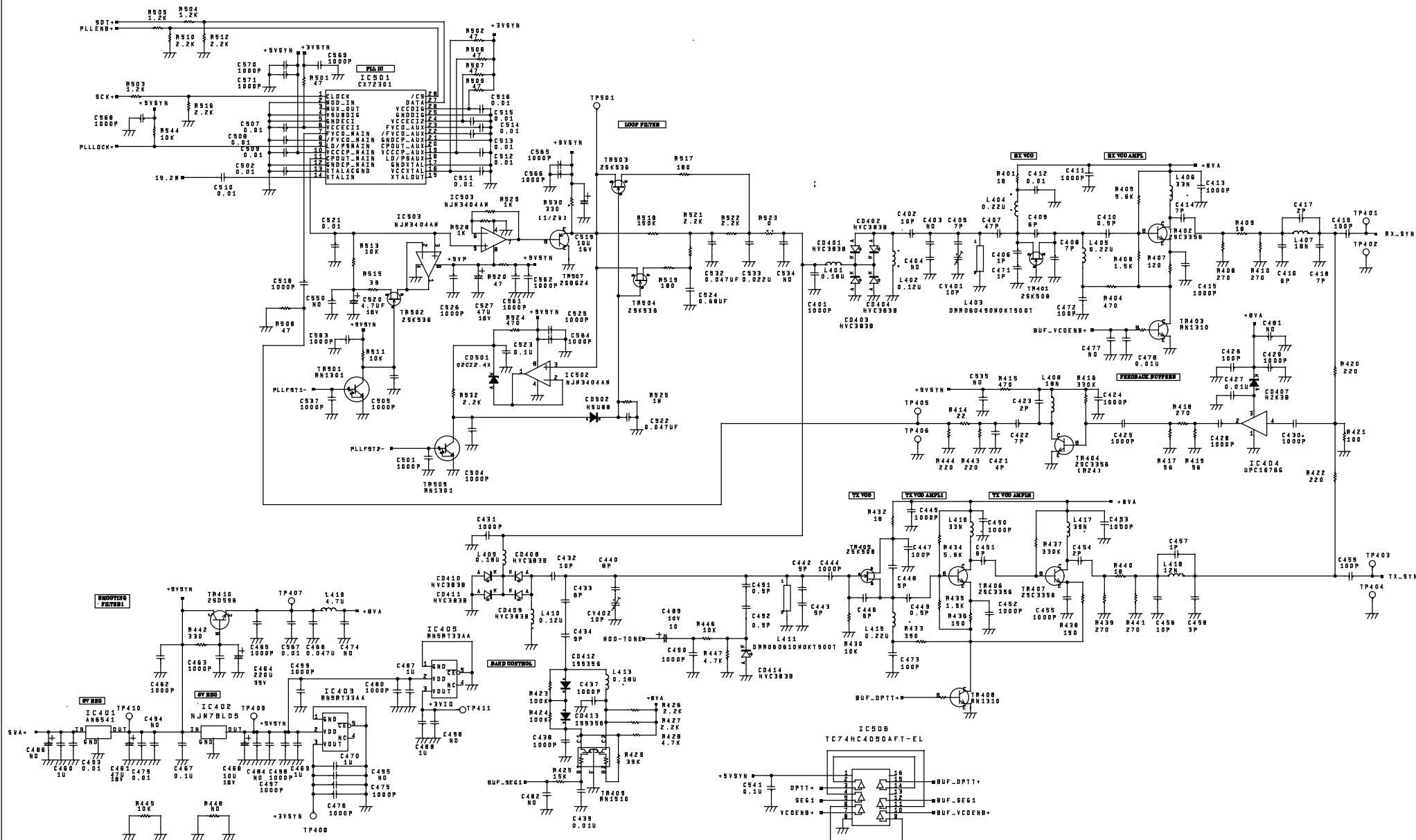
Schematic of JAGUAR 700M(800MHz)RF/SYNTH Unit
